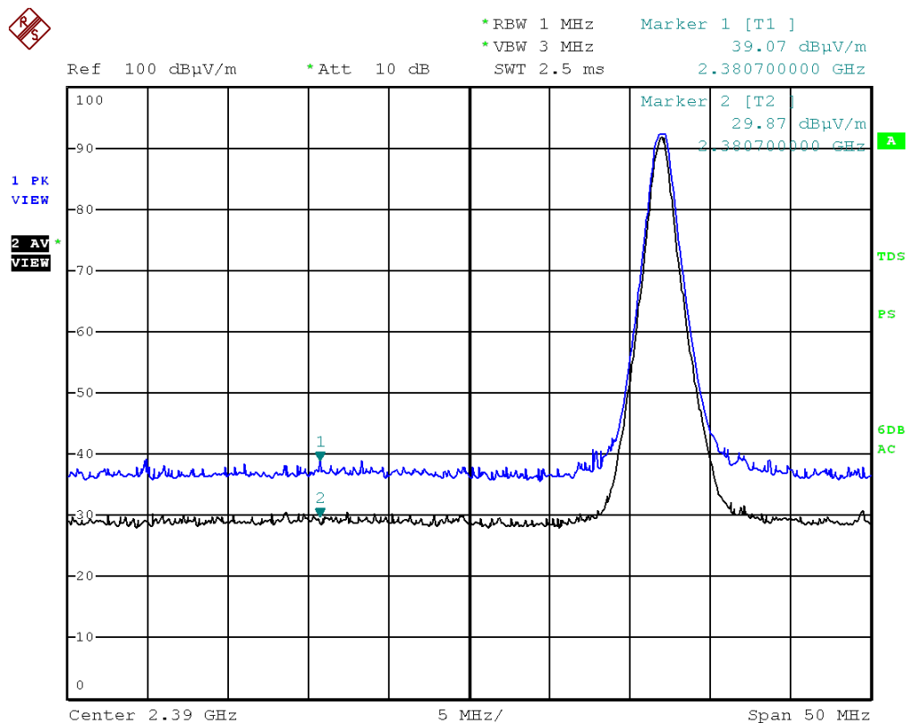
BDR(DH5) Low(Vertical)
