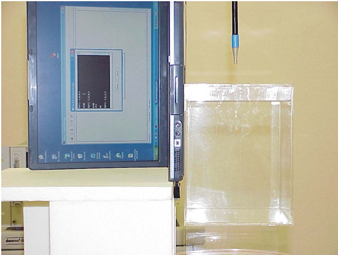
Photo 14. Lap position antenna parallel to phantom
