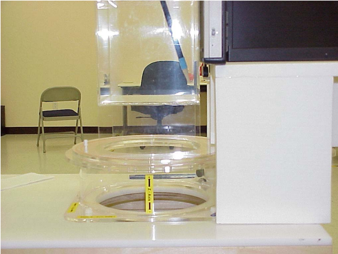
Photo 5. Lap position antenna away from phantom
