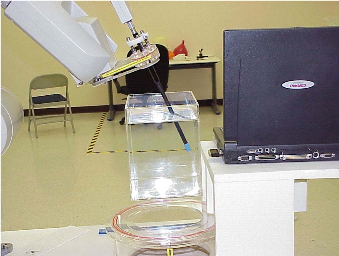
Photo 4. Antenna Horizontal 2.5cm Bystander
