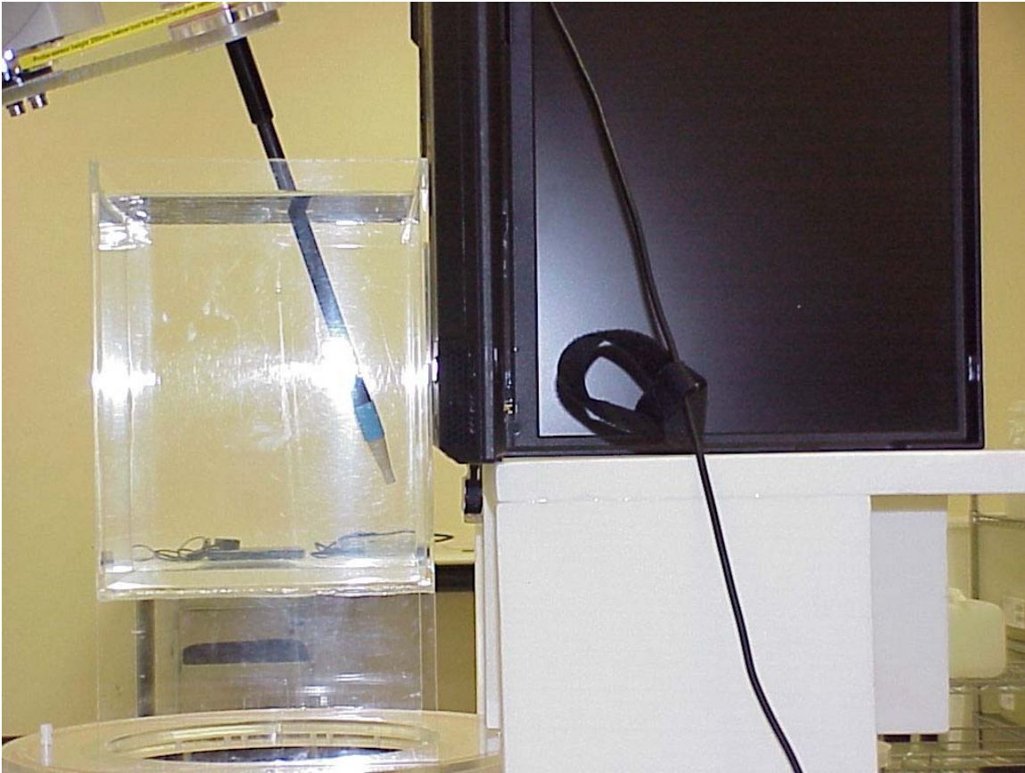
Photo 9. Lap position antenna away from phantom
