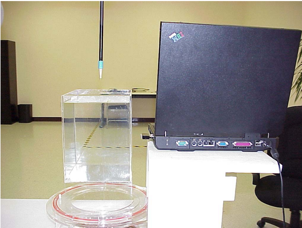
Photo 8. Antenna Horizontal 2.5cm Bystander
