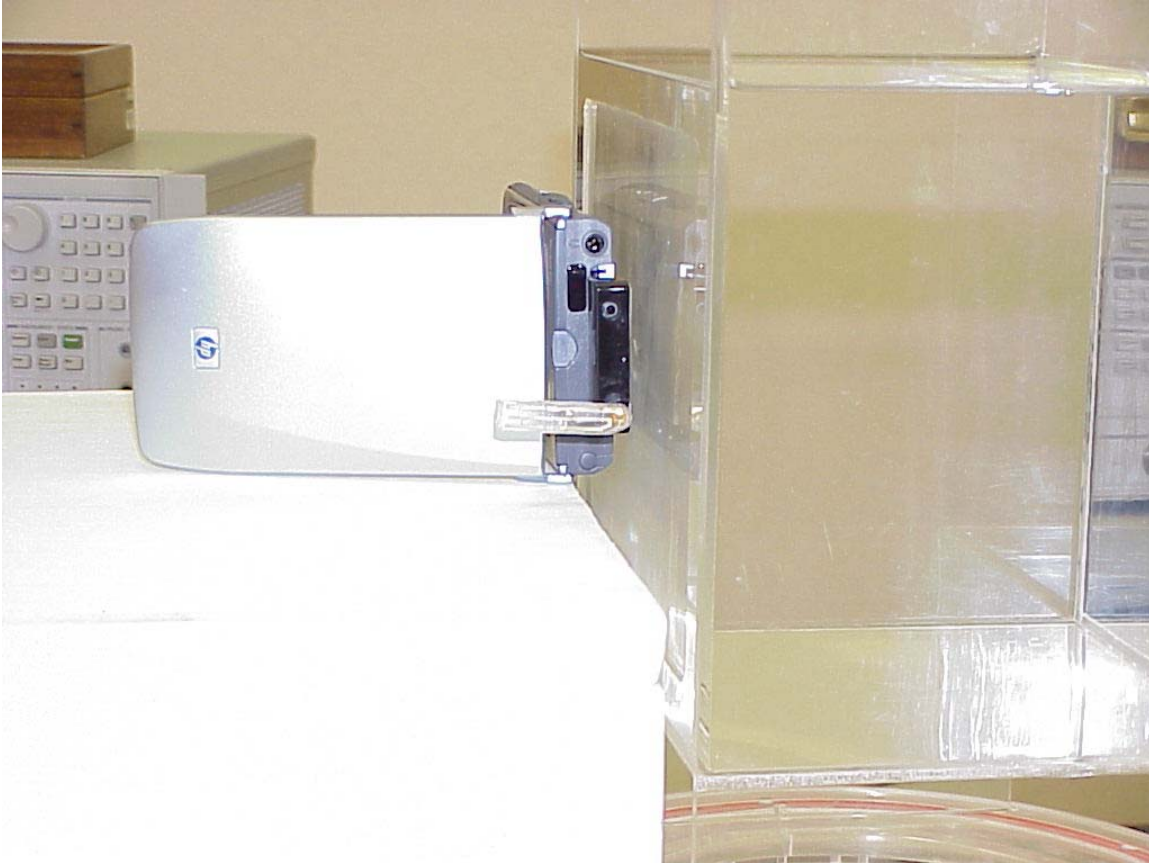
Photo 2. Lap position antenna away from phantom
