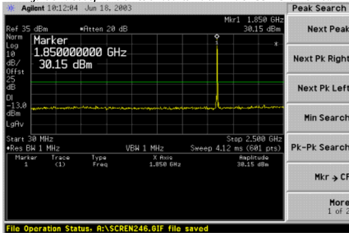
Figure 8-2: Out of Band emission at antenna terminals–GSM Channel Low
