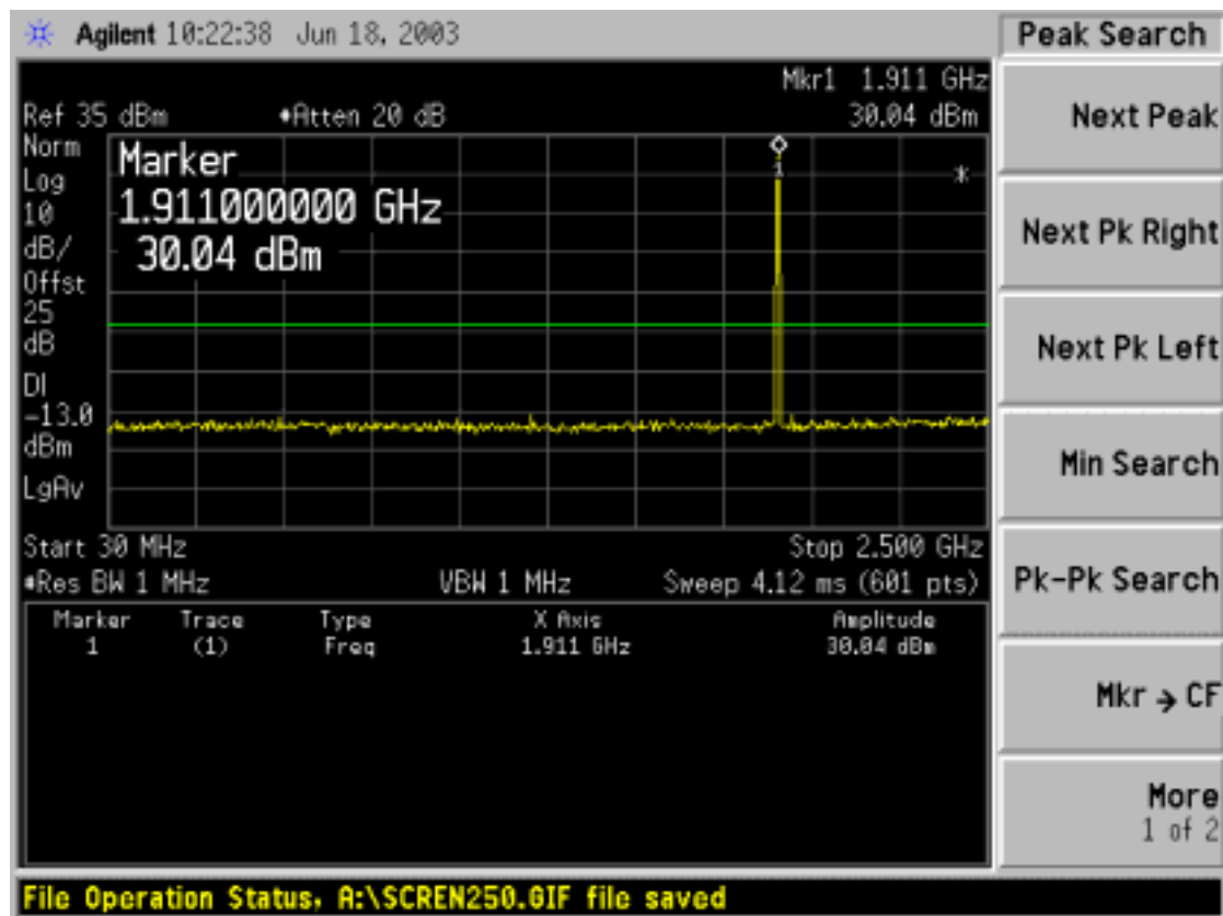
Figure 8-6: Out of Band emission at antenna terminals–GSM Channel High
