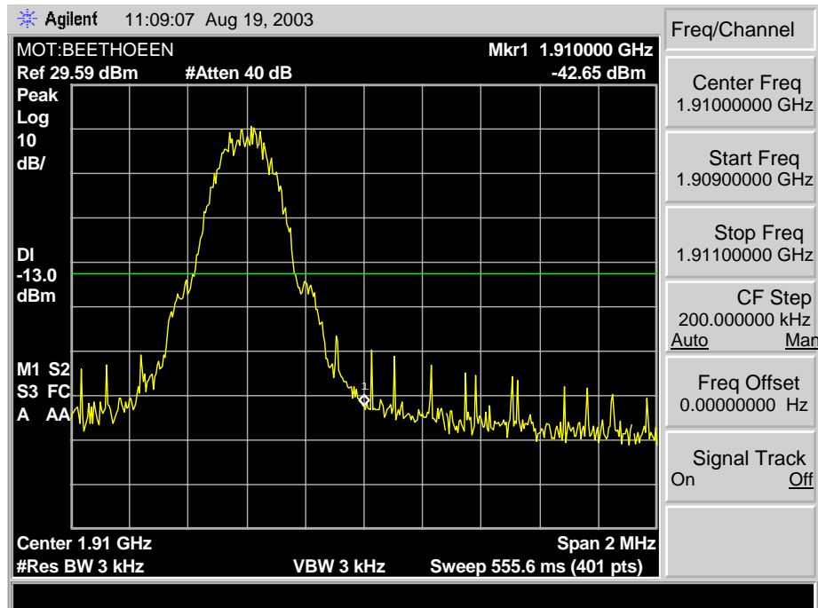
GSM 1900 C5 Max. Block Edge
