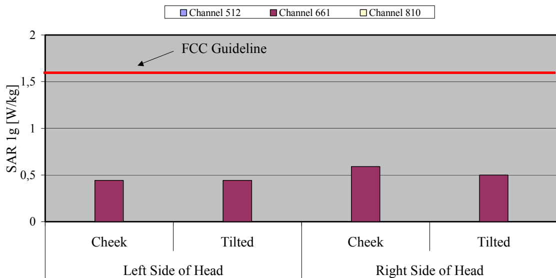
Fig. 7: The measured head phantom SAR values for the Chi Mei Communication Systems, Inc. Wolfgang for PCS 1900 in comparison to the FCC exposure limit.
