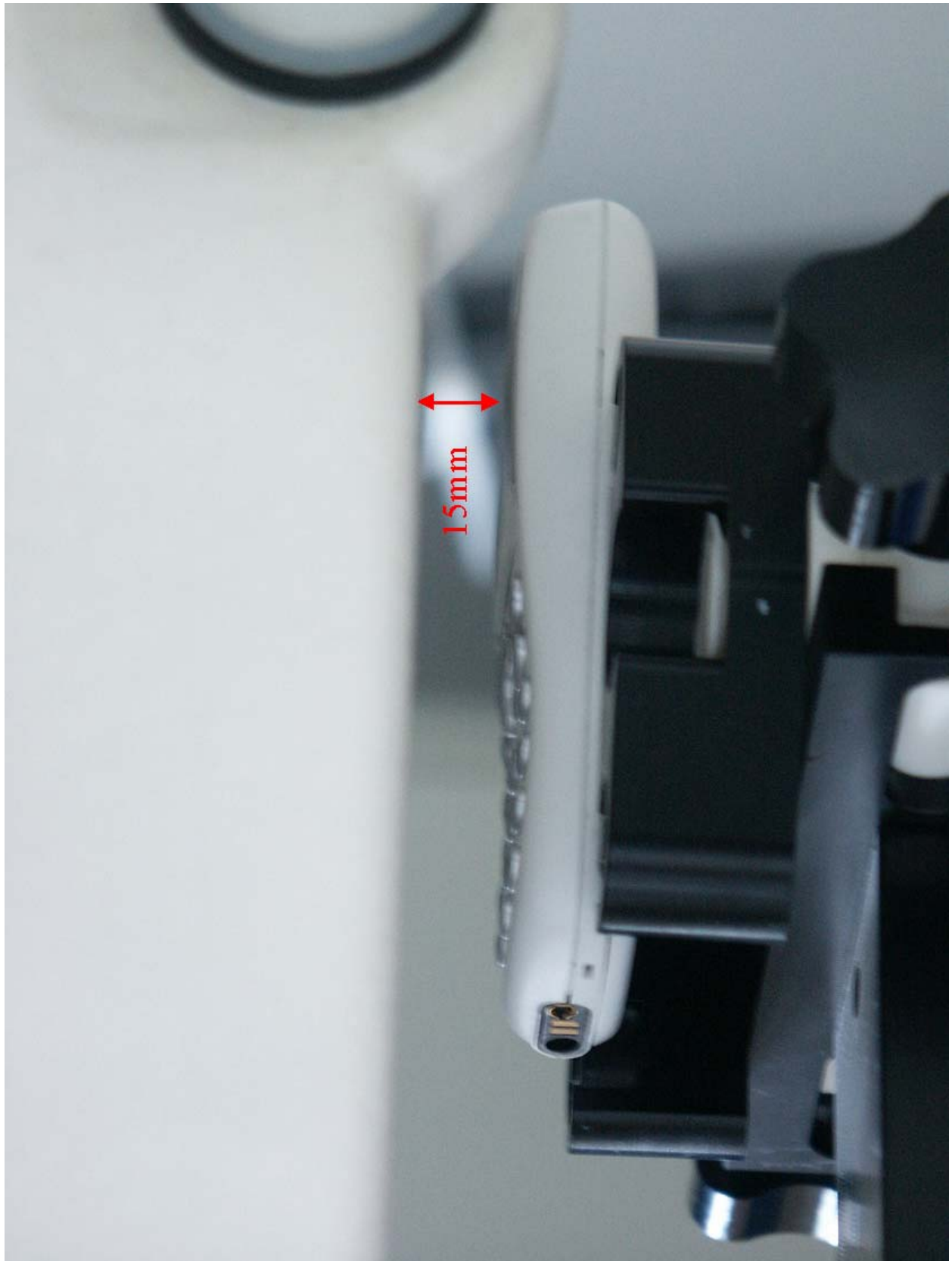
Fig. 23: Body worn configuration without headset, antenna towards the ground.
