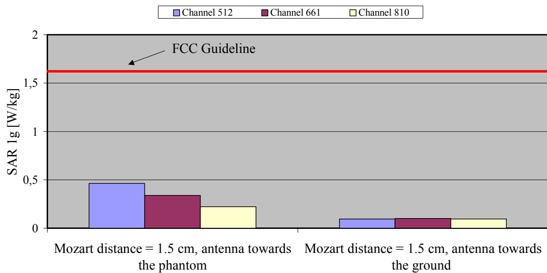
Fig. 9: The measured SAR values in body-worn configuration without headset for the Chi Mei Communication Systems, Inc. Wolfgang for PCS 1900 in comparison to the FCC exposure limit.
