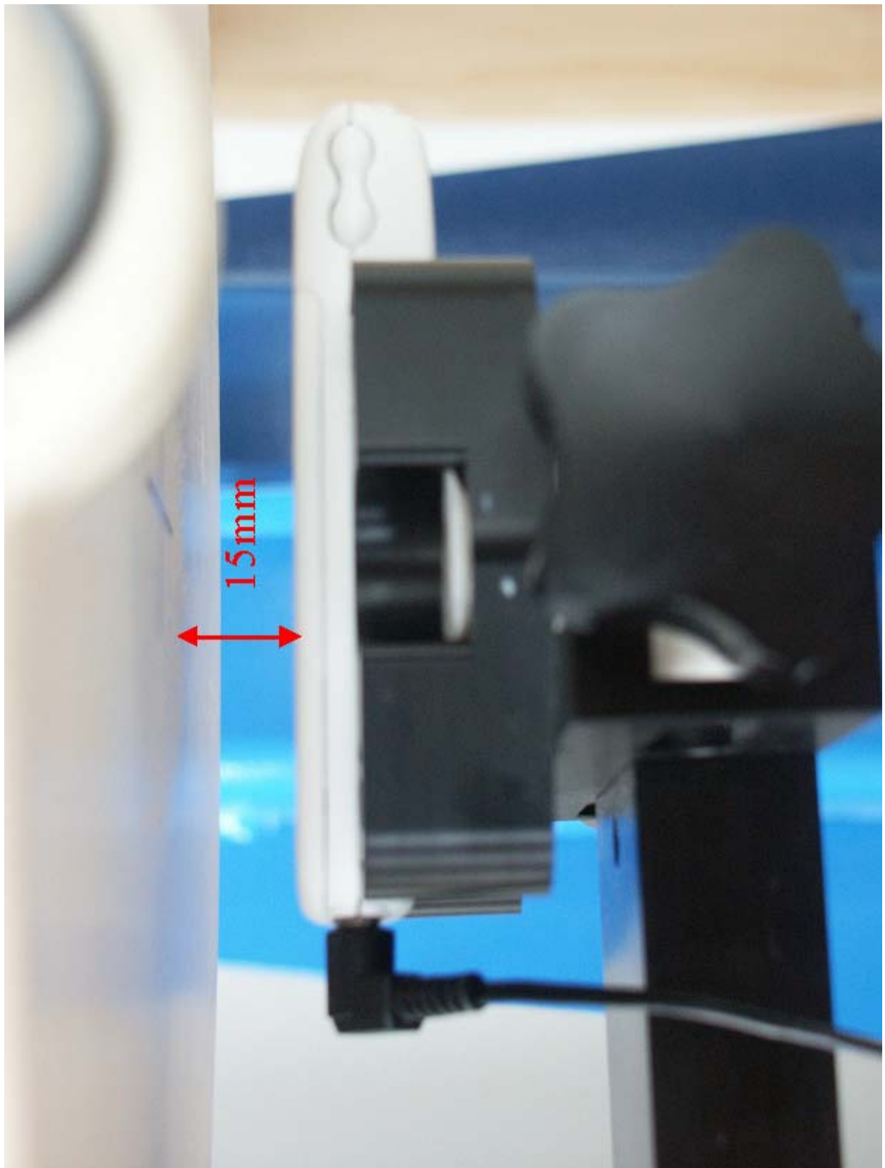
Fig. 20: Body worn configuration talk mode with headset, antenna towards the phantom.
