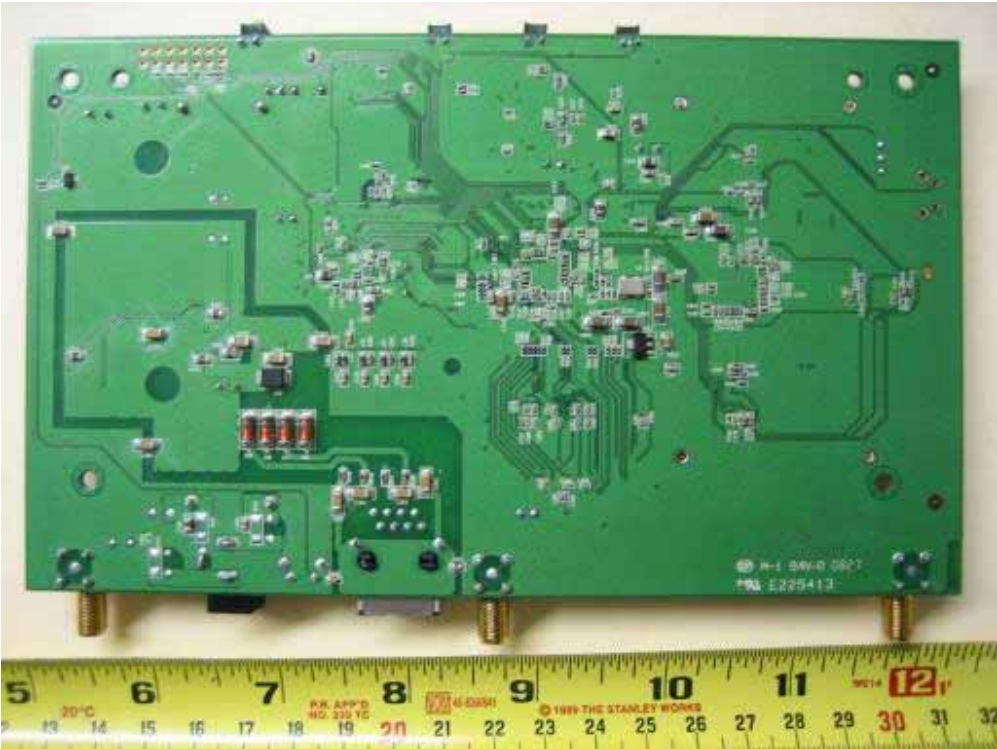
Solder View
