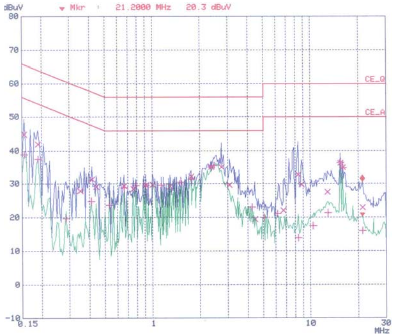
< Neutral line >
