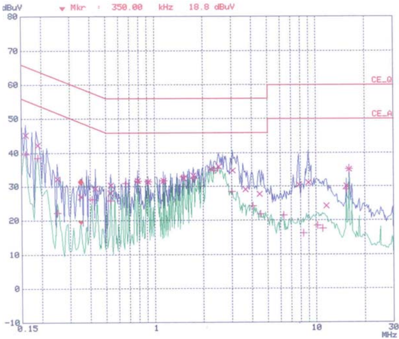
< Hot line >
