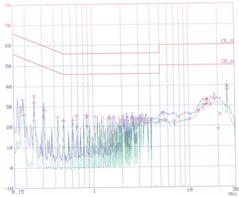
< Hot line >
