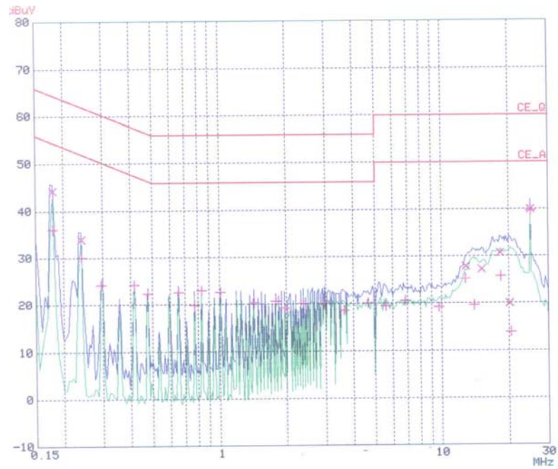
< Hot line >
