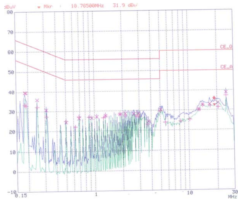
< Neutral line >
