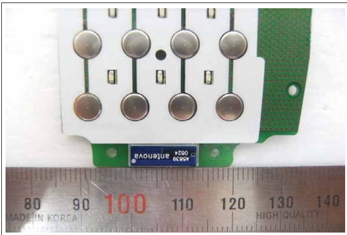
(Bluetooth Antenna)
