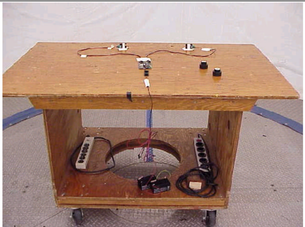
Radiated Emissions EUT Setup in Open Area Test Site (free standing - Test configuration #1)
