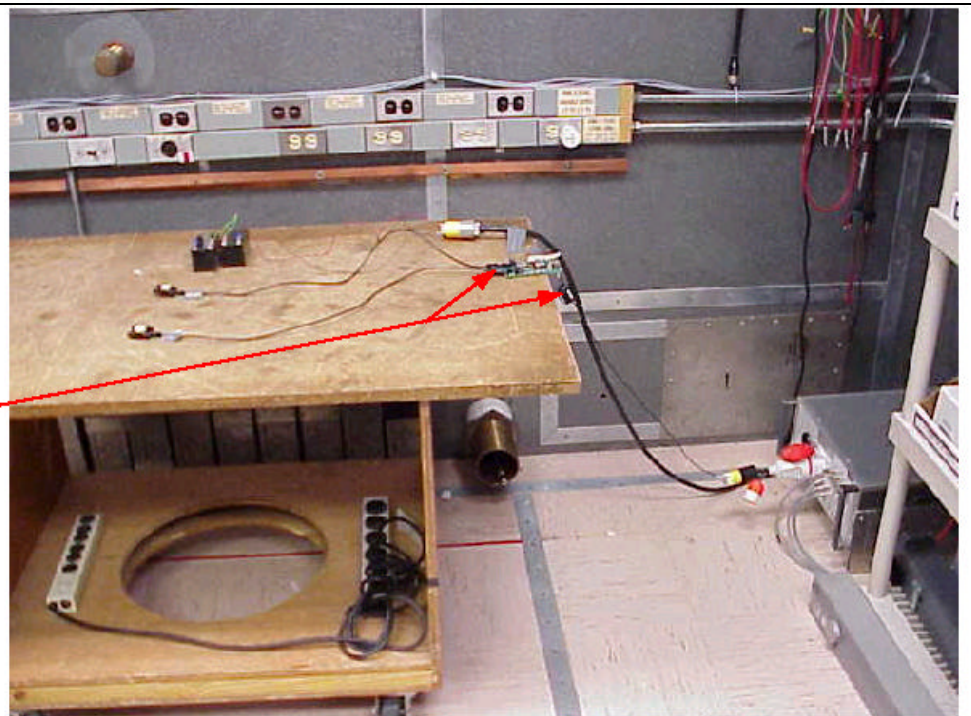
Conducted Emissions (free standing - Test configuration #1)
