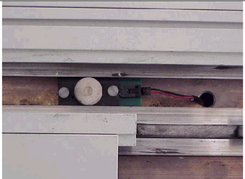
EUT in enclosure showing antenna coil
