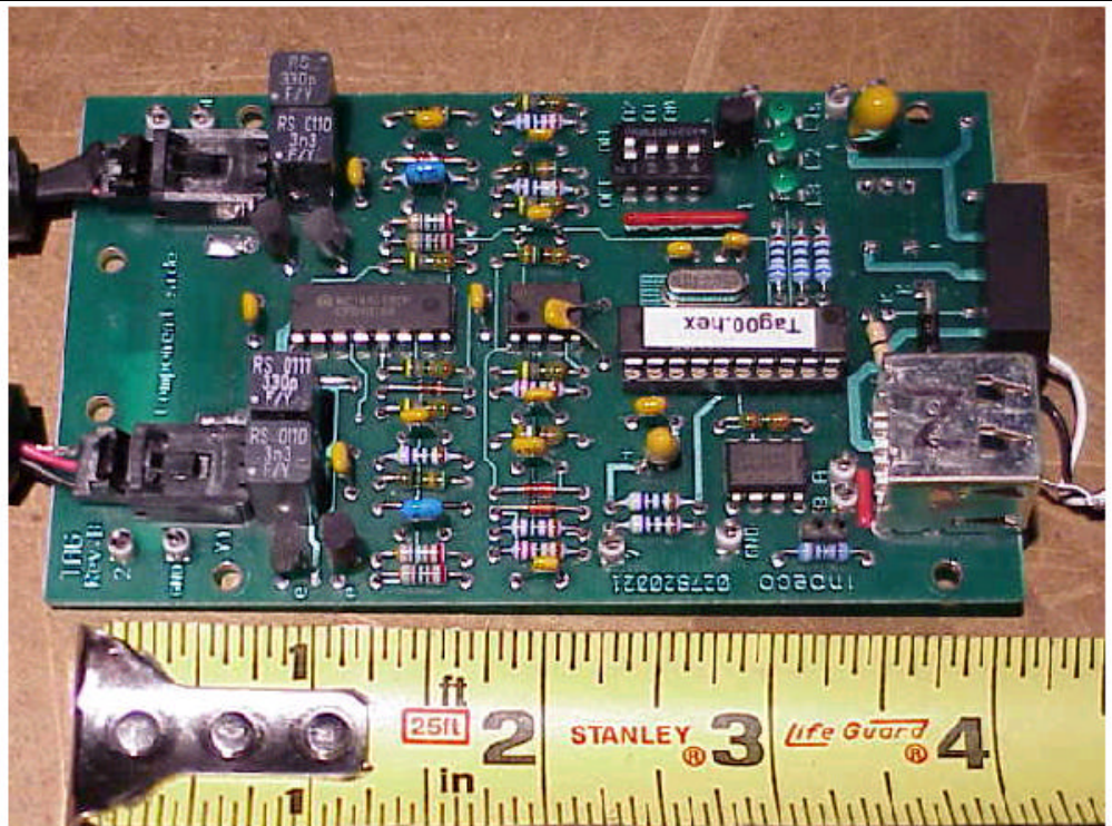
Close up top view of RF Receiver
