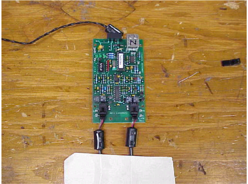
Close up view of Receiver RF Module showing ferrites
