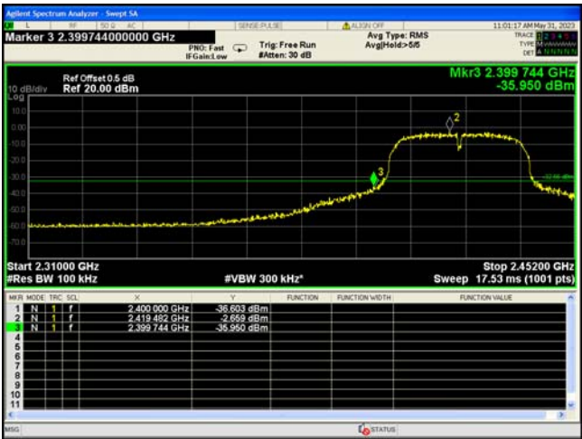
TX 11n HT40: Band edge-left side
