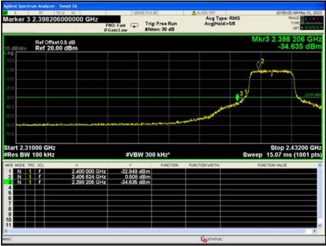
TX 11n HT20: Band edge-left side
