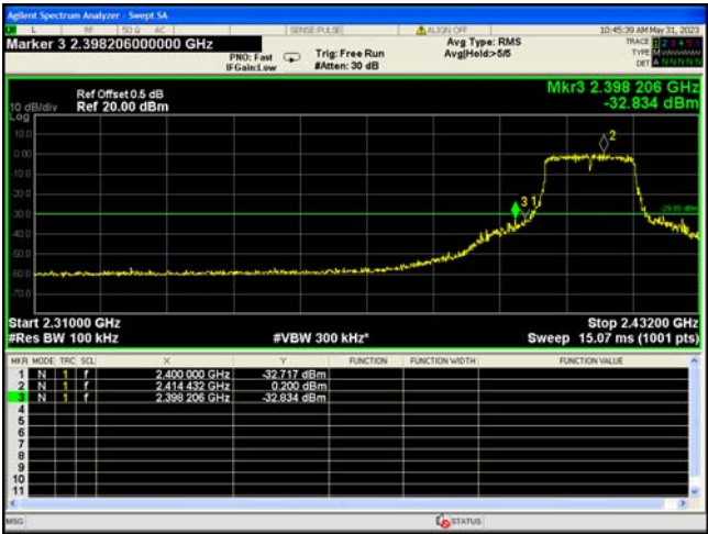
TX 11g: Band edge-left side
