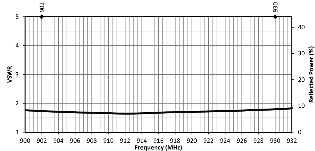
Figure 3. ANT-916-CW-RCL VSWR
