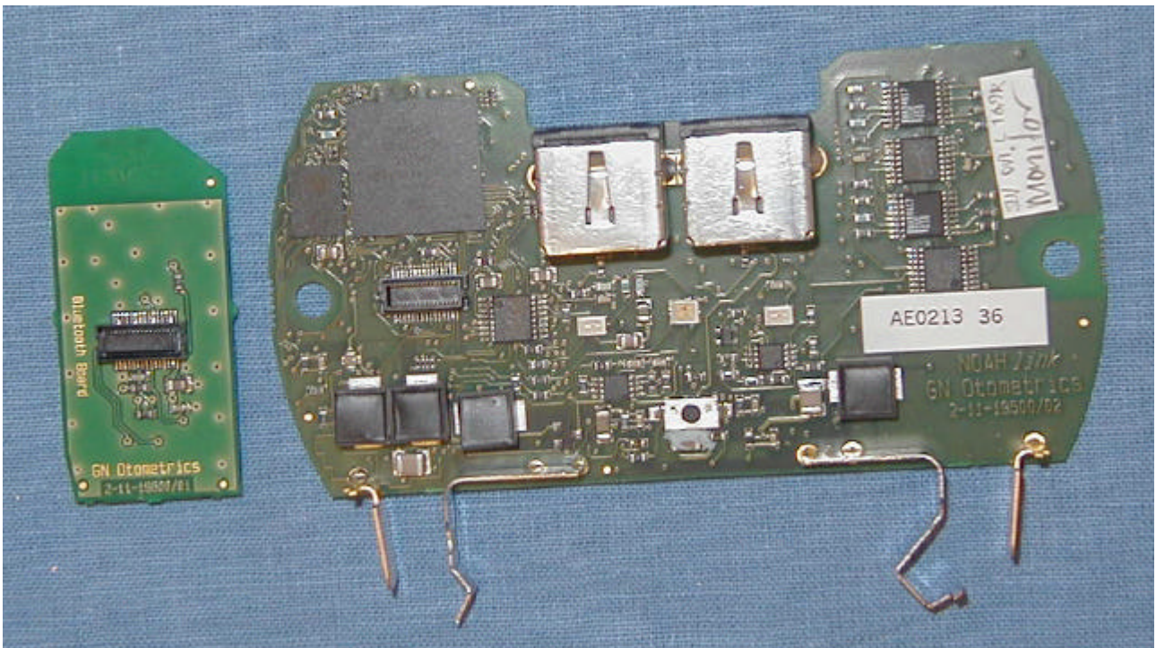
Internal photo of EUT, bottom side (BT radio module removed)
