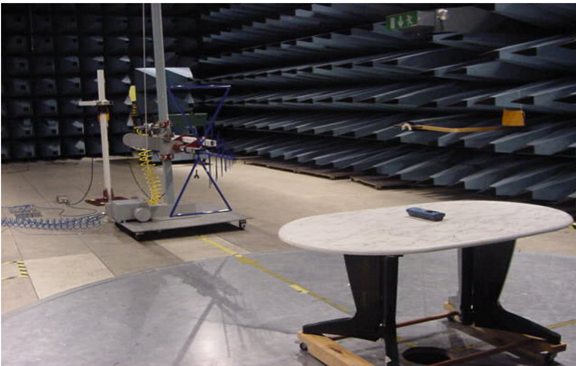
Radiated spurious emissions (30 - 1000 MHz)
