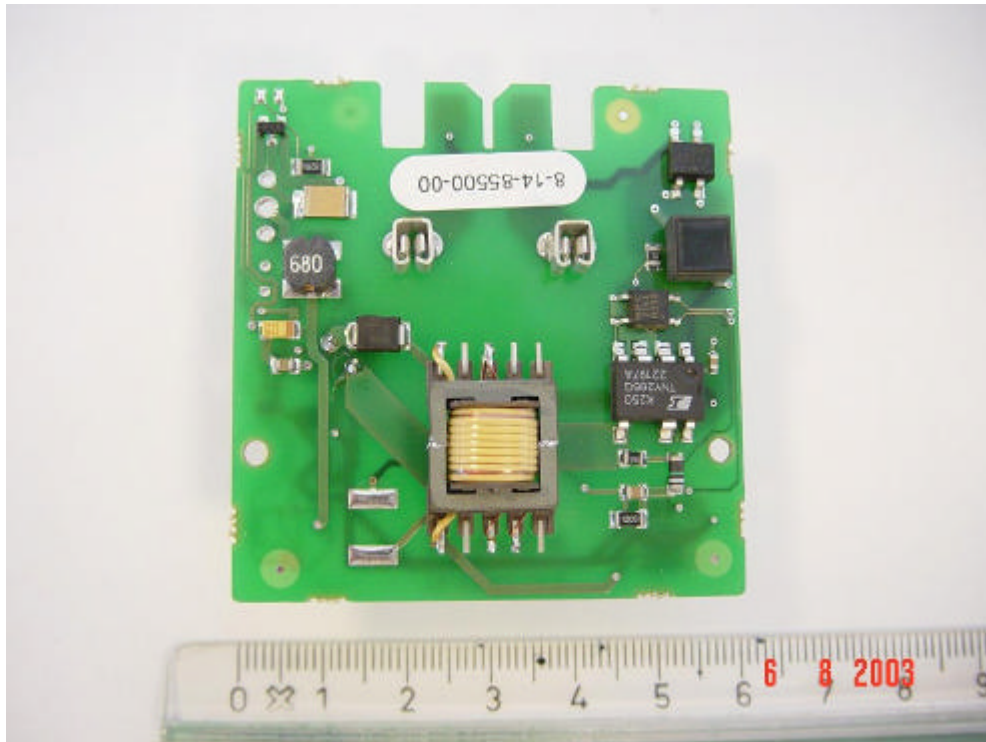
Charger board, bottom
