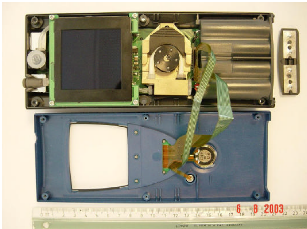
Inside of hand held unit
