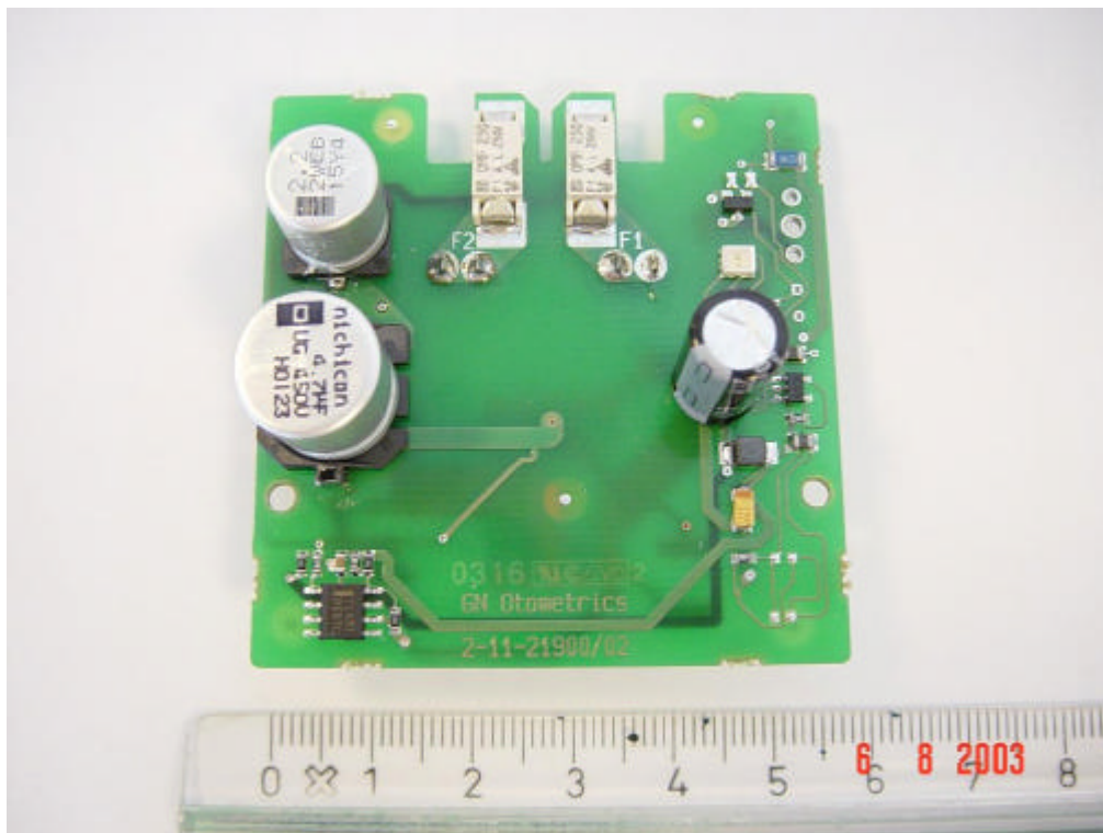
Charger board, top
