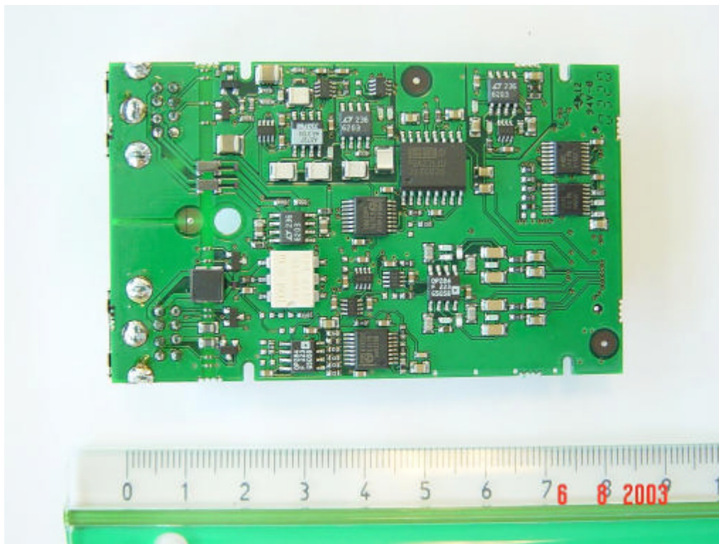
Front board, bottom
