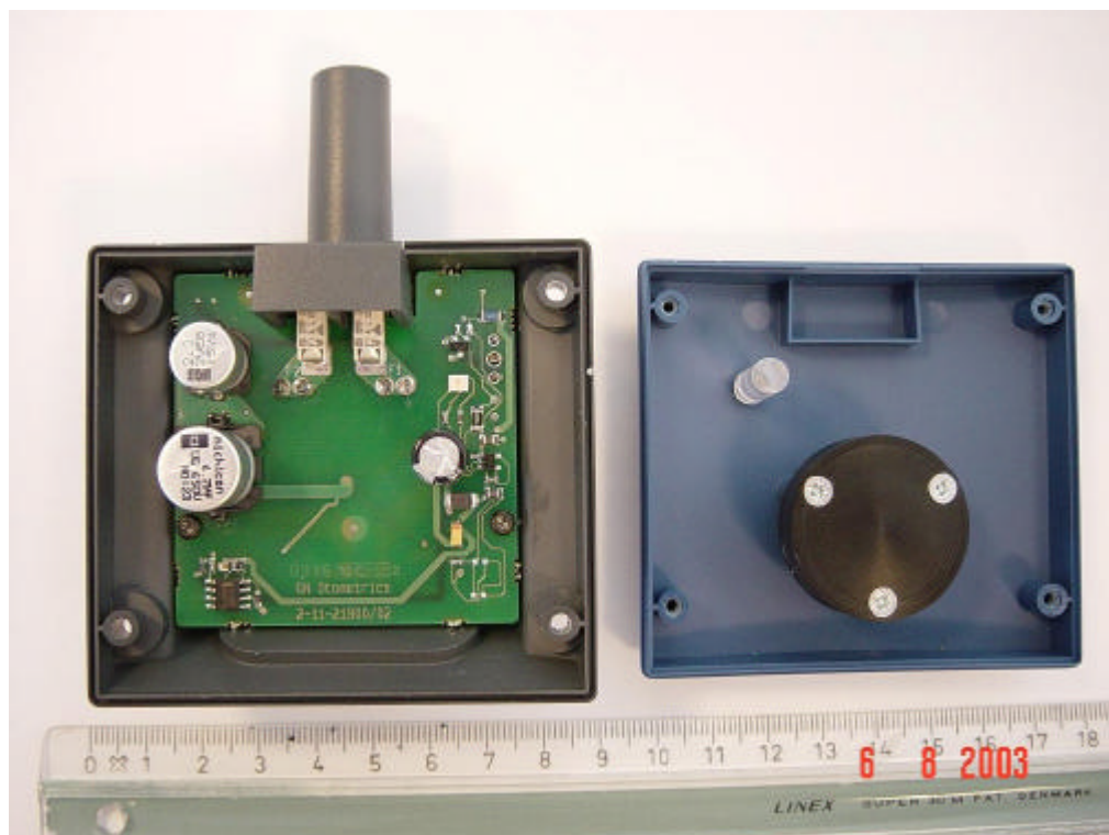
Inside of charger unit
