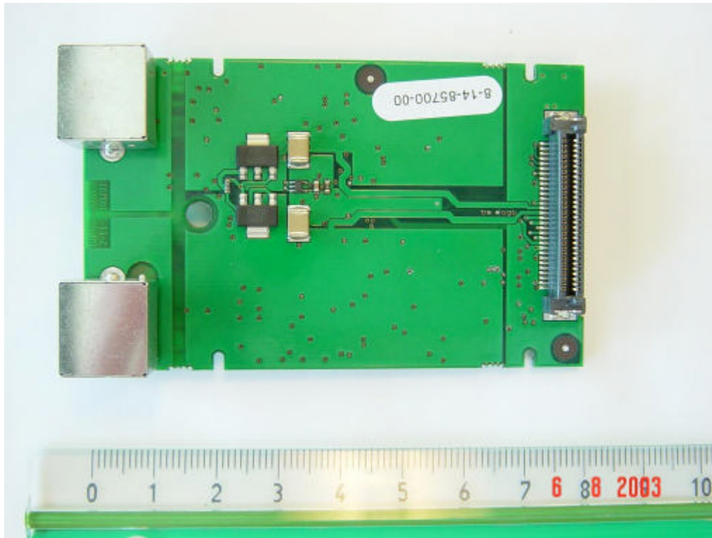
Front board, top
