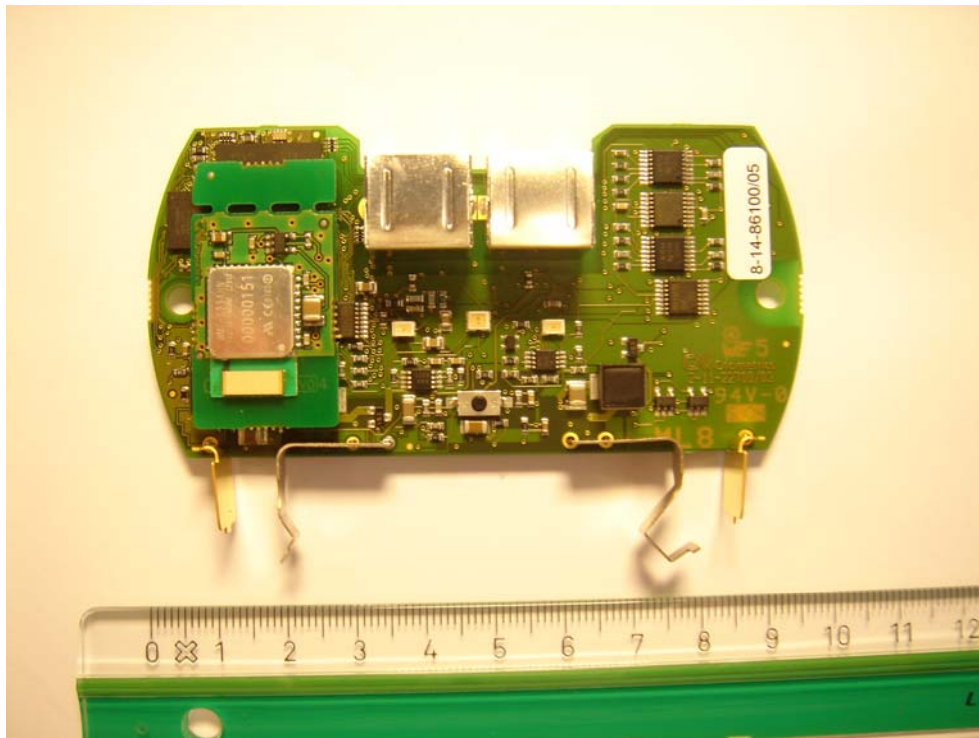
Main board top with bluetooth board
