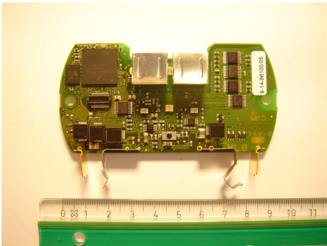
Main board top without bluetooth board
