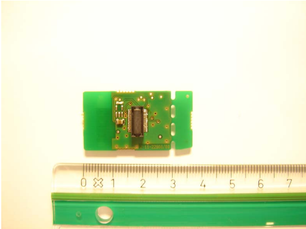
Bluetooth board top
