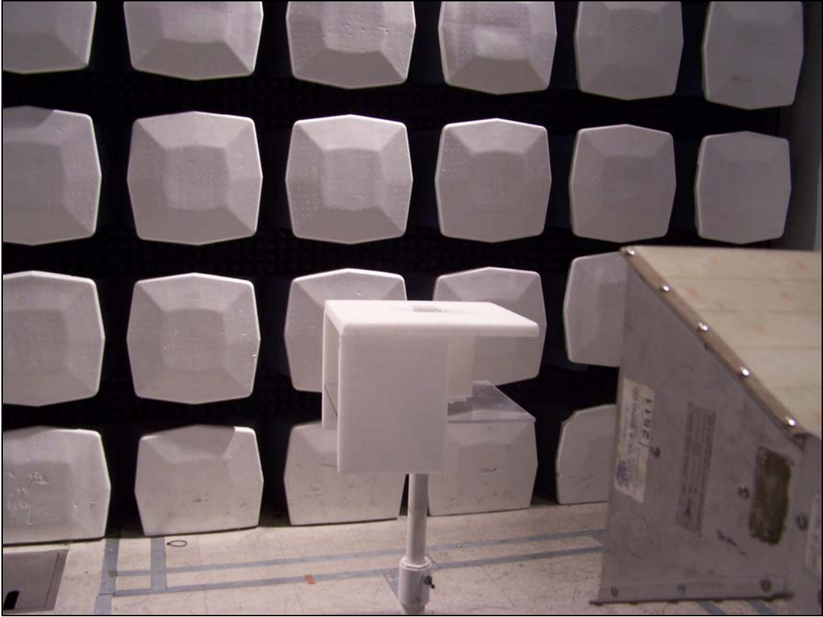
Photograph 4. Peak Test Setup
