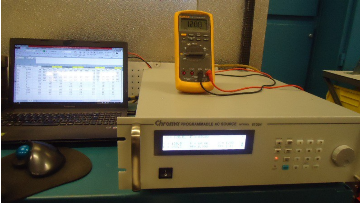
Figure 4.8 - Test Setup - Power system
