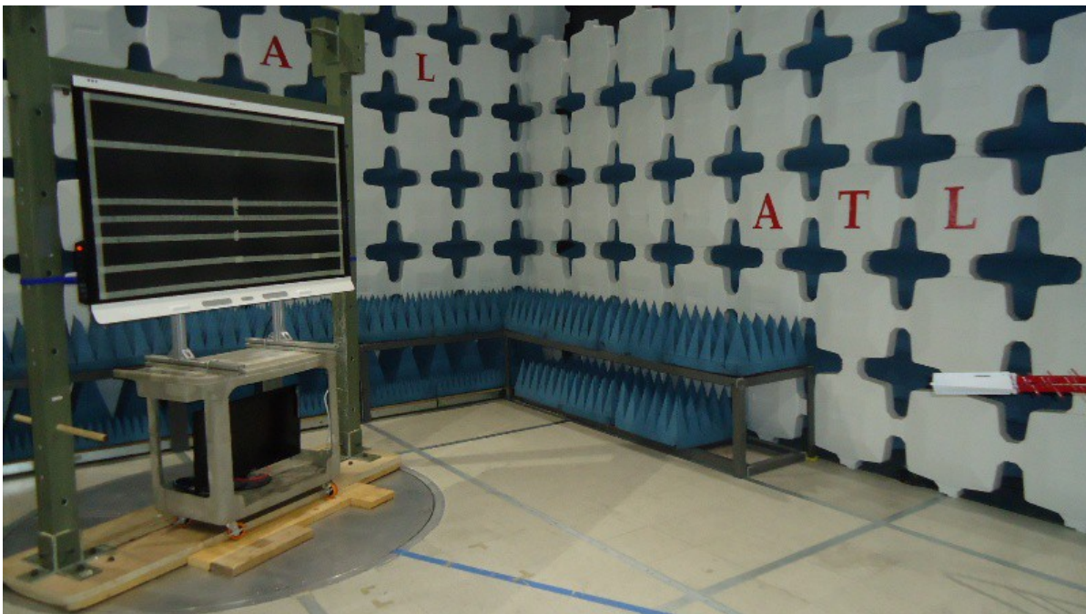
Figure 4.7b - Test Setup - Side View
