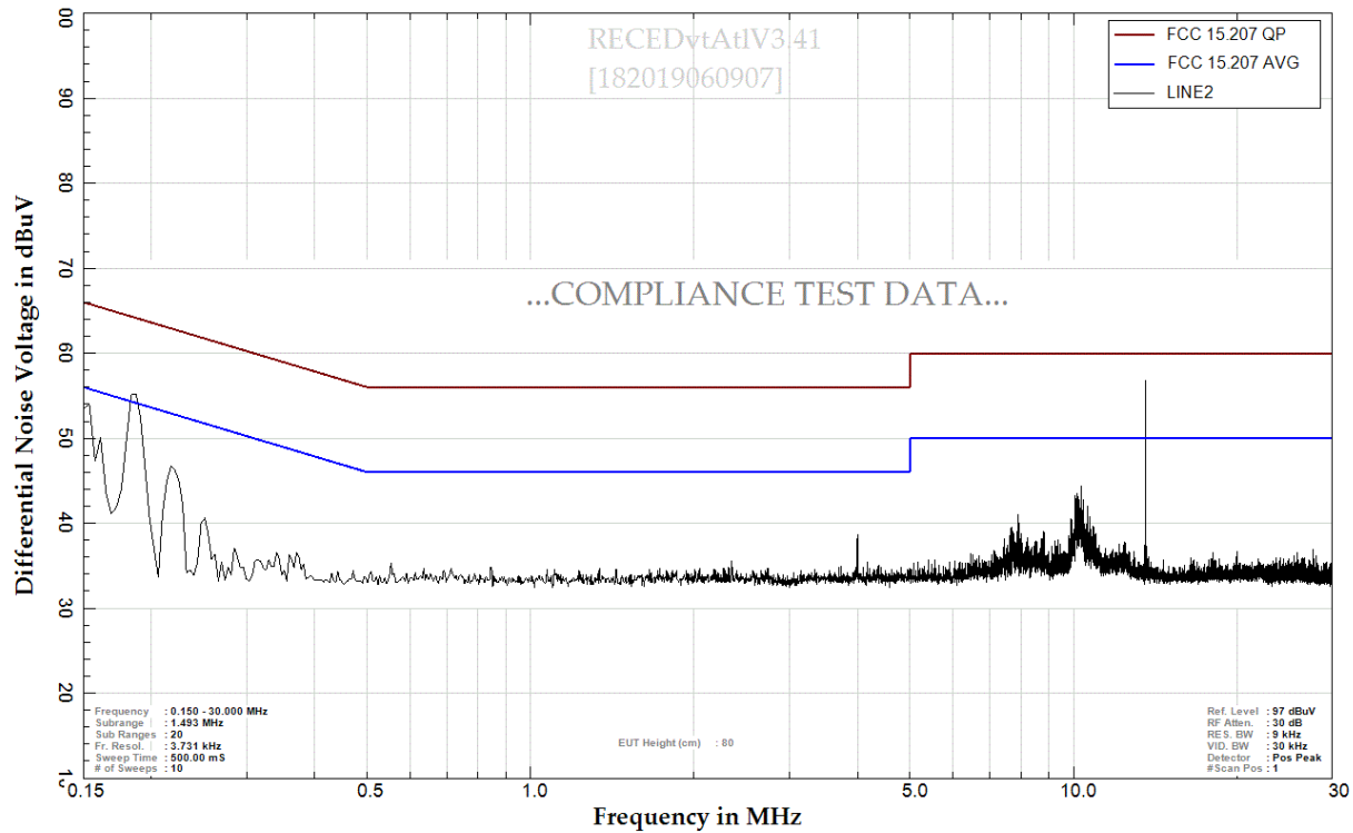
Figure 6.3 - AC Power Line Conducted Emission Scan Line 2 (Line N)
