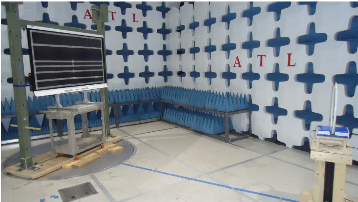
Figure 1.2 - Test Setup - Side View
