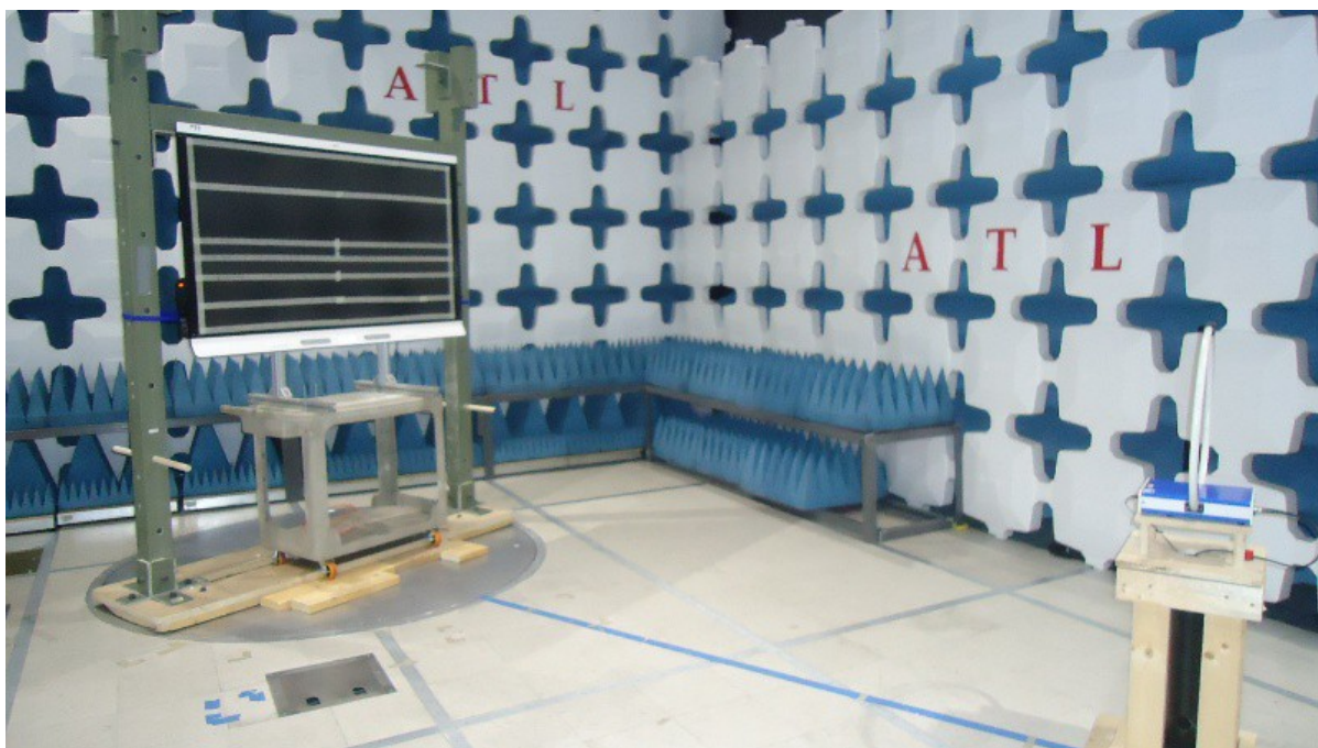
Figure 1.6a - Test Setup - Side View
