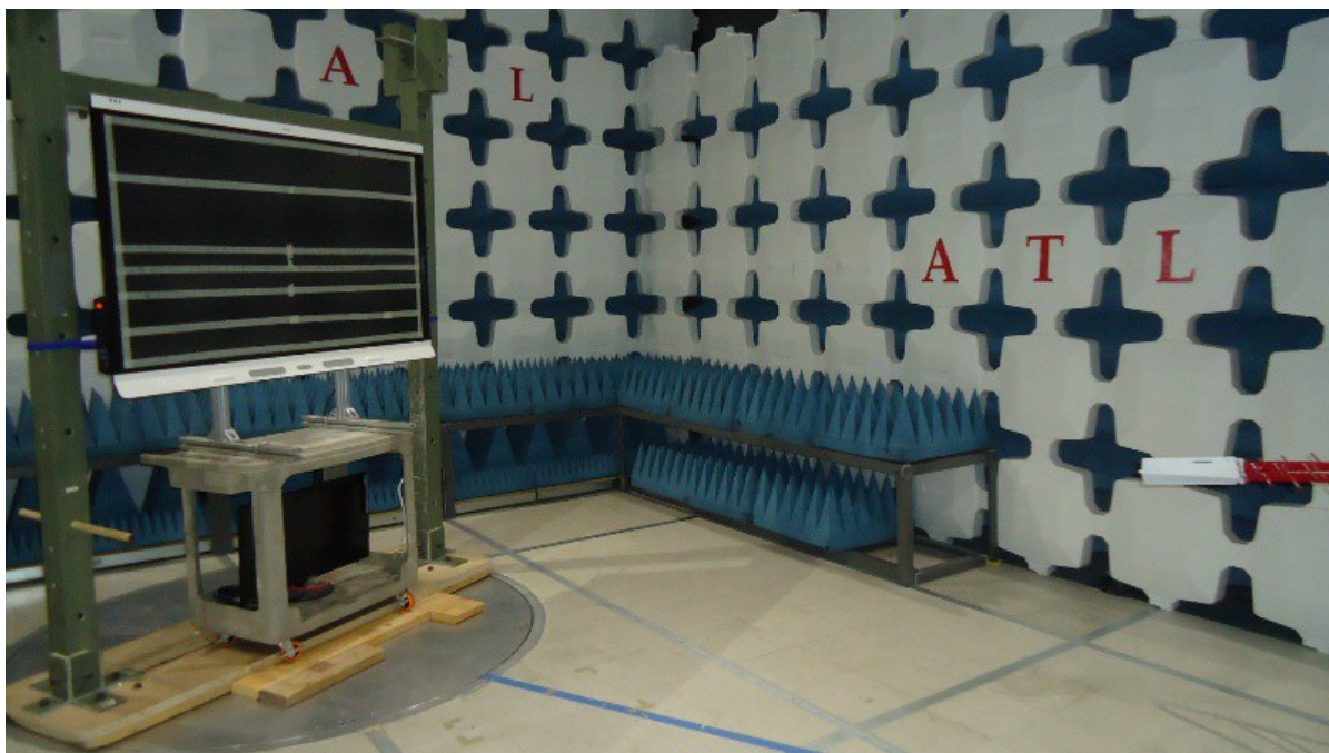
Figure 1.6b - Test Setup - Side View
