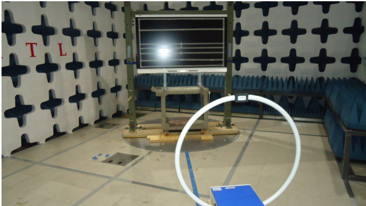
Figure 1.5a - Test Setup - Front View
