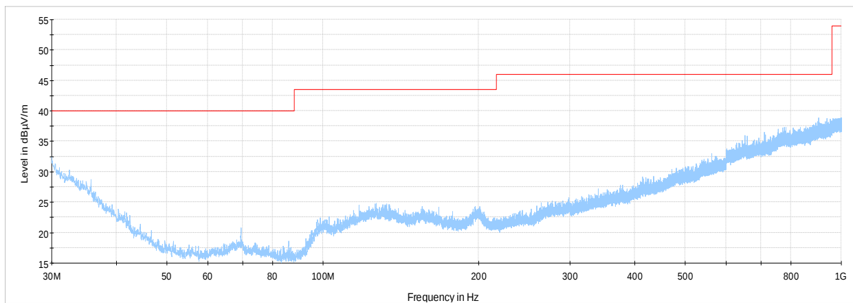
Figure 8.3-8: Radiated spurious emissions for high channel below 1 GHz for restricted band emissions
