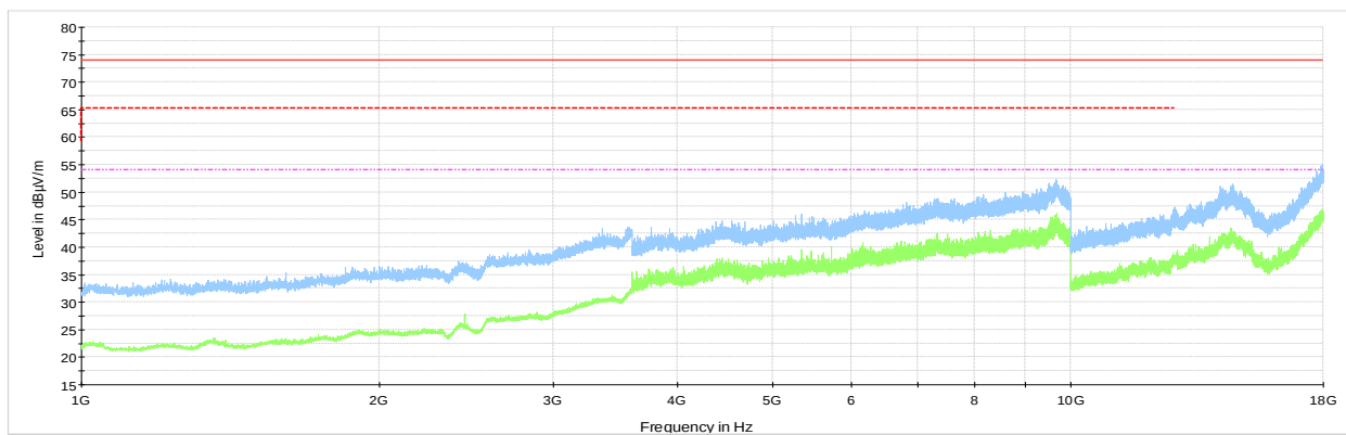
Figure 8.3-10: Radiated spurious emissions for mid channel above 1 GHz for restricted band emissions
