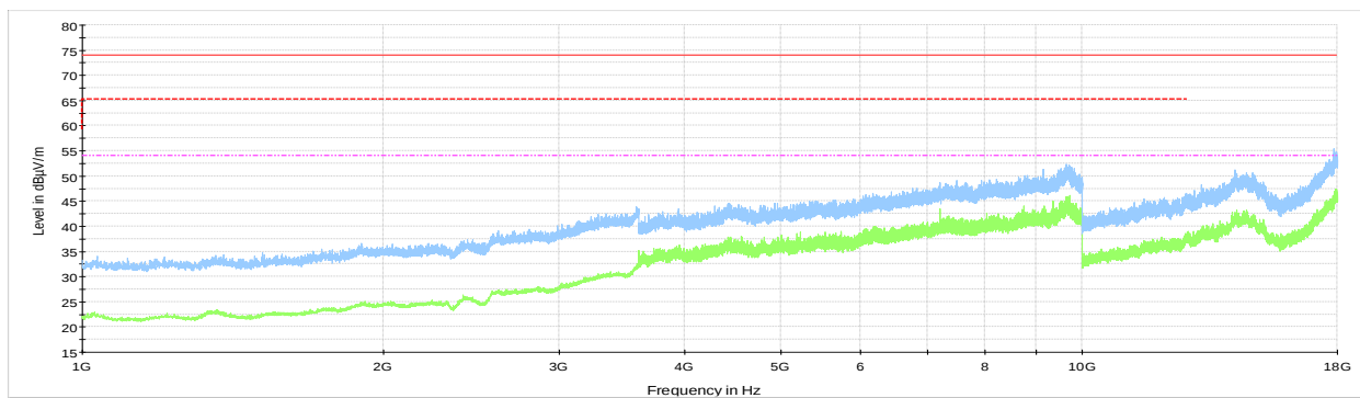
Figure 8.3-11: Radiated spurious emissions for high channel above 1 GHz for restricted band emissions
