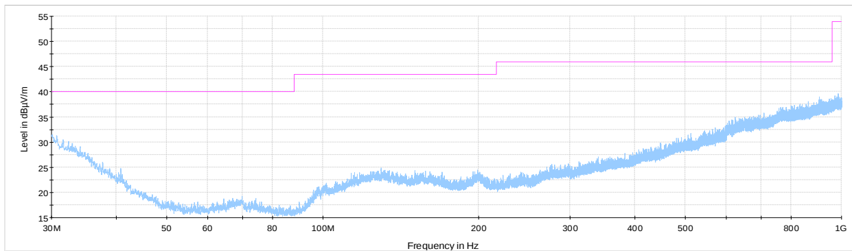
Figure 8.3-7: Radiated spurious emissions for mid channel below 1 GHz for restricted band emissions
