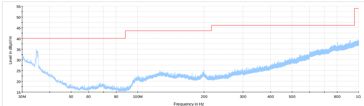
Figure 8.3-6: Radiated spurious emissions for low channel below 1 GHz for restricted band emissions
