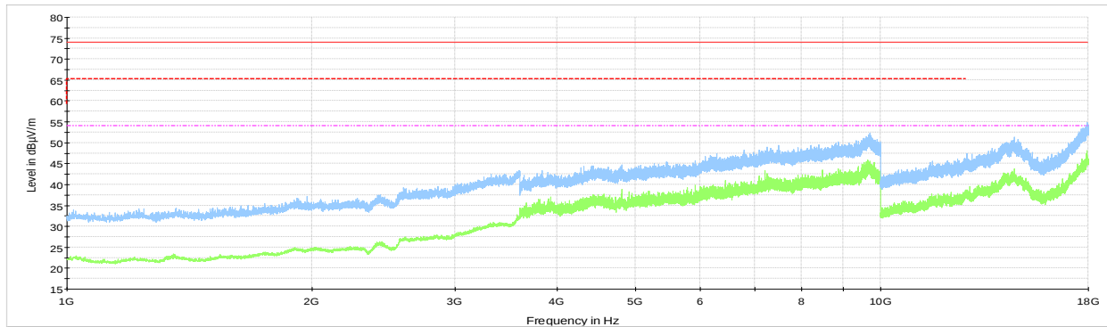
Figure 8.3-9: Radiated spurious emissions for low channel above 1 GHz for restricted band emissions
