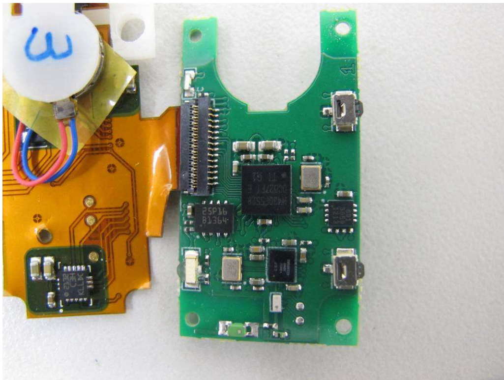
Fig. 2: Internal view
