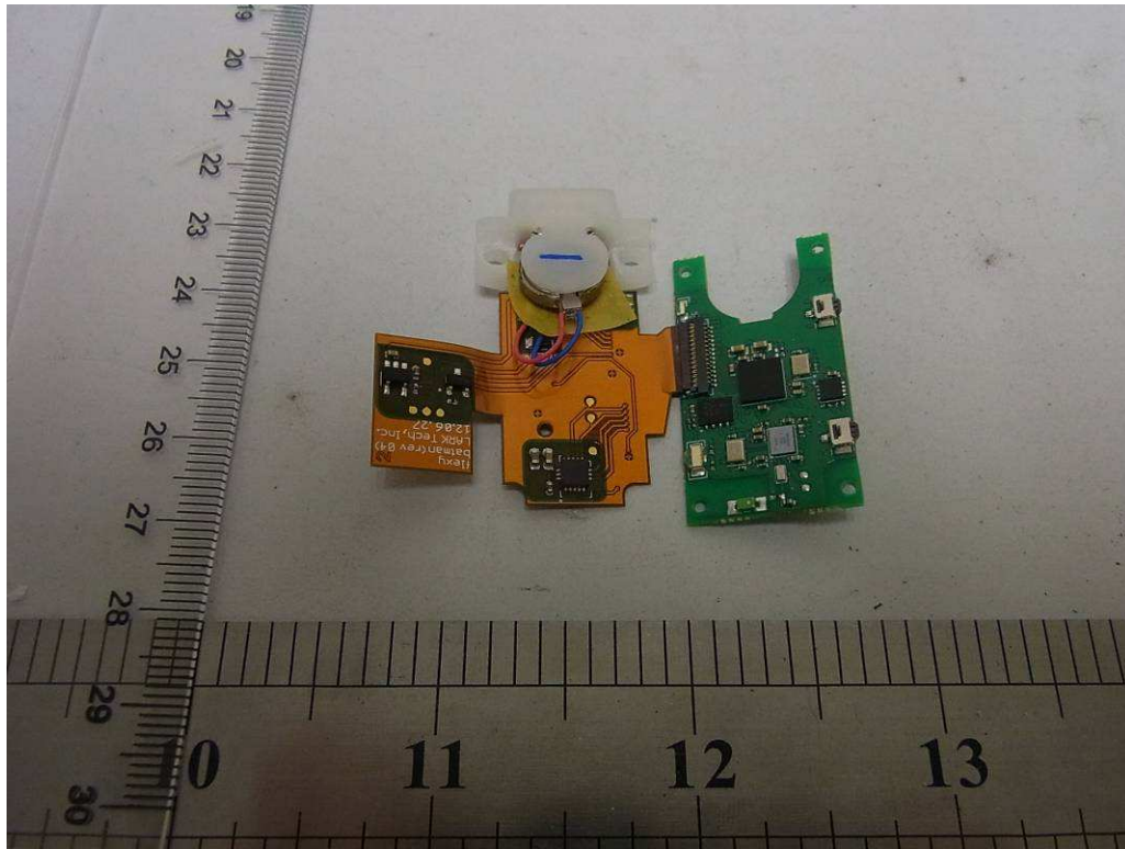
Fig. 1: Internal view
