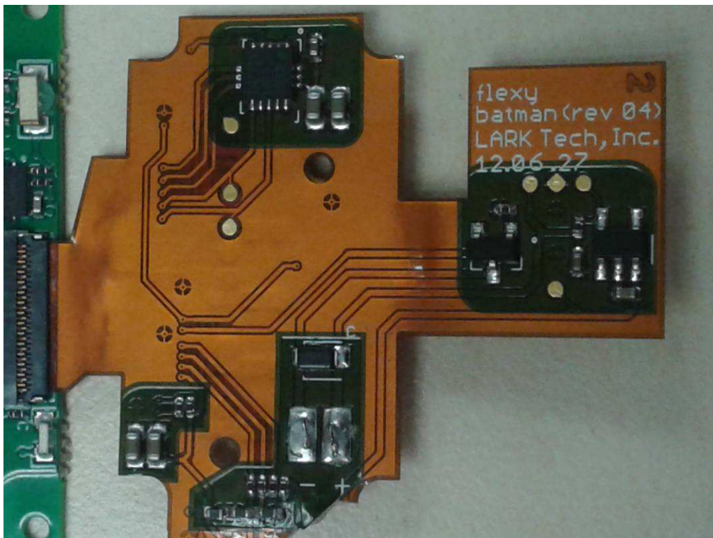
Fig. 6: Internal view
