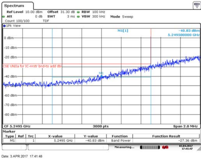
Figure 8.4-301: Lower band edge for ISSED, 10 MHz channel, 32 dBi antenna, BPSK
