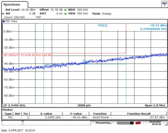
Figure 8.4-303: Lower band edge for ISSED, 20 MHz channel, 32 dBi antenna, BPSK
