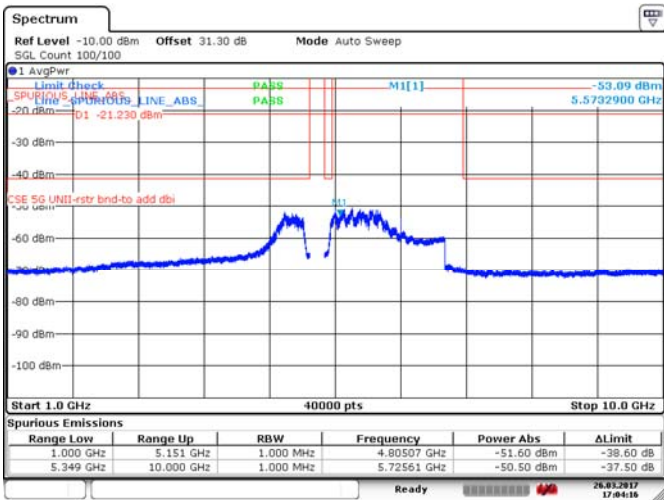
Figure 8.4-250: Average Spurious emissions within restricted bands, 20 MHz channel, mid channel, 32 dBi antenna, cho, BPSK
