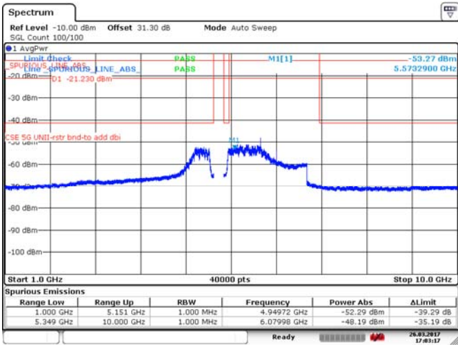
Figure 8.4-252: Average Spurious emissions within restricted bands, 20 MHz channel, mid channel, 32 dBi antenna, cho, 256-QAM
