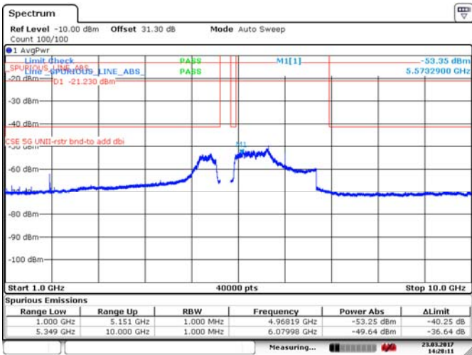
Figure 8.4-218: Average Spurious emissions within restricted bands, 10 MHz channel, low channel, 32 dBi antenna, cho, BPSK
