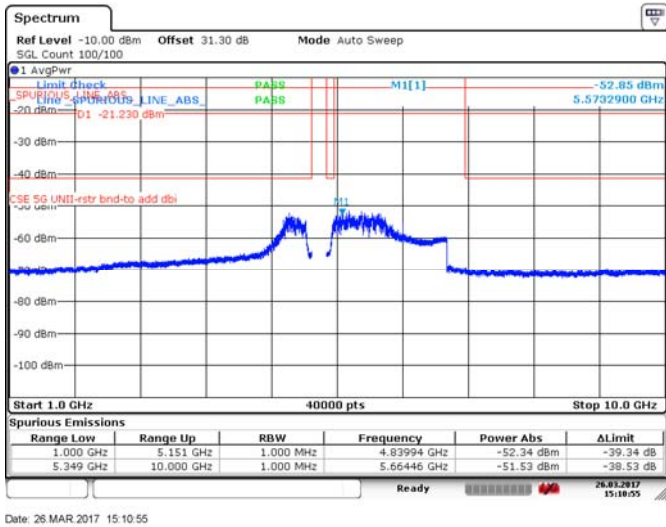
Figure 8.4-284: Average Spurious emissions within restricted bands, 40 MHz channel, high channel, 32 dBi antenna, cho, 256-QAM
