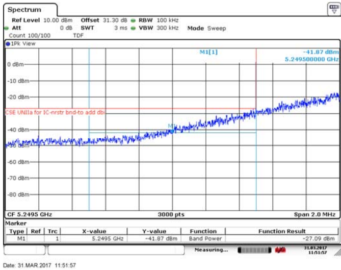
Figure 8.4-302: Lower band edge for ISSED, 10 MHz channel, 32 dBi antenna, 256QAM
