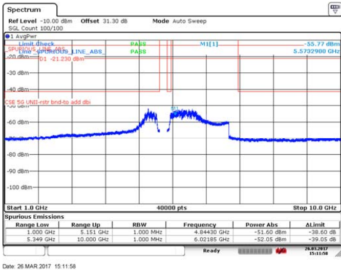
Figure 8.4-282: Average Spurious emissions within restricted bands, 40 MHz channel, high channel, 32 dBi antenna, cho, BPSK
