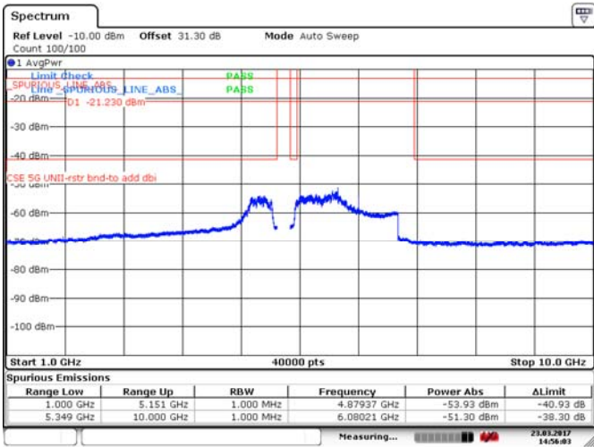
Figure 8.4-220: Average Spurious emissions within restricted bands, 10 MHz channel, low channel, 32 dBi antenna, cho, 256QAM
