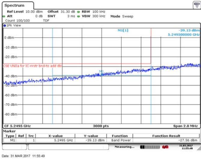
Figure 8.4-304: Lower band edge for ISSED, 20 MHz channel, 32 dBi antenna, 256QAM
