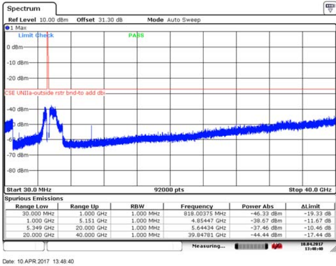
Figure 8.4-182: Spurious emissions outside restricted bands, 10 MHz channel, low channel, 32 dBi antenna, ch1, BPSK
