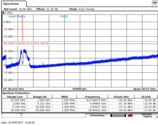
Figure 8.4-200: Spurious emissions outside restricted bands, 20 MHz channel, mid channel, 32 dBi antenna, ch1, 256-QAM
