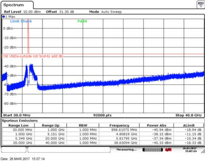
Figure 8.4-211: Spurious emissions outside restricted bands, 40 MHz channel, mid channel, 32 dBi antenna, cho, 256-QAM
