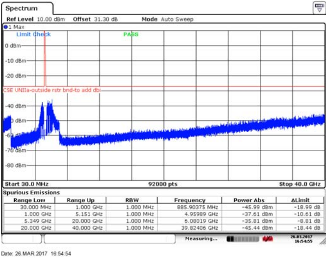
Figure 8.4-193: Spurious emissions outside restricted bands, 20 MHz channel, low channel, 32 dBi antenna, cho, BPSK
