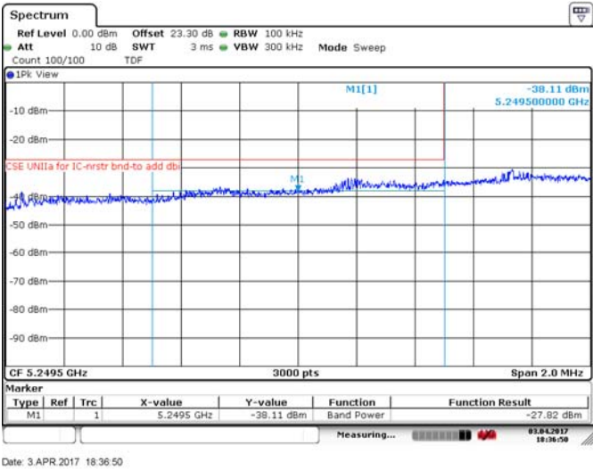
Figure 8.4-179: Lower band edge for ISED, 40 MHz channel, 24 dBi antenna, BPSK
