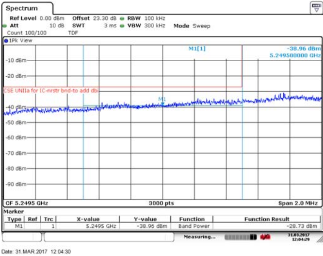
Figure 8.4-180: Lower band edge for ISED, 40 MHz channel, 24 dBi antenna, 256QAM
