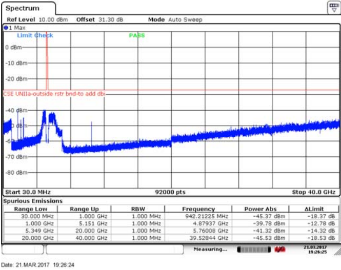
Figure 8.4-183: Spurious emissions outside restricted bands, 10 MHz channel, low channel, 32 dBi antenna, cho, 256QAM
