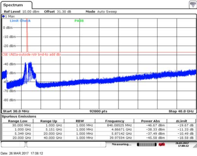
Figure 8.4-201: Spurious emissions outside restricted bands, 20 MHz channel, high channel, 32 dBi antenna, cho, BPSK
