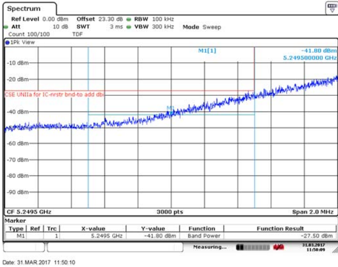
Figure 8.4-176: Lower band edge for ISED, 10 MHz channel, 24 dBi antenna, 256QAM
