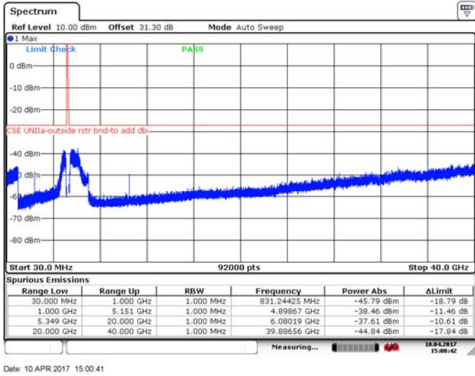
Figure 8.4-208: Spurious emissions outside restricted bands, 40 MHz channel, low channel, 32 dBi antenna, ch1, 256QAM
