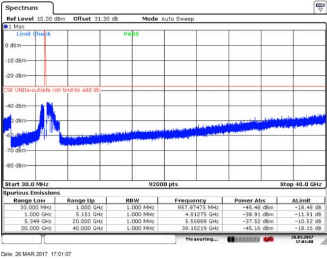
Figure 8.4-199: Spurious emissions outside restricted bands, 20 MHz channel, mid channel, 32 dBi antenna, cho, 256-QAM
