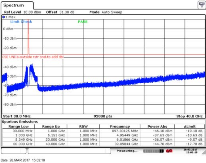
Figure 8.4-209: Spurious emissions outside restricted bands, 40 MHz channel, mid channel, 32 dBi antenna, cho, BPSK
