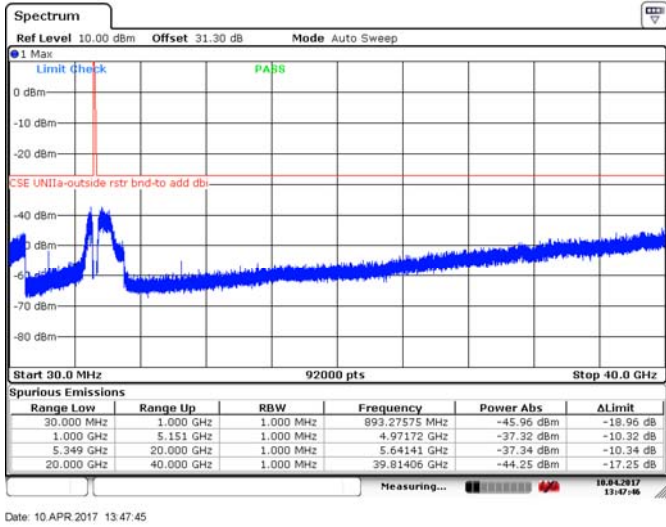
Figure 8.4-184: Spurious emissions outside restricted bands, 10 MHz channel, low channel, 32 dBi antenna, ch1, 256QAM
