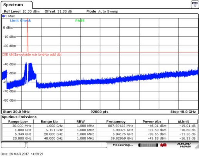
Figure 8.4-207: Spurious emissions outside restricted bands, 40 MHz channel, low channel, 32 dBi antenna, cho, 256QAM
