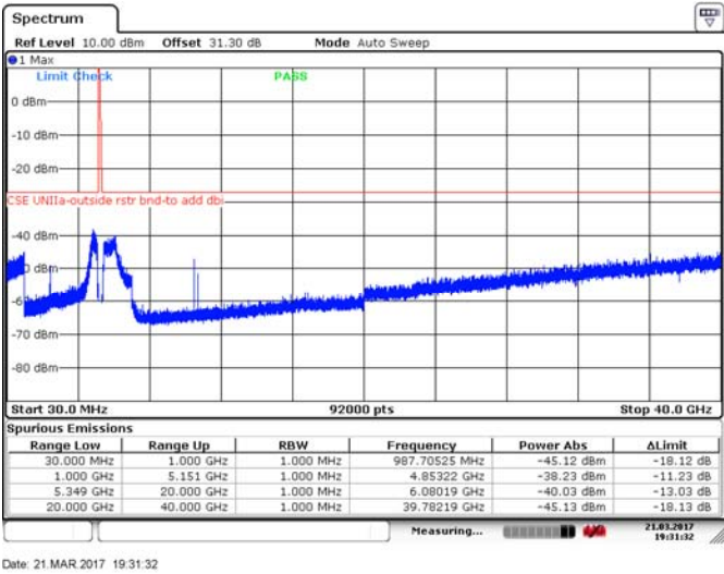
Figure 8.4-189: Spurious emissions outside restricted bands, 10 MHz channel, high channel, 32 dBi antenna, cho, BPSK
