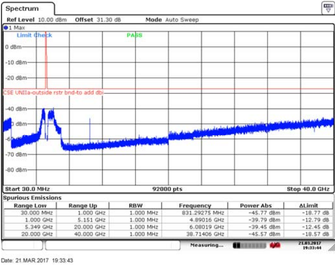
Figure 8.4-181: Spurious emissions outside restricted bands, 10 MHz channel, low channel, 32 dBi antenna, cho, BPSK
