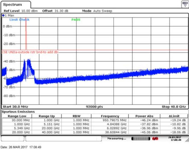
Figure 8.4-203: Spurious emissions outside restricted bands, 20 MHz channel, high channel, 32 dBi antenna, cho, 256-QAM
