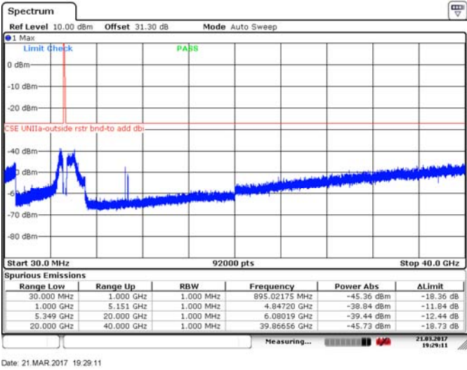
Figure 8.4-191: Spurious emissions outside restricted bands, 10 MHz channel, high channel, 32 dBi antenna, cho, 256-QAM
