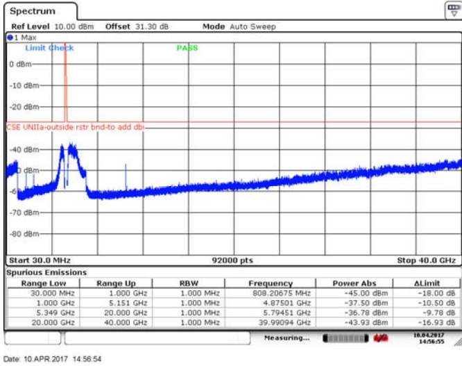
Figure 8.4-212: Spurious emissions outside restricted bands, 40 MHz channel, mid channel, 32 dBi antenna, ch1, 256-QAM
