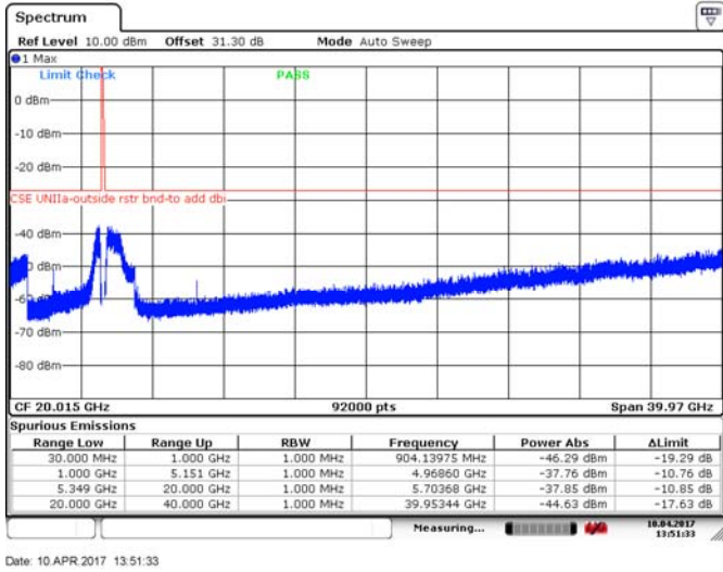
Figure 8.4-192: Spurious emissions outside restricted bands, 10 MHz channel, high channel, 32 dBi antenna, cho, 256-QAM
