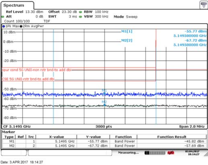
Figure 8.4-167: Lower band edge for FCC, 20 MHz channel, 24 dBi antenna, BPSK
