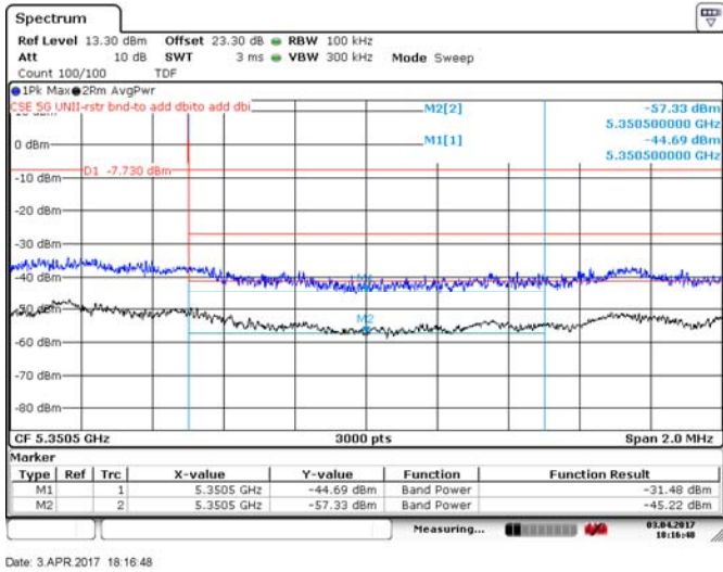
Figure 8.4-168: Upper band edge for FCC, 20 MHz channel, 24 dBi antenna, BPSK
