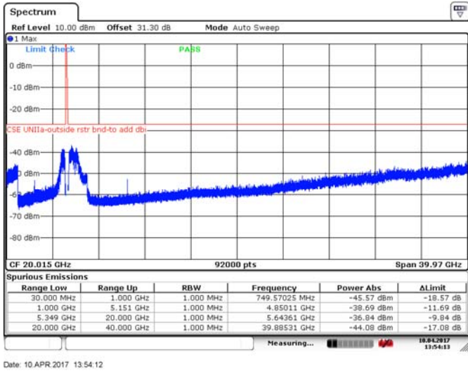
Figure 8.4-194: Spurious emissions outside restricted bands, 20 MHz channel, low channel, 32 dBi antenna, ch1, BPSK
