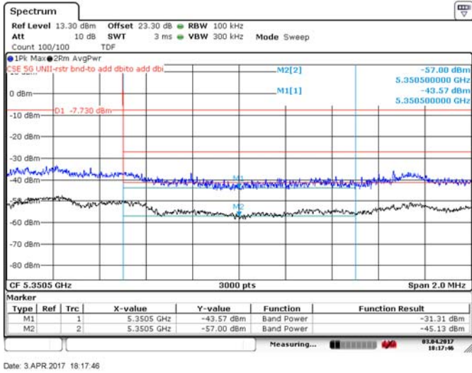
Figure 8.4-170: Upper band edge for FCC, 20 MHz channel, 24 dBi antenna, 256QAM
