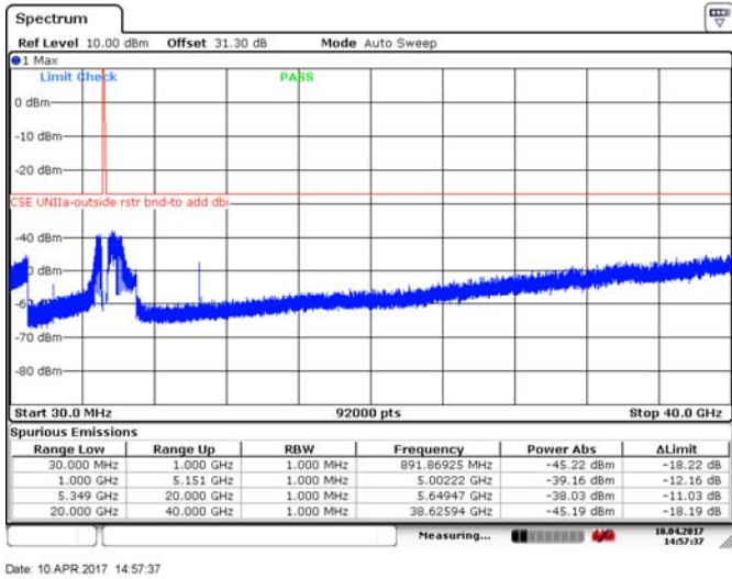
Figure 8.4-210: Spurious emissions outside restricted bands, 40 MHz channel, mid channel, 32 dBi antenna, ch1, BPSK
