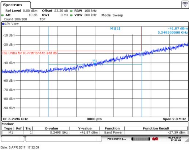
Figure 8.4-175: Lower band edge for ISED, 10 MHz channel, 24 dBi antenna, BPSK
