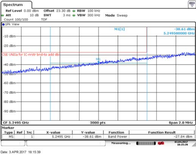
Figure 8.4-177: Lower band edge for ISED, 20 MHz channel, 24 dBi antenna, BPSK
