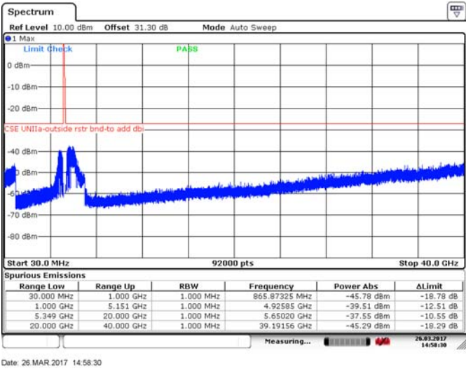
Figure 8.4-205: Spurious emissions outside restricted bands, 40 MHz channel, low channel, 32 dBi antenna, cho, BPSK
