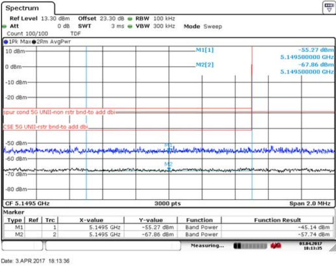
Figure 8.4-169: Lower band edge for FCC, 20 MHz channel, 24 dBi antenna, 256QAM
