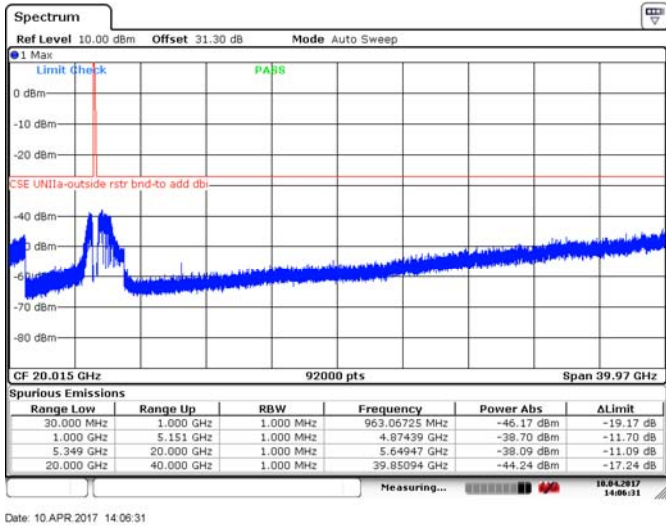
Figure 8.4-198: Spurious emissions outside restricted bands, 20 MHz channel, mid channel, 32 dBi antenna, ch1, BPSK
