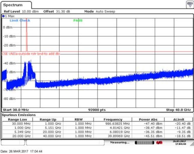
Figure 8.4-197: Spurious emissions outside restricted bands, 20 MHz channel, mid channel, 32 dBi antenna, cho, BPSK
