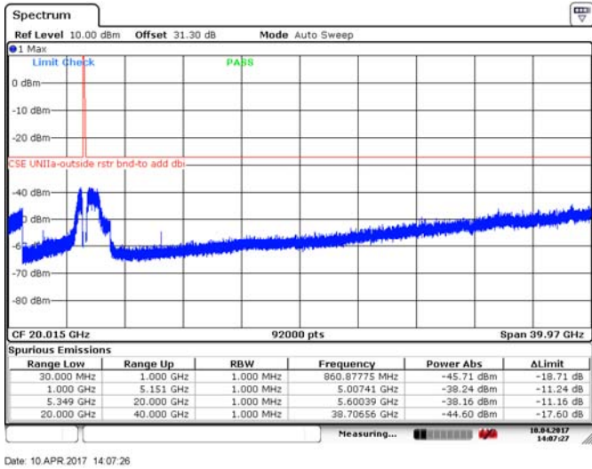
Figure 8.4-202: Spurious emissions outside restricted bands, 20 MHz channel, high channel, 32 dBi antenna, ch1, BPSK
