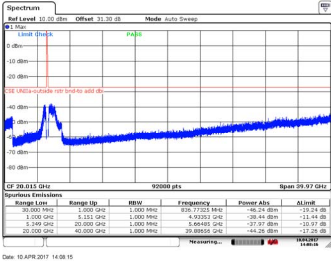
Figure 8.4-204: Spurious emissions outside restricted bands, 20 MHz channel, high channel, 32 dBi antenna, ch1, 256-QAM
