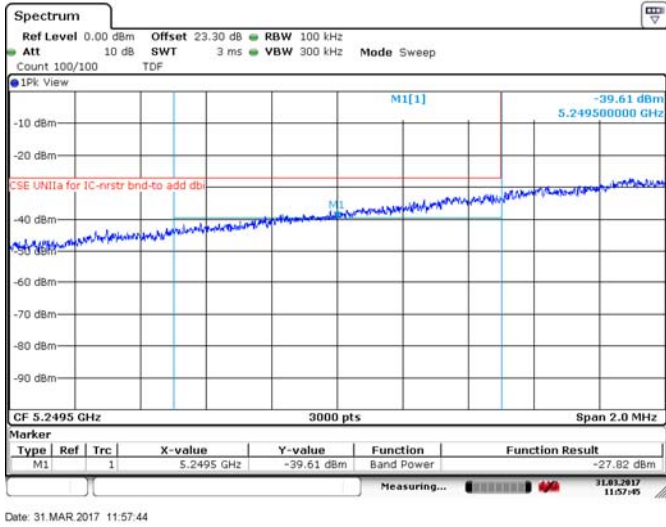
Figure 8.4-178: Lower band edge for ISED, 20 MHz channel, 24 dBi antenna, 256QAM
