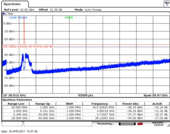
Figure 8.4-196: Spurious emissions outside restricted bands, 20 MHz channel, low channel, 32 dBi antenna, ch1, 256QAM
