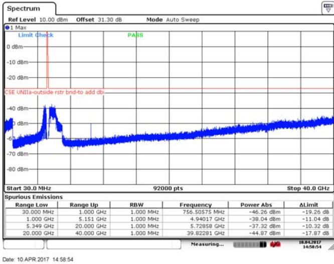
Figure 8.4-206: Spurious emissions outside restricted bands, 40 MHz channel, low channel, 32 dBi antenna, ch1, BPSK
