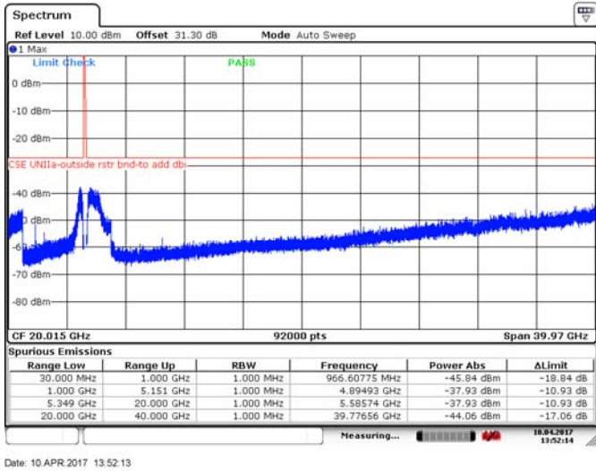
Figure 8.4-190: Spurious emissions outside restricted bands, 10 MHz channel, high channel, 32 dBi antenna, ch1, BPSK
