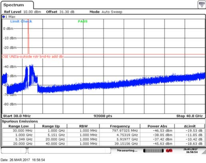
Figure 8.4-195: Spurious emissions outside restricted bands, 20 MHz channel, low channel, 32 dBi antenna, cho, 256QAM
