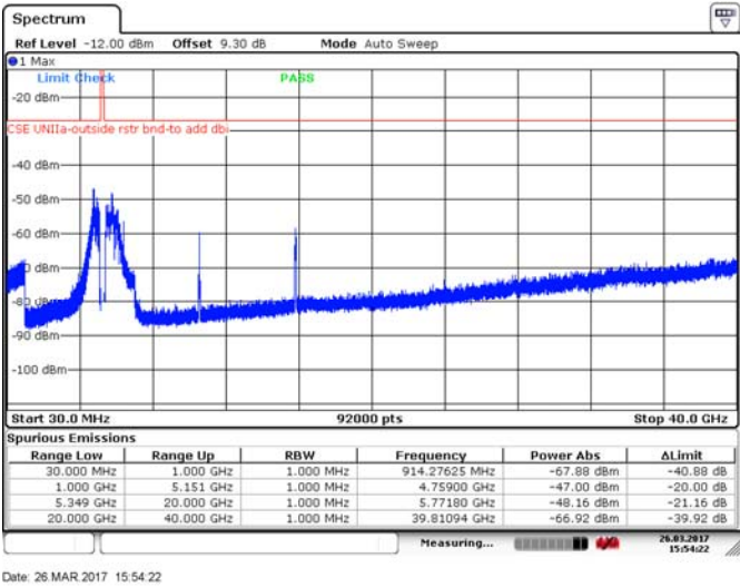
Figure 8.4-25: Spurious emissions outside restricted bands, 40 MHz channel, low channel, 10 dBi antenna, cho, 256-QAM
