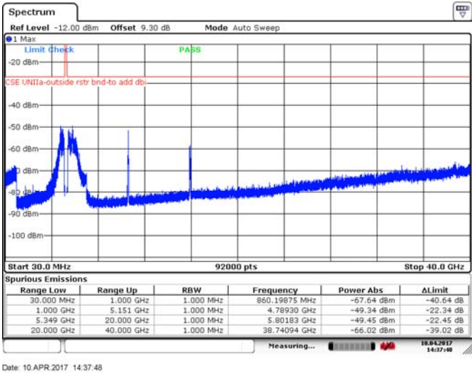
Figure 8.4-30: Spurious emissions outside restricted bands, 40 MHz channel, mid channel, 10 dBi antenna, ch1, 256-QAM
