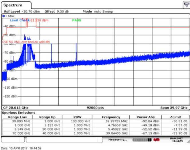
Figure 8.4-64: Spurious emissions within restricted bands, 40 MHz channel, low channel, 10 dBi antenna, ch1, 256QAM
