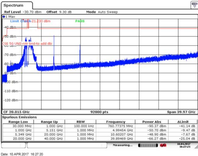
Figure 8.4-56: Spurious emissions within restricted bands, 20 MHz channel, mid channel, 10 dBi antenna, ch1, 256-QAM
