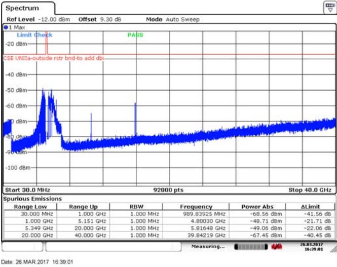
Figure 8.4-19: Spurious emissions outside restricted bands, 20 MHz channel, mid channel, 10 dBi antenna, cho, BPSK
