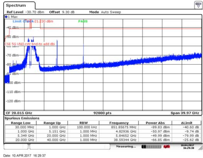
Figure 8.4-60: Spurious emissions within restricted bands, 20 MHz channel, high channel, 10 dBi antenna, ch1, 256-QAM,
