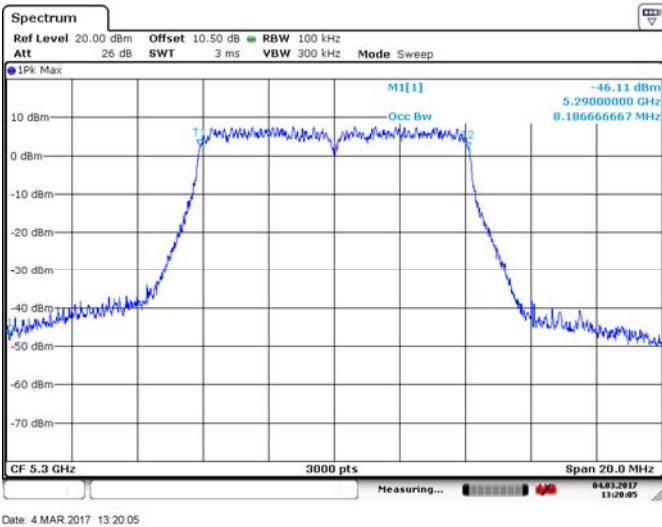
Figure 8.2-1: 99 % bandwidth of 10 MHz channel, sample plot
