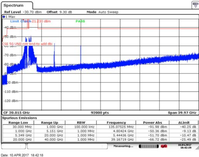
Figure 8.4-72: Spurious emissions within restricted bands, 40 MHz channel, high channel, 10 dBi antenna, ch1, 256-QAM
