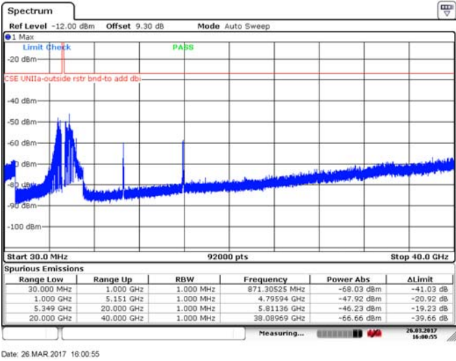
Figure 8.4-31: Spurious emissions outside restricted bands, 40 MHz channel, mid channel, 10 dBi antenna, cho, BPSK
