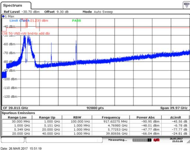
Figure 8.4-61: Spurious emissions within restricted bands, 40 MHz channel, low channel, 10 dBi antenna, cho, BPSK
