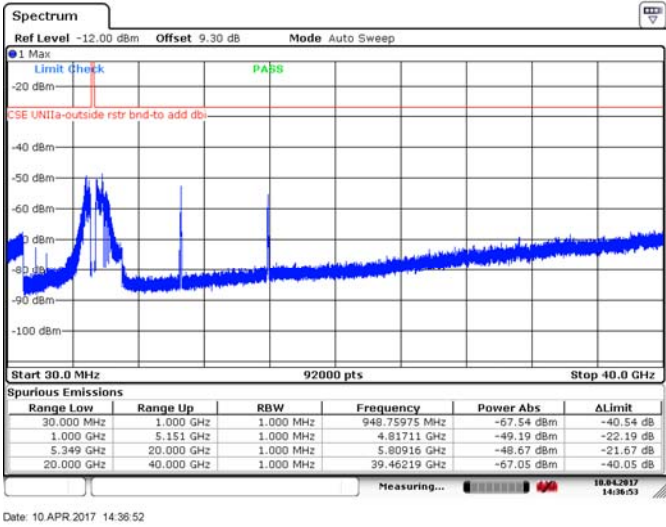
Figure 8.4-32: Spurious emissions outside restricted bands, 40 MHz channel, mid channel, 10 dBi antenna, ch1, BPSK
