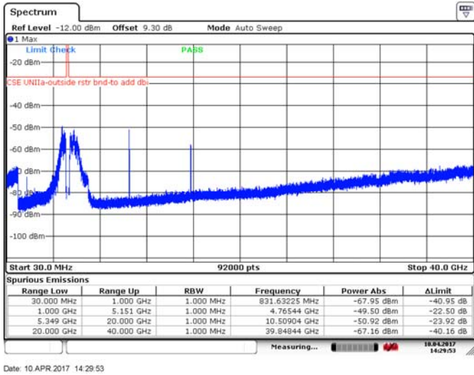
Figure 8.4-14: Spurious emissions outside restricted bands, 20 MHz channel, low channel, 10 dBi antenna, ch1, 256-QAM
