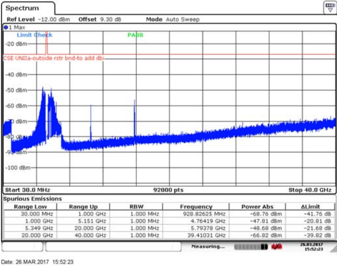
Figure 8.4-27: Spurious emissions outside restricted bands, 40 MHz channel, low channel, 10 dBi antenna, cho, BPSK
