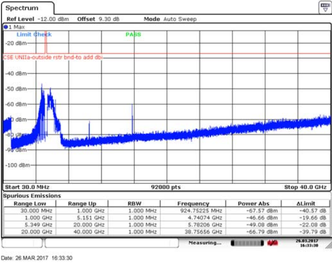
Figure 8.4-15: Spurious emissions outside restricted bands, 20 MHz channel, low channel, 10 dBi antenna, cho, BPSK
