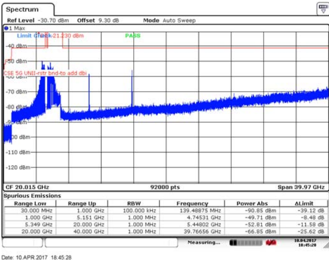
Figure 8.4-62: Spurious emissions within restricted bands, 40 MHz channel, low channel, 10 dBi antenna, ch1, BPSK
