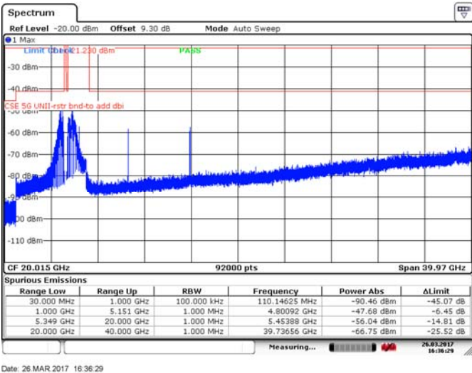
Figure 8.4-55: Spurious emissions within restricted bands, 20 MHz channel, mid channel, 10 dBi antenna, cho, 256-QAM
