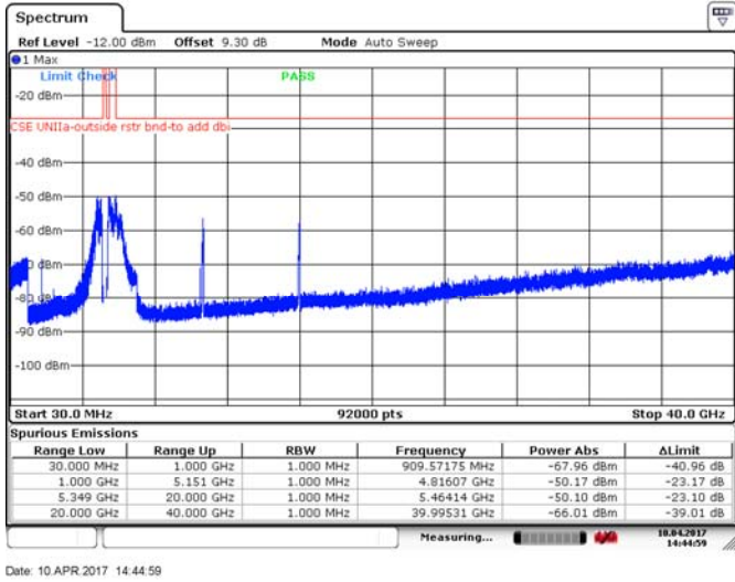
Figure 8.4-36: Spurious emissions outside restricted bands, 40 MHz channel, high channel, 10 dBi antenna, ch1, BPSK
