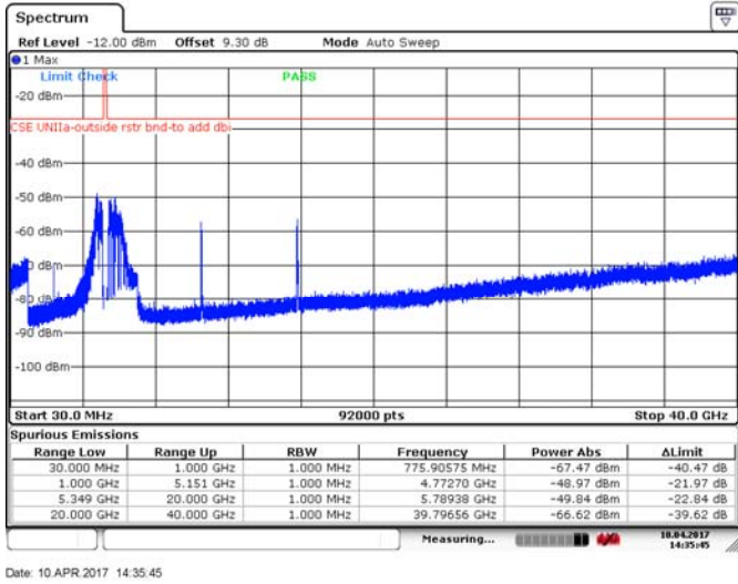
Figure 8.4-28: Spurious emissions outside restricted bands, 40 MHz channel, low channel, 10 dBi antenna, ch1, BPSK
