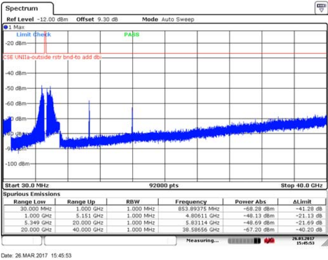
Figure 8.4-33: Spurious emissions outside restricted bands, 40 MHz channel, high channel, 10 dBi antenna, cho, 256-QAM
