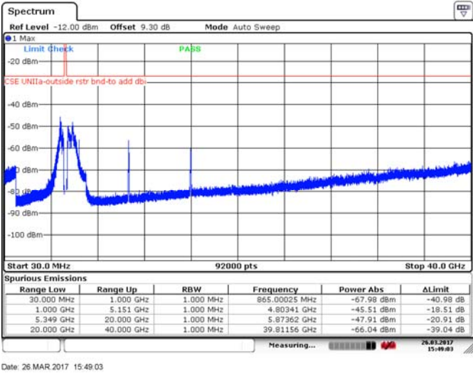
Figure 8.4-35: Spurious emissions outside restricted bands, 40 MHz channel, high channel, 10 dBi antenna, cho, BPSK
