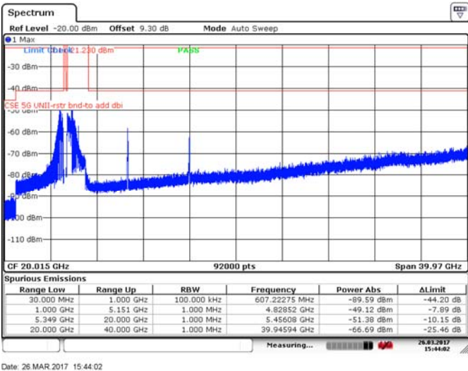
Figure 8.4-71: Spurious emissions within restricted bands, 40 MHz channel, high channel, 10 dBi antenna, cho, 256-QAM
