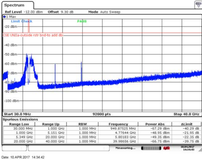
Figure 8.4-26: Spurious emissions outside restricted bands, 40 MHz channel, low channel, 10 dBi antenna, ch1, 256-QAM
