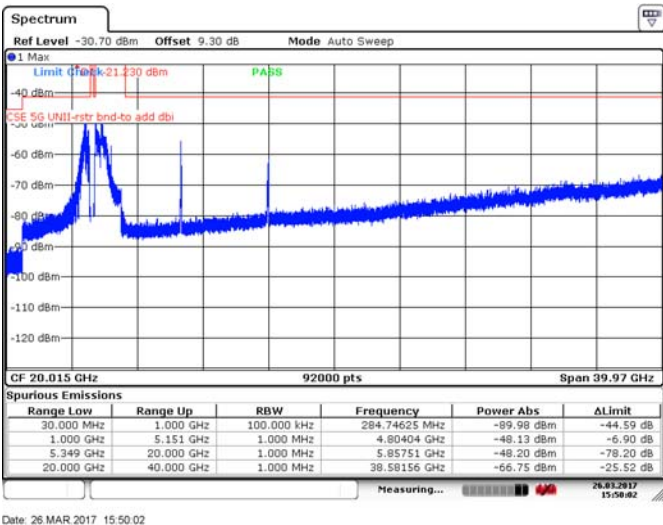
Figure 8.4-69: Spurious emissions within restricted bands, 40 MHz channel, high channel, 10 dBi antenna, cho, BPSK
