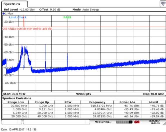
Figure 8.4-20: Spurious emissions outside restricted bands, 20 MHz channel, mid channel, 10 dBi antenna, ch1, BPSK
