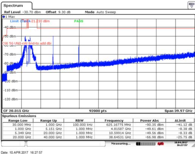
Figure 8.4-54: Spurious emissions within restricted bands, 20 MHz channel, mid channel, 10 dBi antenna, ch1, BPSK
