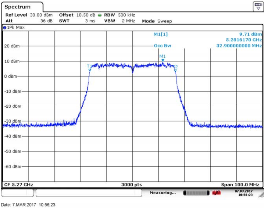
Figure 8.2-3: 99 % bandwidth of 40 MHz channel, sample plot
