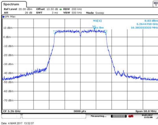
Figure 8.2-2: 99 % bandwidth of 20 MHz channel, sample plot
