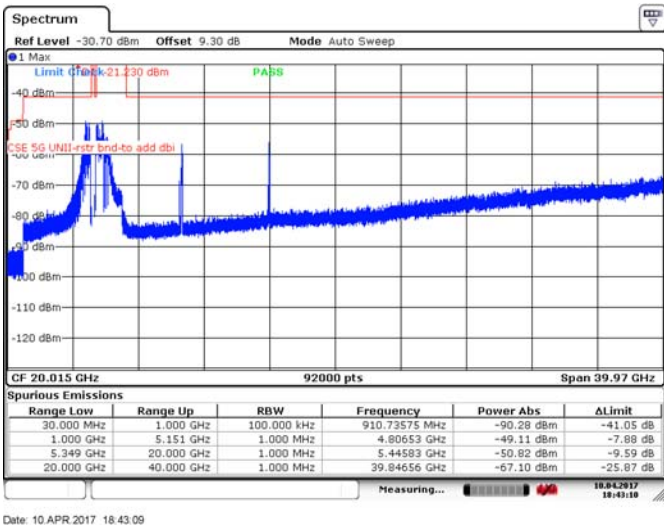
Figure 8.4-70: Spurious emissions within restricted bands, 40 MHz channel, high channel, 10 dBi antenna, ch1, BPSK
