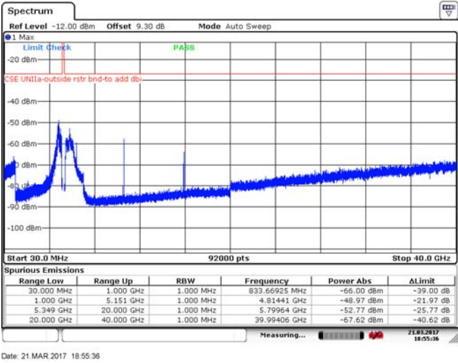
Figure 8.4-7: Spurious emissions outside restricted bands, 10 MHz channel, mid channel, 10 dBi antenna, cho, BPSK
