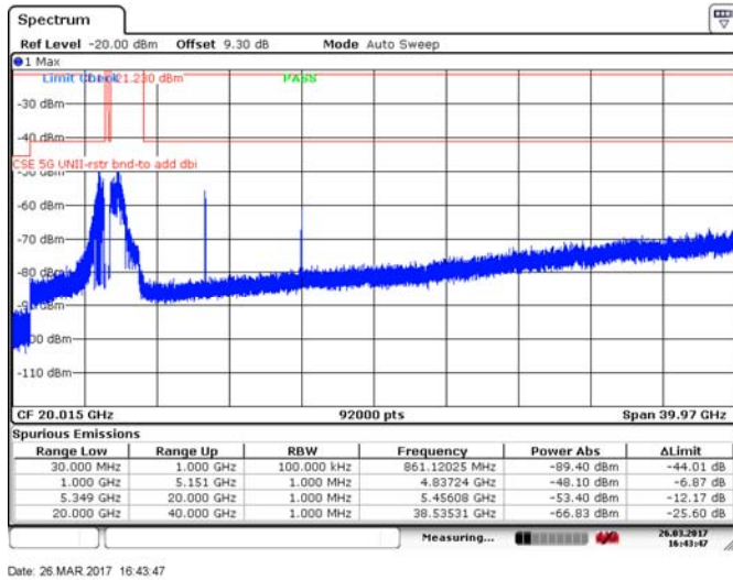
Figure 8.4-59: Spurious emissions within restricted bands, 20 MHz channel, high channel, 10 dBi antenna, cho, 256-QAM,
