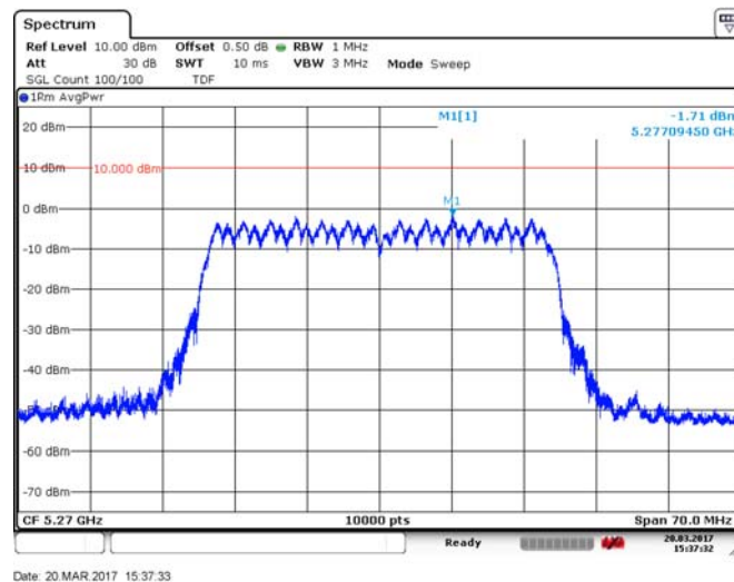
Figure 8.3-3: Sample plot for PSD on 40 MHz channel
