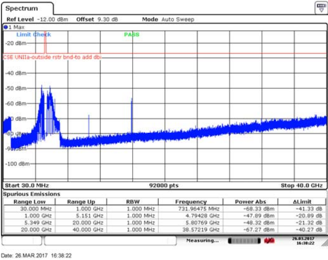
Figure 8.4-17: Spurious emissions outside restricted bands, 20 MHz channel, mid channel, 10 dBi antenna, cho, 256-QAM
