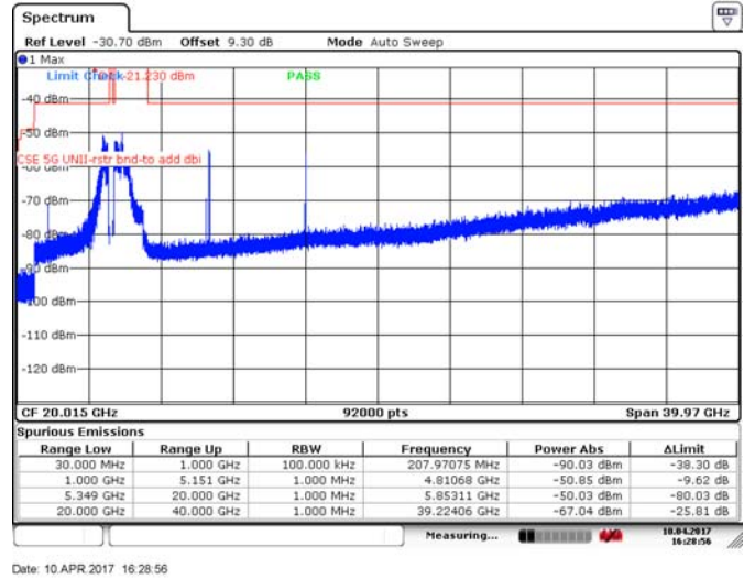
Figure 8.4-58: Spurious emissions within restricted bands, 20 MHz channel, high channel, 10 dBi antenna, ch1, BPSK
