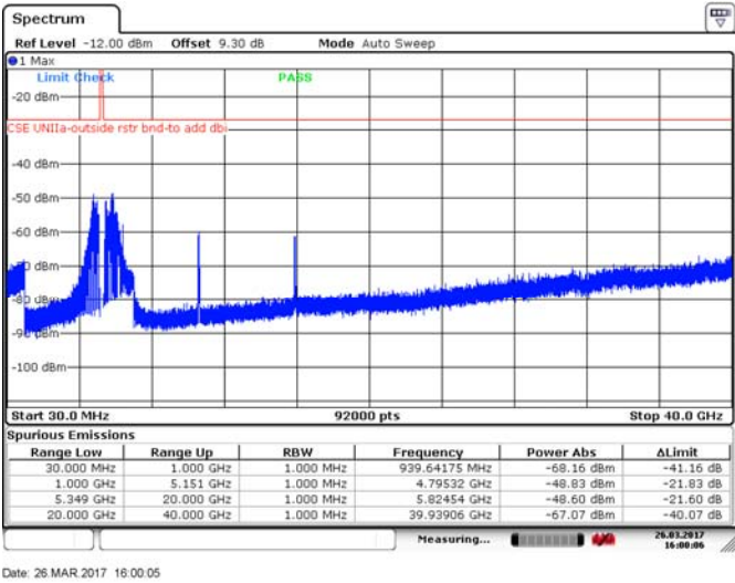
Figure 8.4-29: Spurious emissions outside restricted bands, 40 MHz channel, mid channel, 10 dBi antenna, cho, 256-QAM
