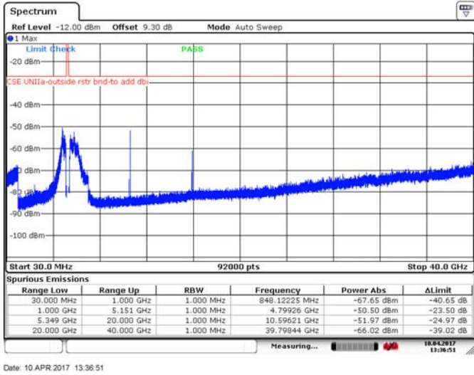
Figure 8.4-8: Spurious emissions outside restricted bands, 10 MHz channel, mid channel, 10 dBi antenna, ch1, BPSK
