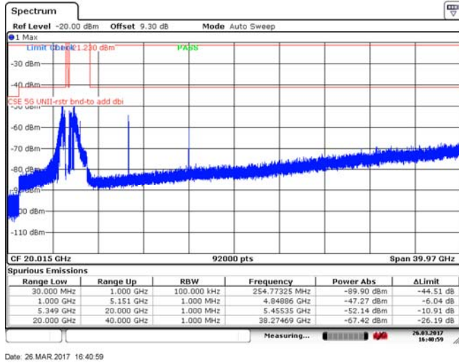
Figure 8.4-57: Spurious emissions within restricted bands, 20 MHz channel, high channel, 10 dBi antenna, cho, BPSK
