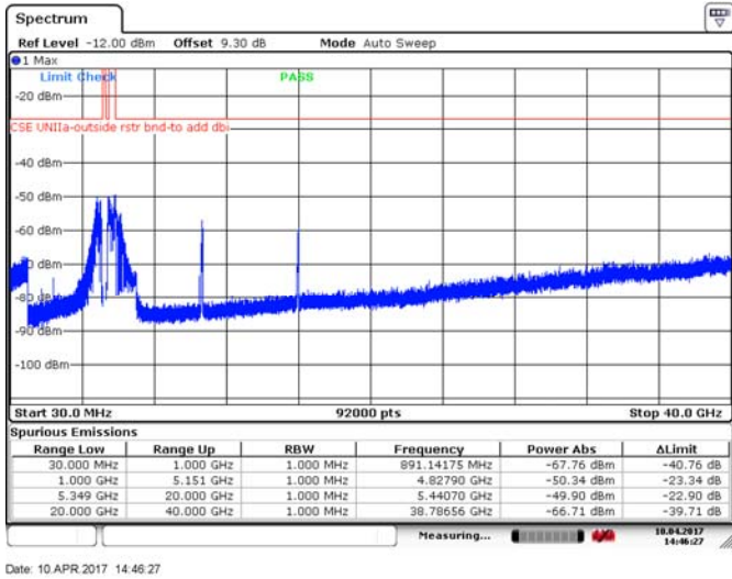
Figure 8.4-34: Spurious emissions outside restricted bands, 40 MHz channel, high channel, 10 dBi antenna, ch1, 256-QAM
