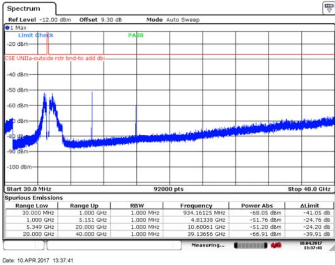
Figure 8.4-18: Spurious emissions outside restricted bands, 20 MHz channel, mid channel, 10 dBi antenna, ch1, 256-QAM
