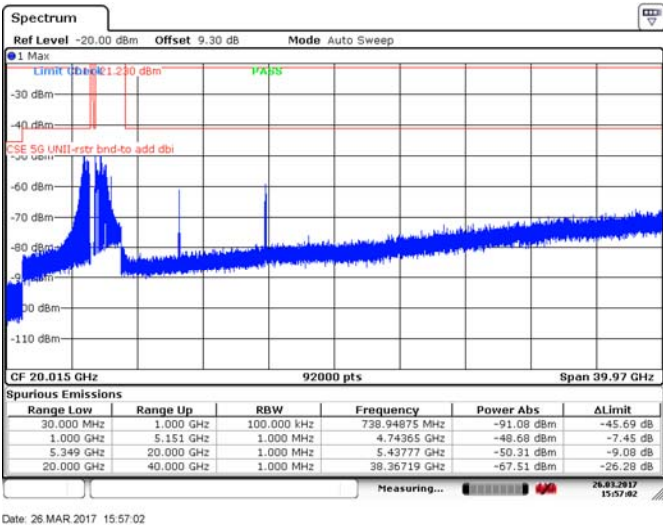
Figure 8.4-63: Spurious emissions within restricted bands, 40 MHz channel, low channel, 10 dBi antenna, cho, 256QAM
