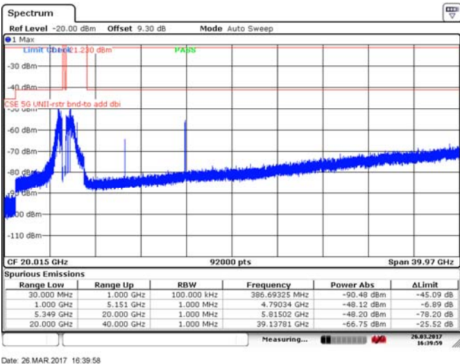
Figure 8.4-53: Spurious emissions within restricted bands, 20 MHz channel, mid channel, 10 dBi antenna, cho, BPSK
