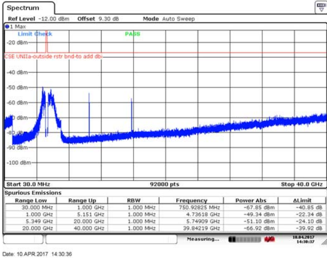
Figure 8.4-16: Spurious emissions outside restricted bands, 20 MHz channel, low channel, 10 dBi antenna, ch1, BPSK
