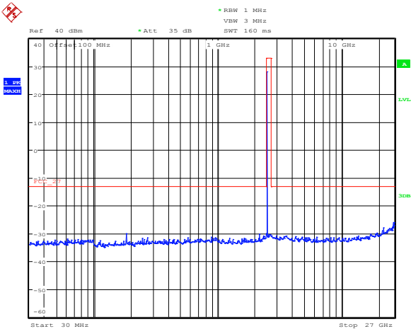
Figure 8.2-7: Conducted spurious emissions at antenna port 1, high channel, 1.25 MHz BW, 256-QAM
