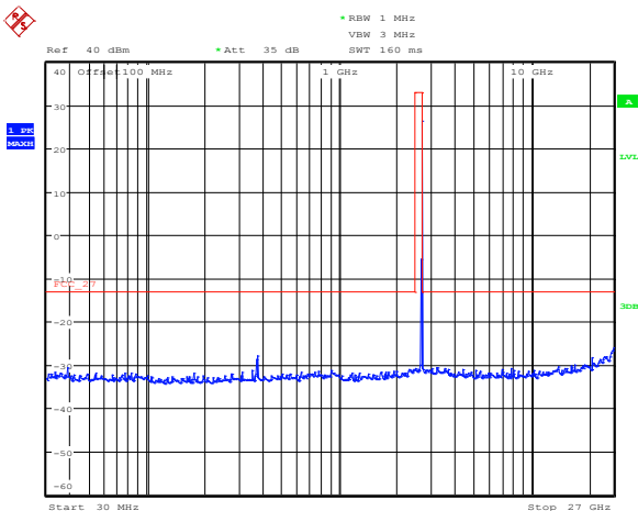
Figure 8.2-12: Conducted spurious emissions at antenna port 2, low channel, 2.5 MHz BW, 256-QAM
