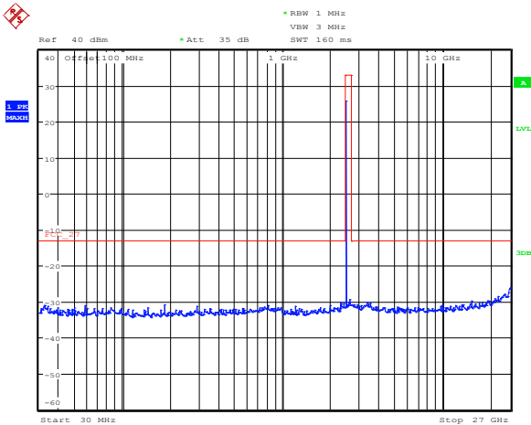
Figure 8.2-8: Conducted spurious emissions at antenna port 2, high channel, 1.25 MHz BW, 256-QAM
