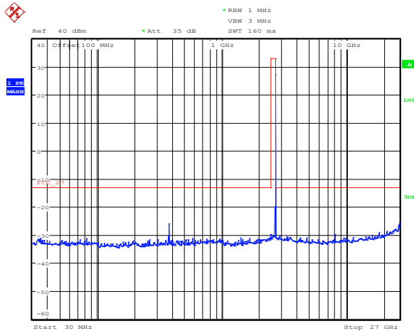
Figure 8.2-4: Conducted spurious emissions at antenna port 2, low channel, 1.25 MHz BW, 256-QAM
