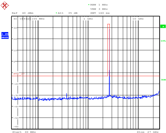
Figure 8.2-11: Conducted spurious emissions at antenna port 1, low channel, 2.5 MHz BW, 256-QAM
