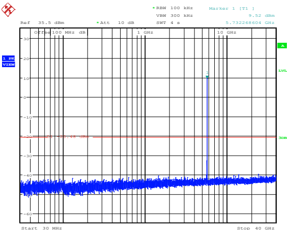
Plot 8.4-34: Conducted spurious emissions at the antenna port 2, 5 MHz channel, low frequency, 10 dBi antenna settings
