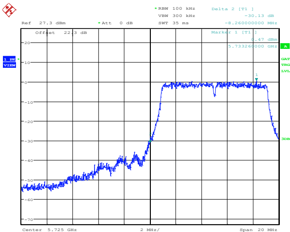
Plot 8.4-25: Conducted lower band edge at the antenna port 2, 5 MHz channel, 19 dBi antenna settings
