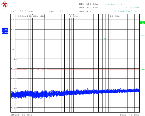
Plot 8.4-37: Conducted spurious emissions at the antenna port 1, 5 MHz channel, mid frequency, 10 dBi antenna settings
