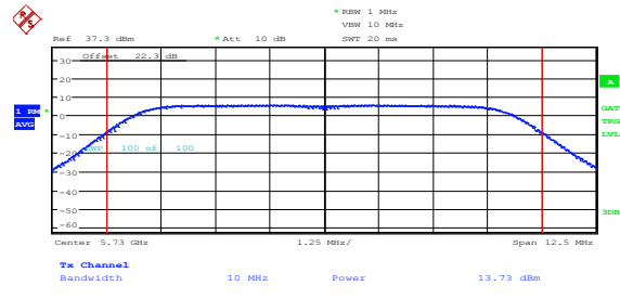
Plot 8.3-2: Peak output power on mid channel
