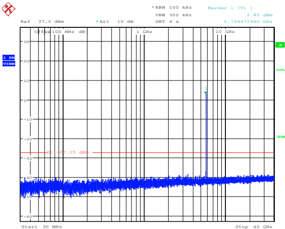
Plot 8.4-6: Conducted spurious emissions at the antenna port 2, 20 MHz channel, low frequency, 19 dBi antenna settings
