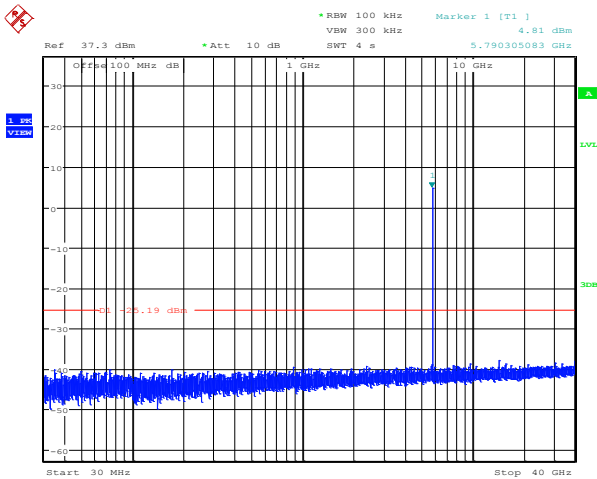
Plot 8.4-5: Conducted spurious emissions at the antenna port 2, 10 MHz channel, low frequency, 19 dBi antenna settings
