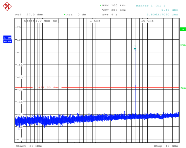
Plot 8.4-13: Conducted spurious emissions at the antenna port 1, 5 MHz channel, high frequency, 19 dBi antenna settings
