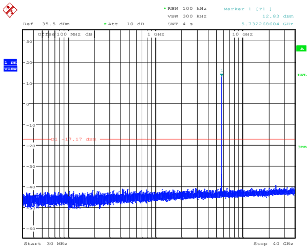
Plot 8.4-33: Conducted spurious emissions at the antenna port 1, 20 MHz channel, low frequency, 10 dBi antenna settings
