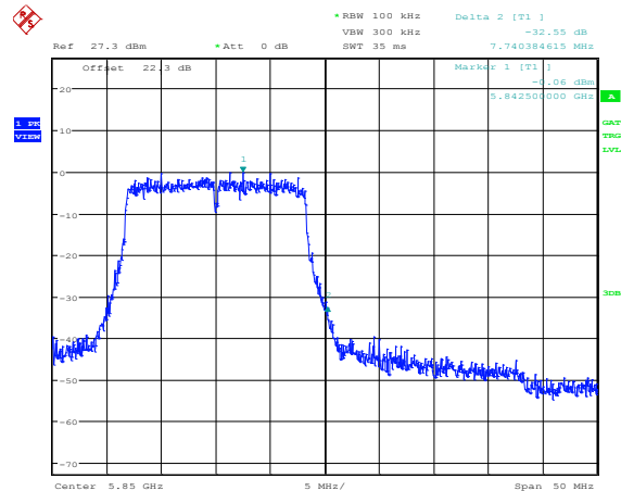
Plot 8.4-22: Conducted upper band edge at the antenna port 1, 10 MHz channel, 19 dBi antenna settings
