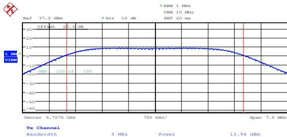
Plot 8.3-1: Peak output power on low channel
