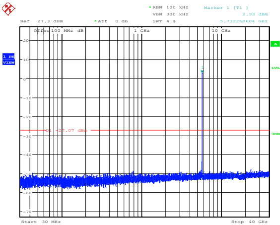
Plot 8.4-2: Conducted spurious emissions at the antenna port 1, 10 MHz channel, low frequency, 19 dBi antenna settings
