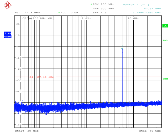
Plot 8.4-10: Conducted spurious emissions at the antenna port 2, 5 MHz channel, mid frequency, 19 dBi antenna settings
