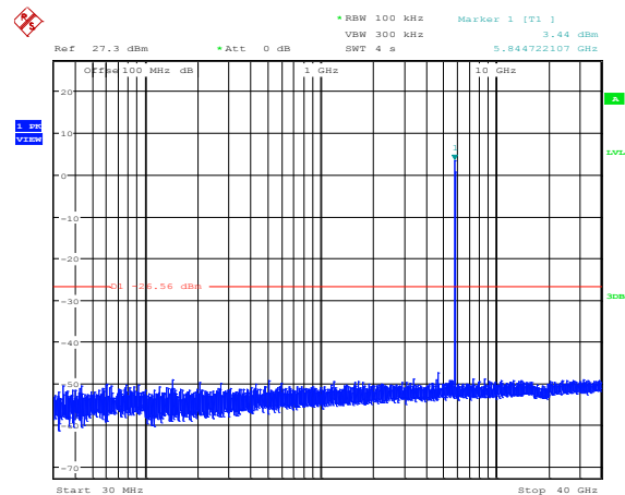
Plot 8.4-14: Conducted spurious emissions at the antenna port 1, 10 MHz channel, high frequency, 19 dBi antenna settings
