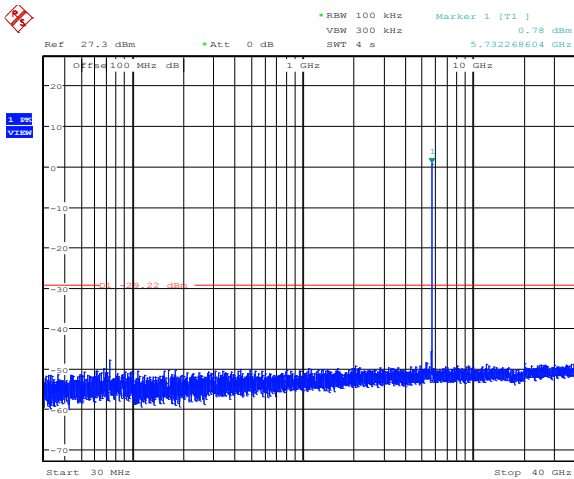
Plot 8.4-1: Conducted spurious emissions at the antenna port 1, 5 MHz channel, low frequency, 19 dBi antenna settings
