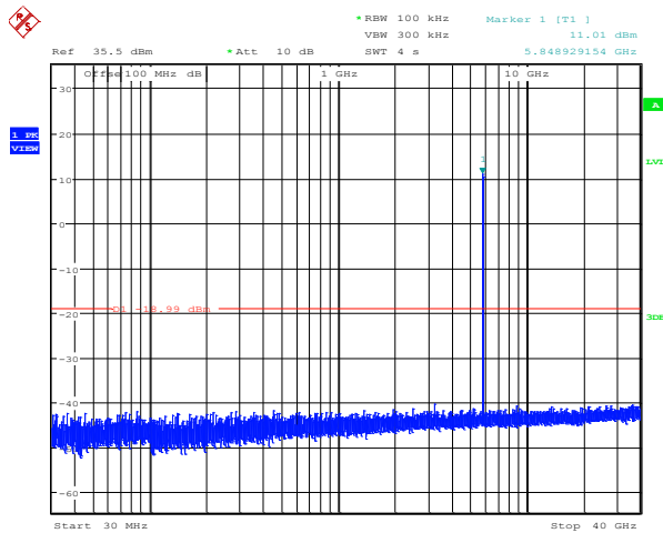
Plot 8.4-41: Conducted spurious emissions at the antenna port 2, 10 MHz channel, mid frequency, 10 dBi antenna settings
