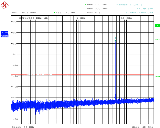
Plot 8.4-38: Conducted spurious emissions at the antenna port 1, 10 MHz channel, mid frequency, 10 dBi antenna settings
