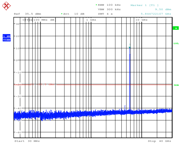
Plot 8.4-45: Conducted spurious emissions at the antenna port 1, 20 MHz channel, high frequency, 10 dBi antenna settings
