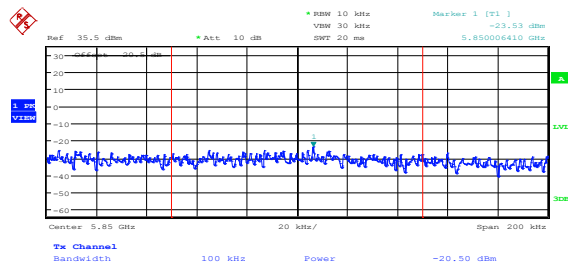
Plot 8.4-62: Conducted lower band edge at the antenna port 2, 10 MHz channel, 10 dBi antenna settings
