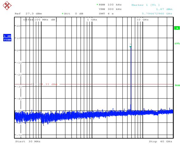
Plot 8.4-9: Conducted spurious emissions at the antenna port 1, 20 MHz channel, mid frequency, 19 dBi antenna settings
