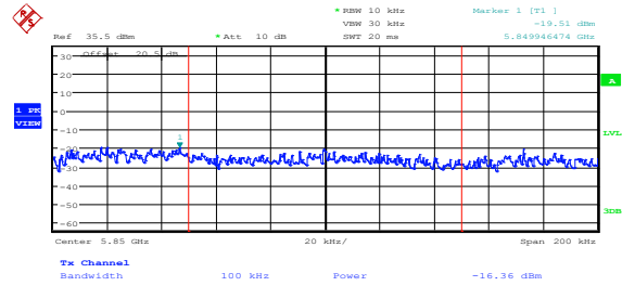
Plot 8.4-50: Conducted lower band edge at the antenna port 1, 5 MHz channel, 10 dBi antenna settings
