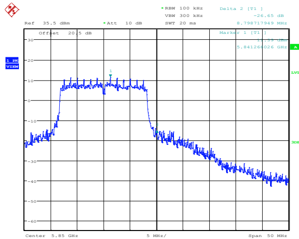
Plot 8.4-65: Conducted lower band edge (in-band) at the antenna port 1, 20 MHz channel, 10 dBi antenna settings
