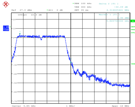
Plot 8.4-18: Conducted spurious emissions at the antenna port 2, 20 MHz channel, high frequency, 19 dBi antenna settings
