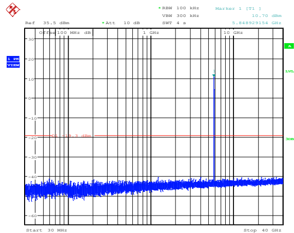
Plot 8.4-42: Conducted spurious emissions at the antenna port 2, 20 MHz channel, mid frequency, 10 dBi antenna settings
