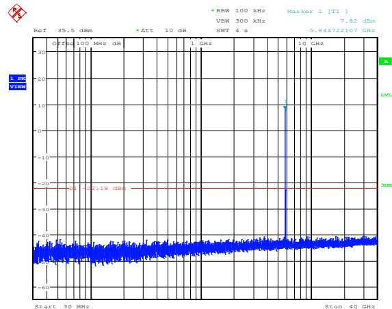
Plot 8.4-46: Conducted spurious emissions at the antenna port 2, 5 MHz channel, high frequency, 10 dBi antenna settings
