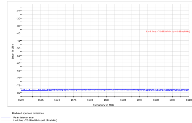
Figure 8.5-1: Field strength within 1559–1610 MHz band for 5 MHz low channel
