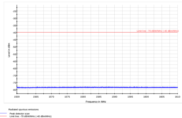
Figure 8.5-4: Field strength within 1559–1610 MHz band for 10 MHz channel
