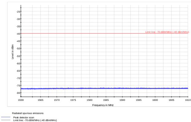
Figure 8.5-3: Field strength within 1559–1610 MHz band for 5 MHz high channel
