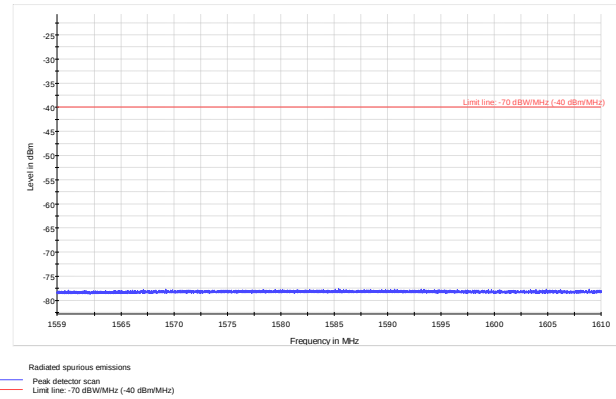
Figure 8.5-2: Field strength within 1559–1610 MHz band for 5 MHz mid channel
