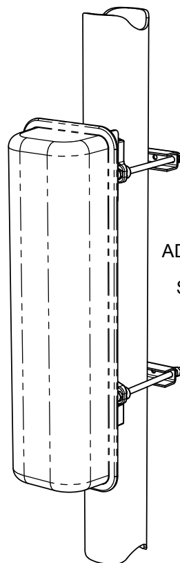
PICTORIAL VIEW
