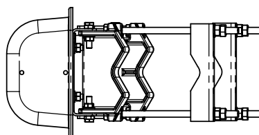
END VIEW
