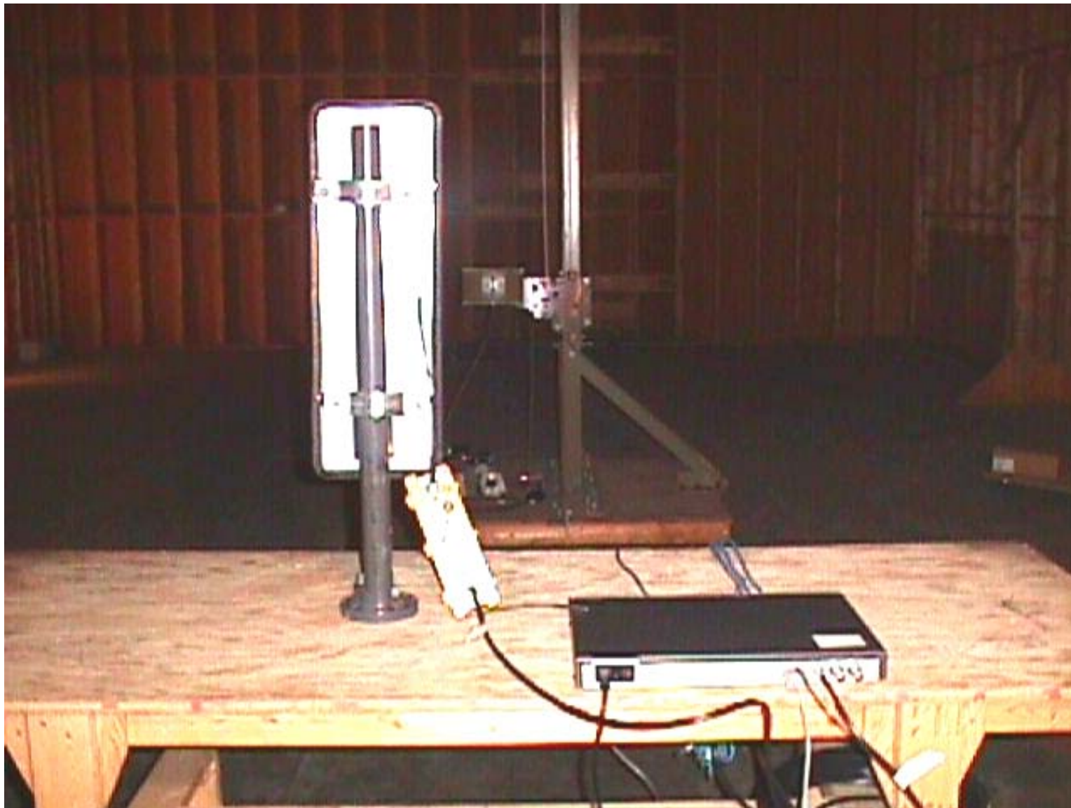
Photo #4: Radiated Emissions Measurements at 3m Distance Radiowave Antenna Model SEC-55V-60-17, Gain: 17 dBi (maximum gain within its family)
