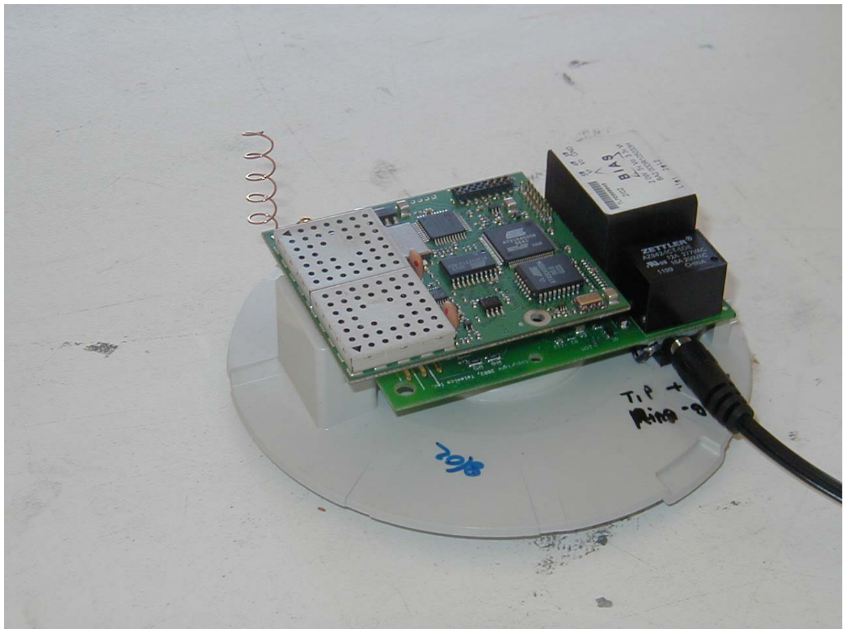
Close-up of module showing helical antenna
