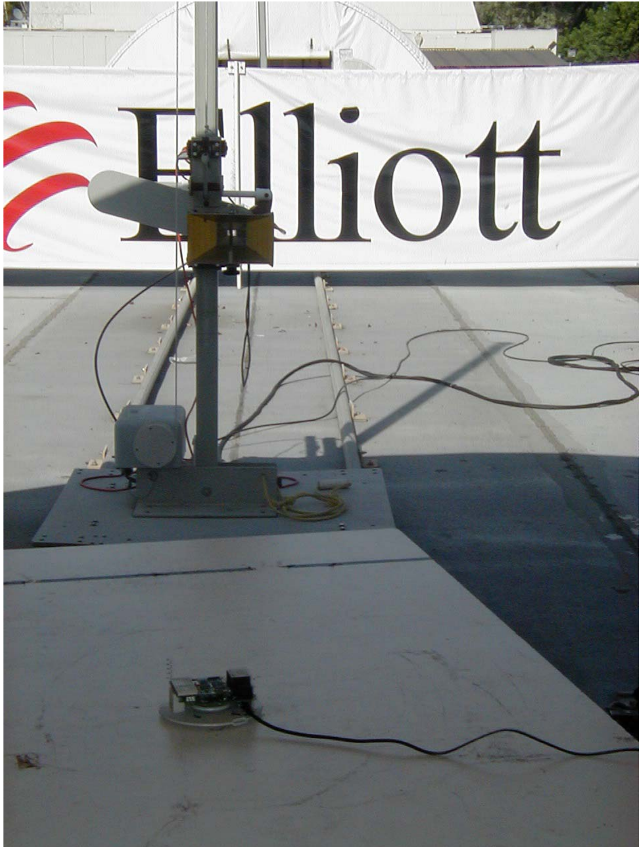
Radiated Emissions in Restricted bands with “helical” antenna
