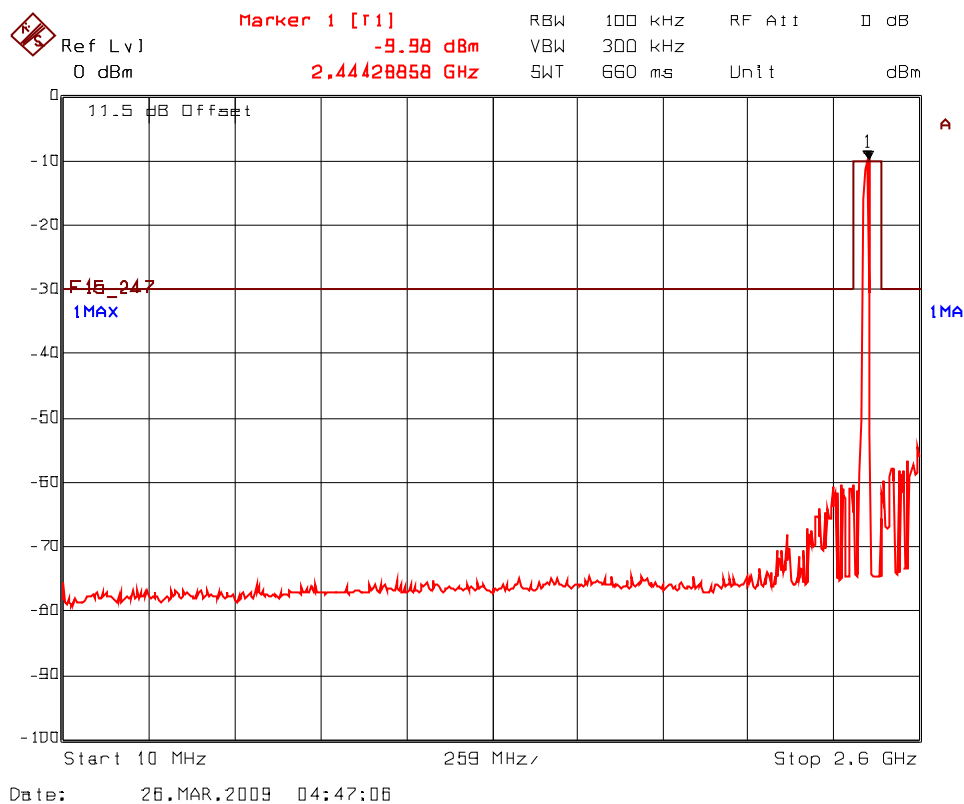
Plot 5.7.4.2.5(i) Spurious RF Conducted Emissions, 802.11g Mode Transmitter Frequency: 2437 MHz
