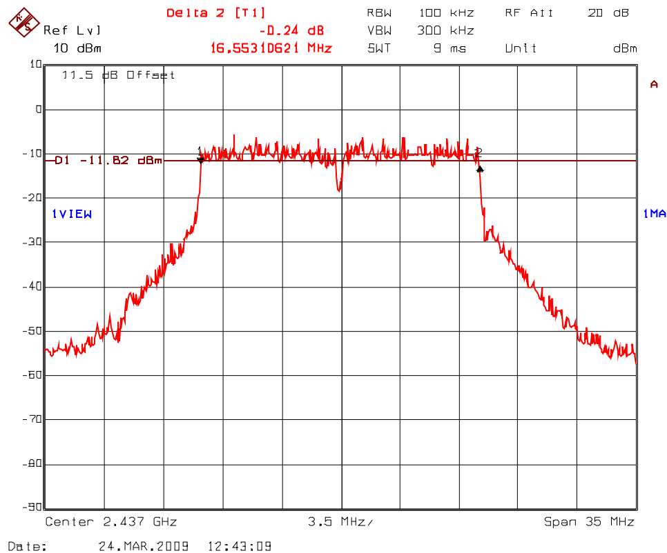
Plot 5.5.4.14. 6 dB Bandwidth Frequency: 2437 MHz; Modulation: QPSK at 18 Mbps
