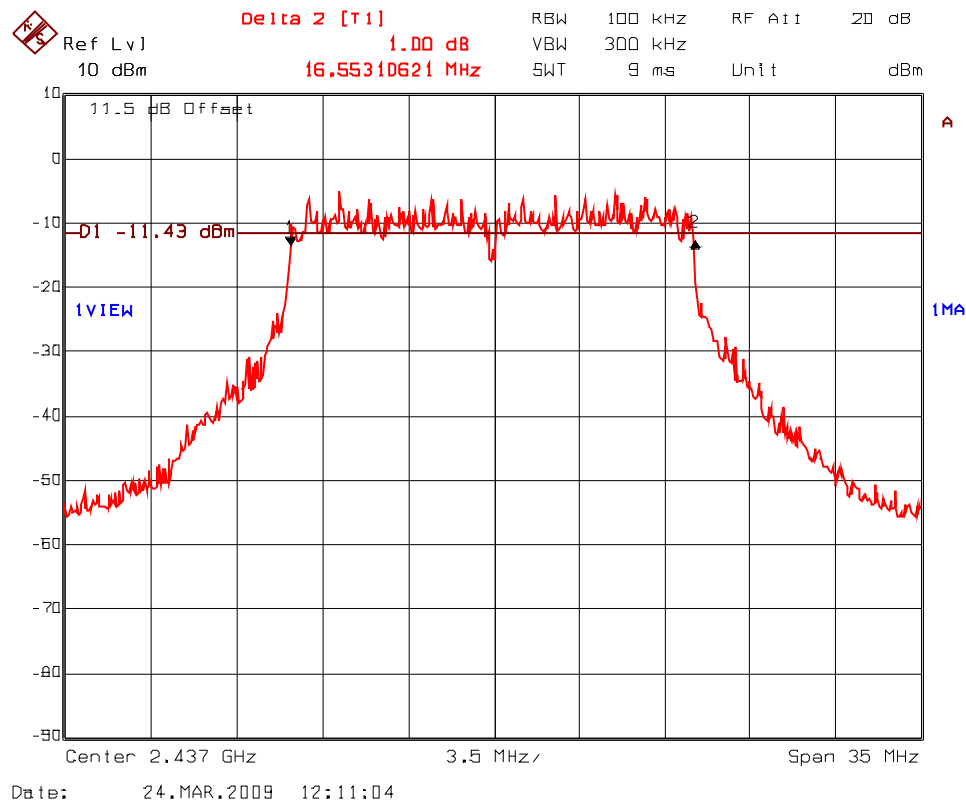
Plot 5.5.4.11. 6 dB Bandwidth Frequency: 2437 MHz; Modulation: BPSK at 9 Mbps
