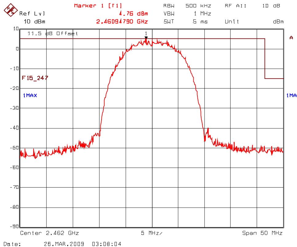
Plot 5.7.4.1.2. Band-Edge RF Conducted Emissions, 802.11b Mode High End of Frequency Band 2412 -2462 MHz
