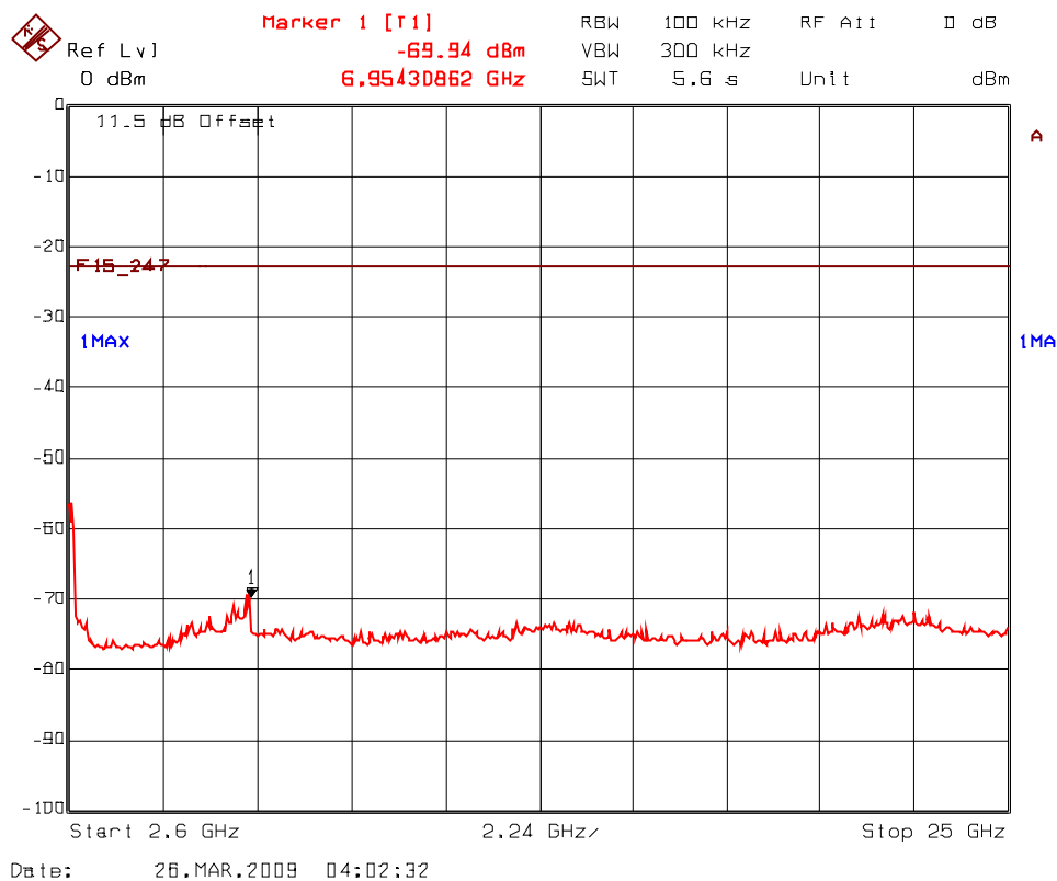
Plot 5.7.4.2.1(ii) Spurious RF Conducted Emissions, 802.11b Mode Transmitter Frequency: 2412 MHz
