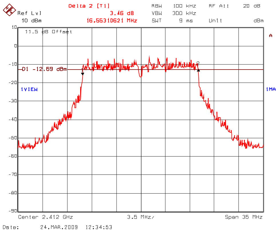
Plot 5.5.4.13. 6 dB Bandwidth Frequency: 2412 MHz; Modulation: QPSK at 18 Mbps
