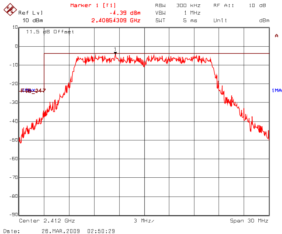
Plot 5.7.4.1.3. Band-Edge RF Conducted Emissions, 802.11g Mode Low End of Frequency Band 2412 -2462 MHz
