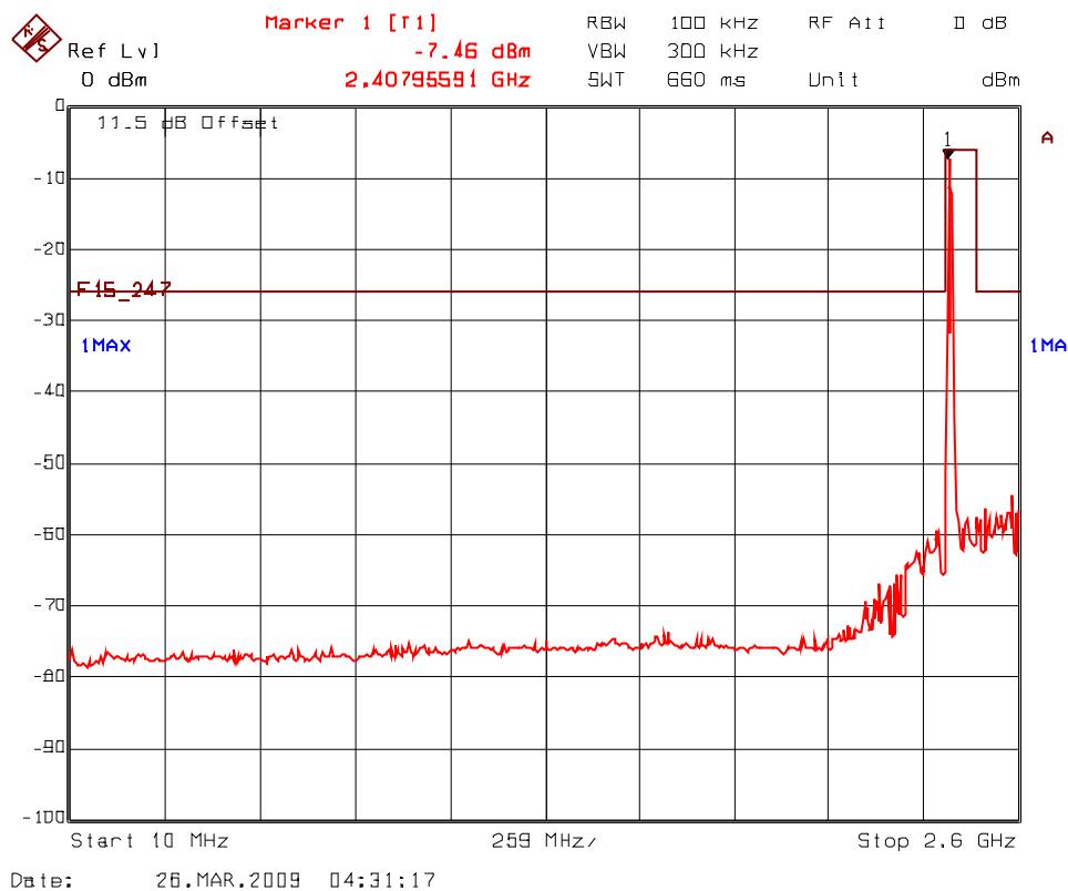
Plot 5.7.4.2.4(i) Spurious RF Conducted Emissions, 802.11g Mode Transmitter Frequency: 2412 MHz
