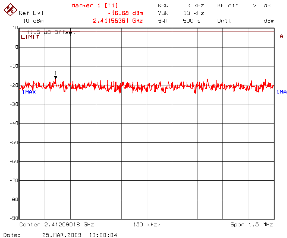
Plot 5.9.4.1. Power Spectral Density Frequency: 2412 MHz
