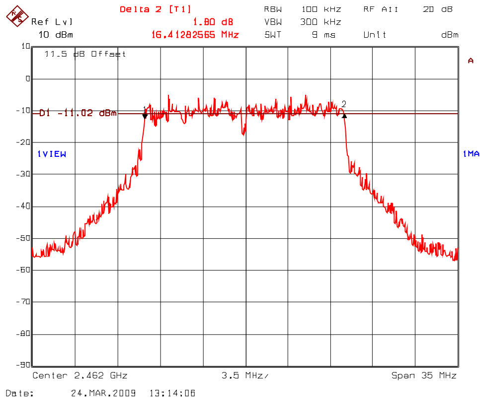
Plot 5.5.4.18. 6 dB Bandwidth Frequency: 2462 MHz; Modulation: 16QAM at 36 Mbps
