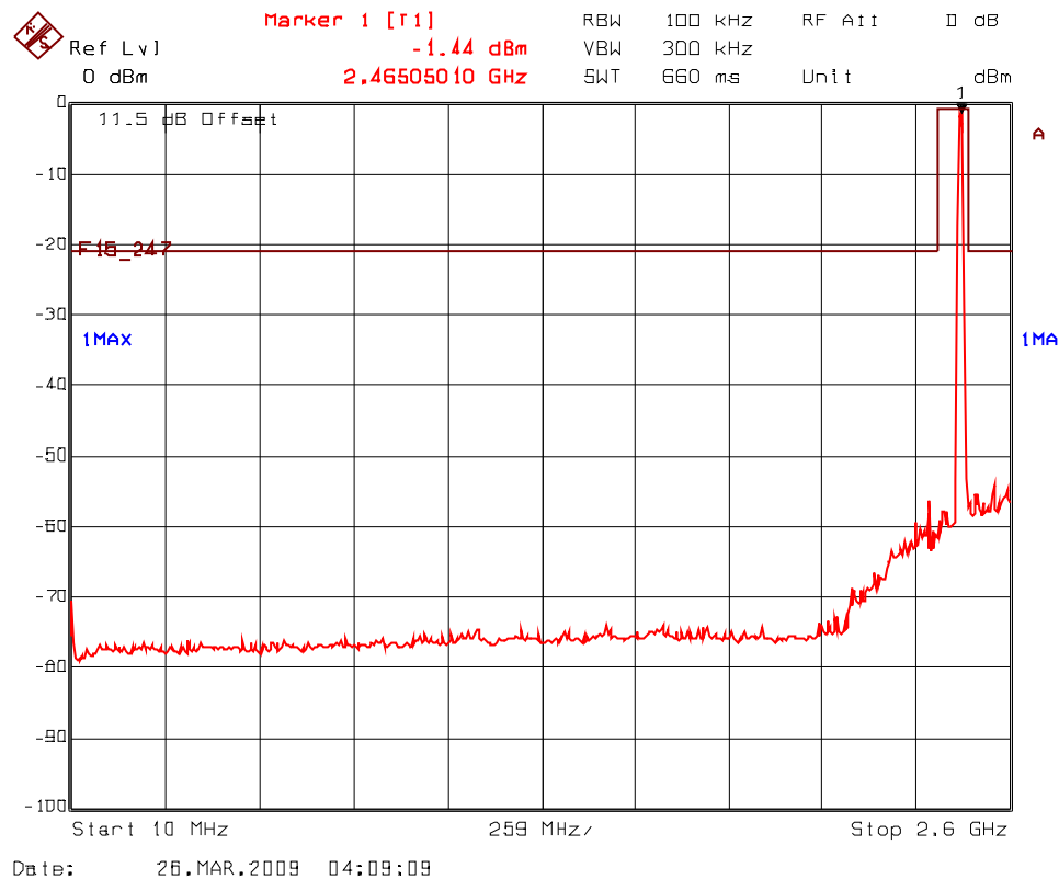
Plot 5.7.4.2.3(i) Spurious RF Conducted Emissions, 802.11b Mode Transmitter Frequency: 2462 MHz
