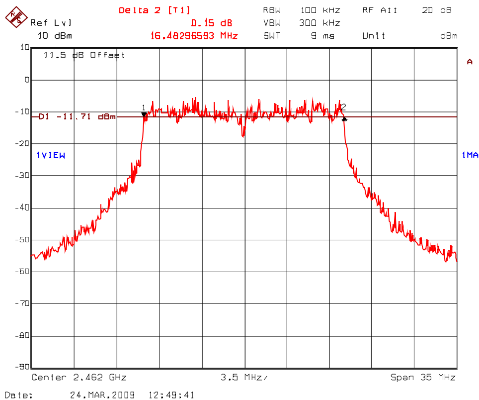
Plot 5.5.4.15. 6 dB Bandwidth Frequency: 2462 MHz; Modulation: QPSK at 18 Mbps
