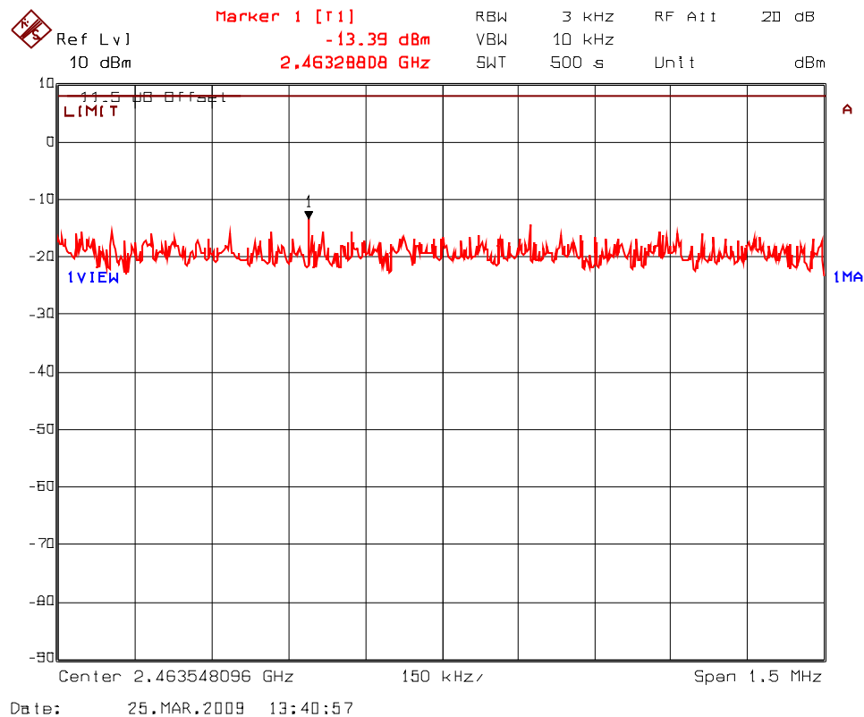
Plot 5.9.4.3. Power Spectral Density Frequency: 2462 MHz
