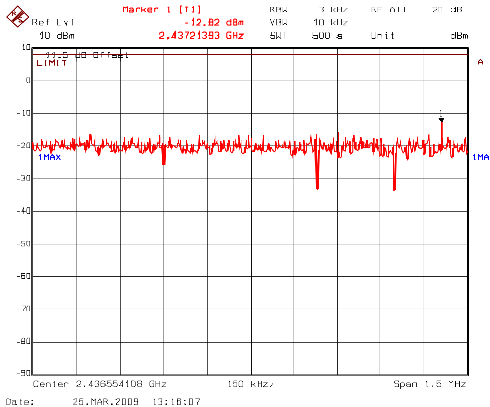
Plot 5.9.4.2. Power Spectral Density Frequency: 2437 MHz
