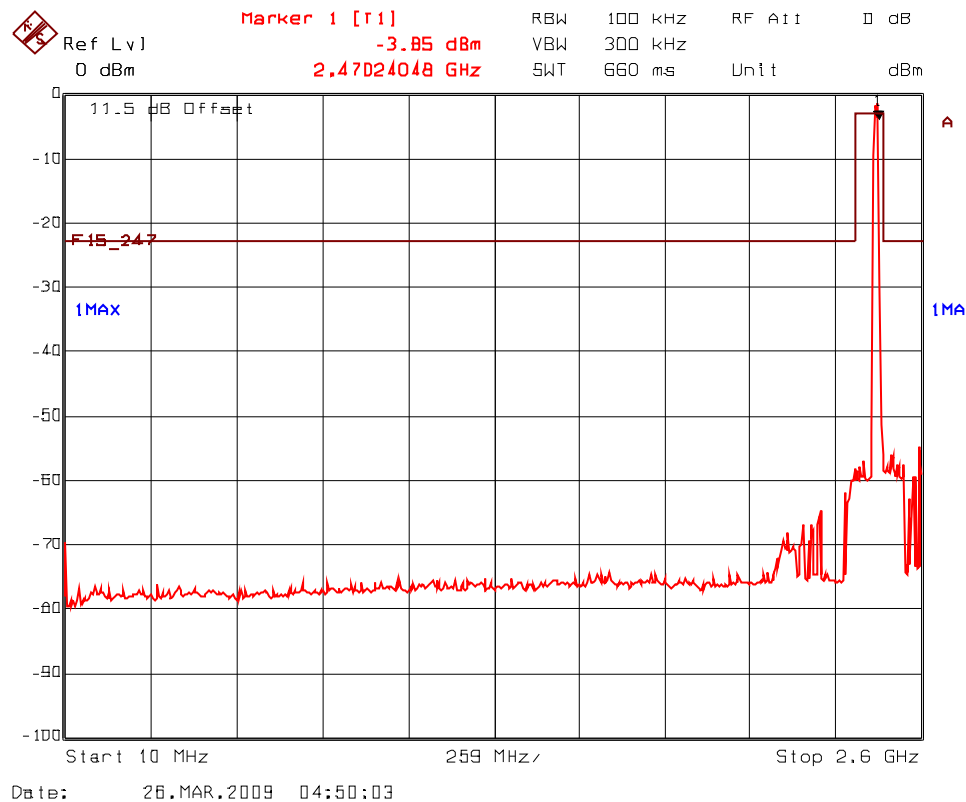
Plot 5.7.4.2.6(i) Spurious RF Conducted Emissions, 802.11g Mode Transmitter Frequency: 2462 MHz
