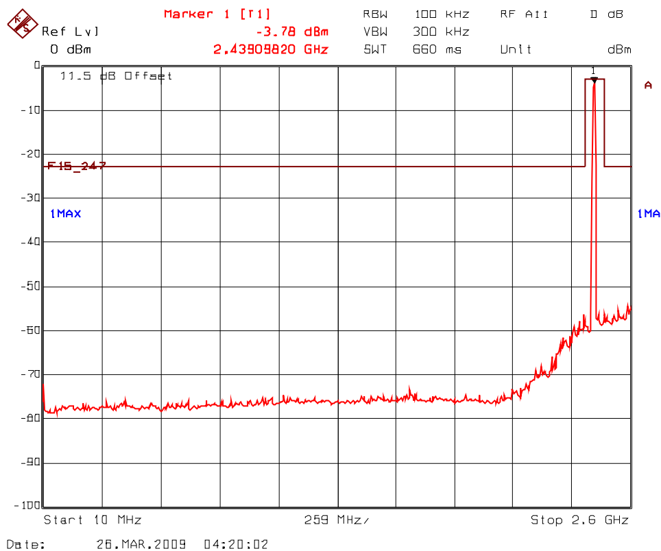
Plot 5.7.4.2.2(i) Spurious RF Conducted Emissions, 802.11b Mode Transmitter Frequency: 2437 MHz
