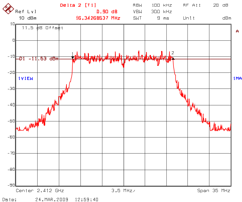
Plot 5.5.4.16. 6 dB Bandwidth Frequency: 2412 MHz; Modulation: 16QAM at 36 Mbps
