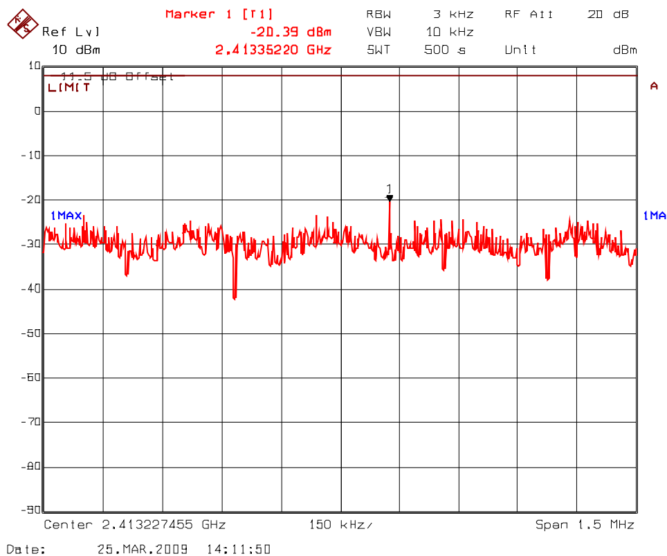
Plot 5.9.4.4. Power Spectral Density Frequency: 2412 MHz
