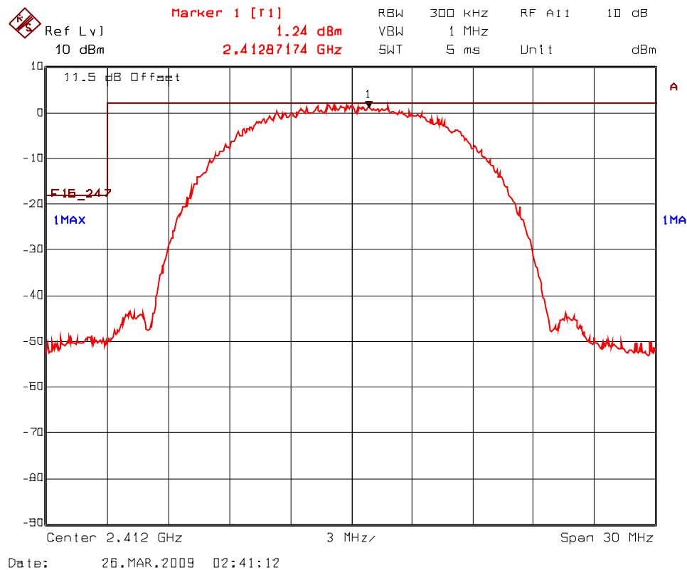
Plot 5.7.4.1.1. Band-Edge RF Conducted Emissions, 802.11b Mode Low End of Frequency Band 2412 -2462 MHz
