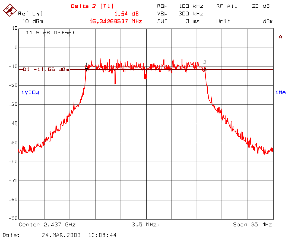
Plot 5.5.4.17. 6 dB Bandwidth Frequency: 2437 MHz; Modulation: 16QAM at 36 Mbps
