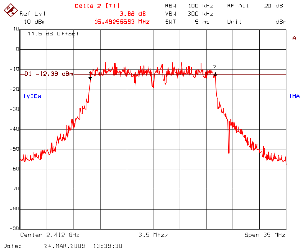
Plot 5.5.4.19. 6 dB Bandwidth Frequency: 2412 MHz; Modulation: 64QAM at 54 Mbps
