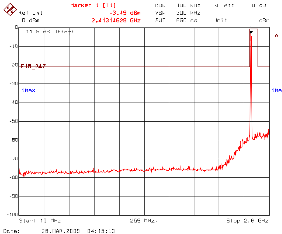
Plot 5.7.4.2.1(i) Spurious RF Conducted Emissions, 802.11b Mode Transmitter Frequency: 2412 MHz
