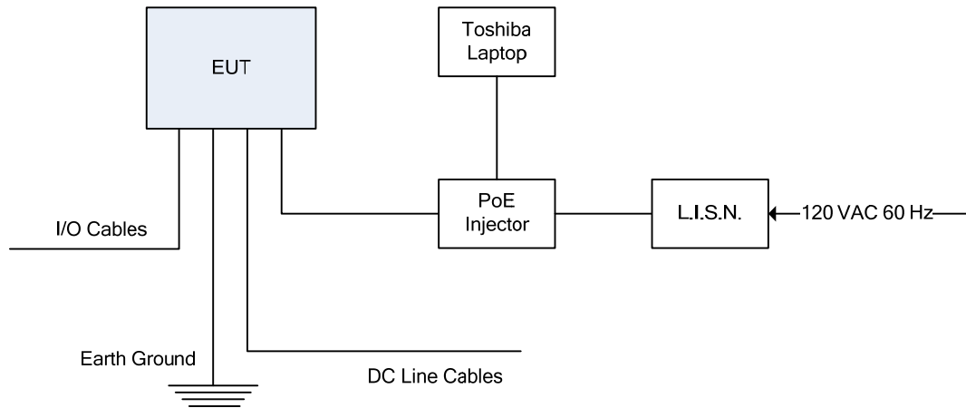
Test Configuration 2: Power Over Ethernet (PoE) Injector
