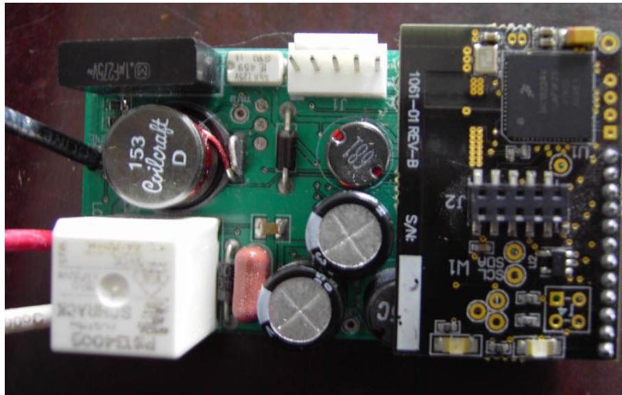
Figure 5 PCB of the EUT-Front View
