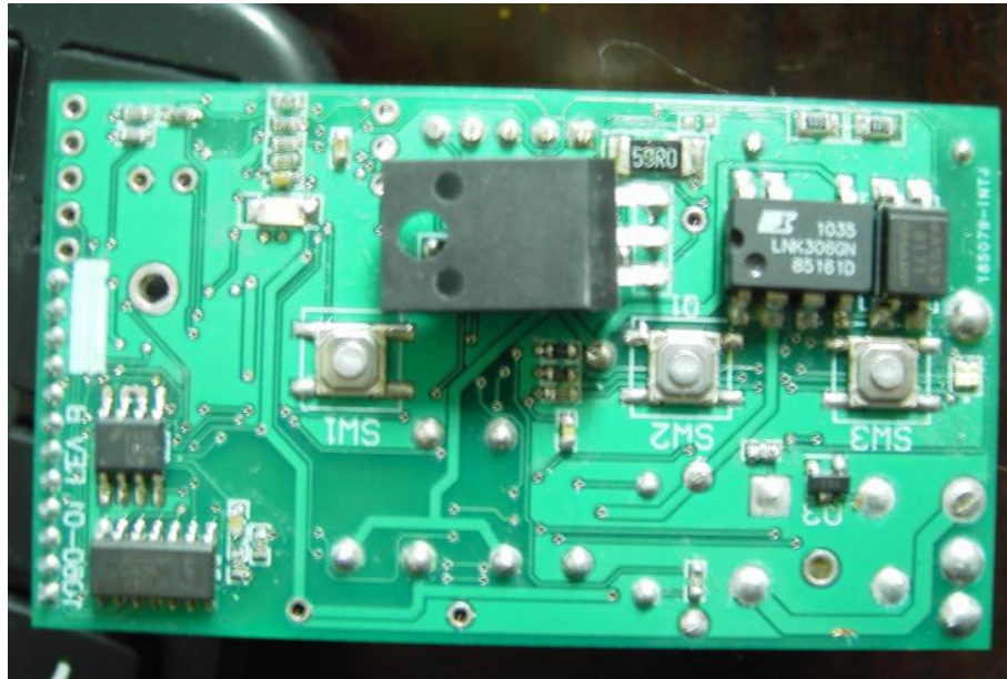
Figure 6 PCB of the EUT-Back View
