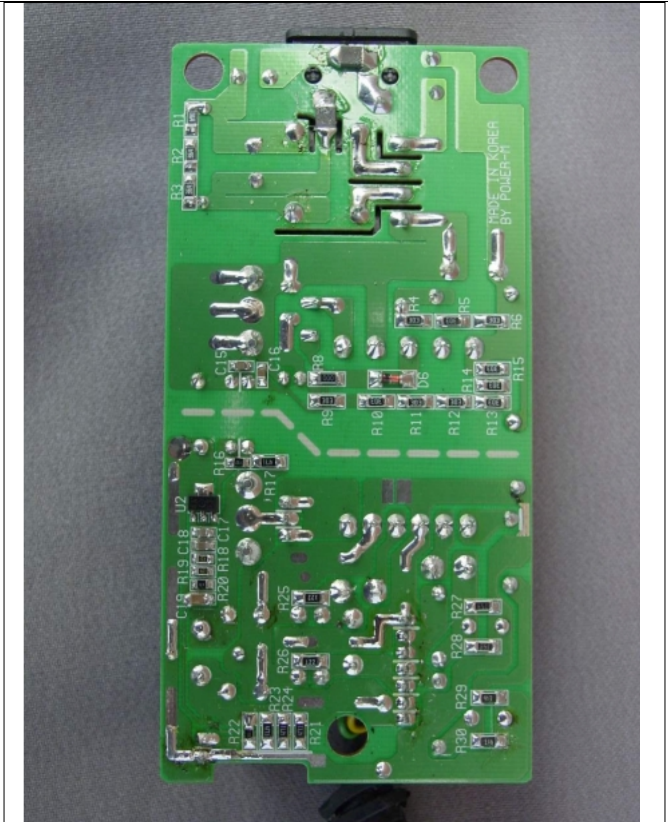
[Bottom view of the Adapter board]
