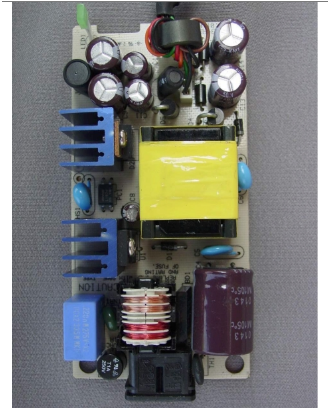
[ Top view of the Adapter board]
