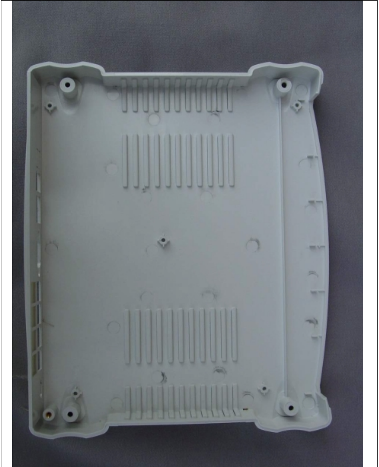
[ Lower cover view of the enclosure case ]
