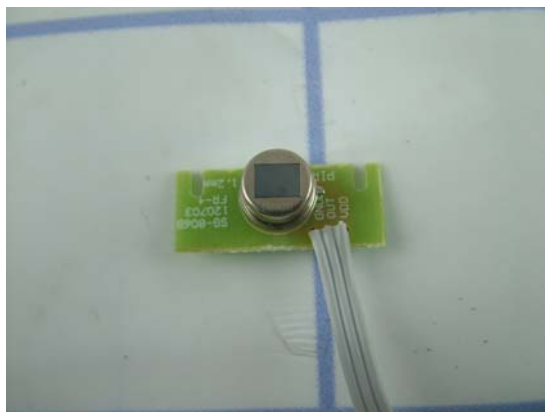
PCB2 side1
