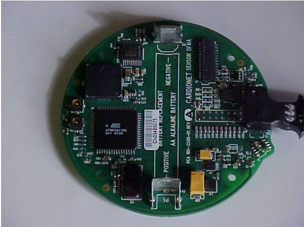
SENSOR PCB TOP
