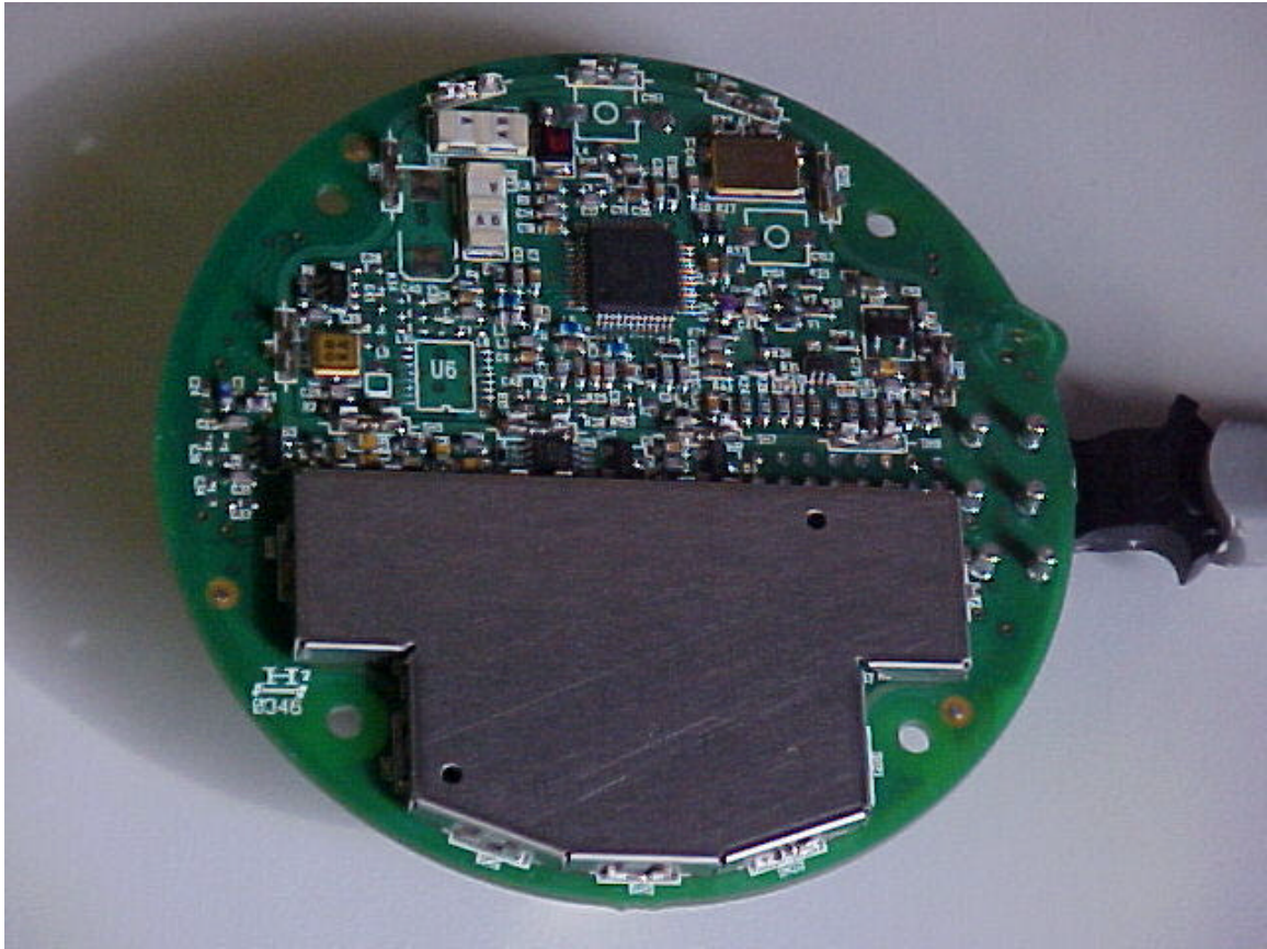
SENSOR PCB WITH SHIELD
