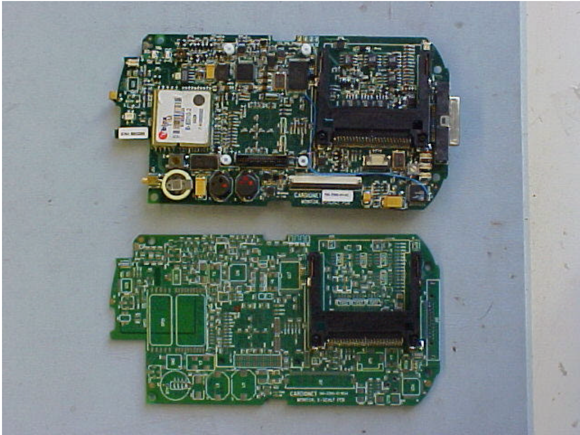
PCBS TOPSIDE
