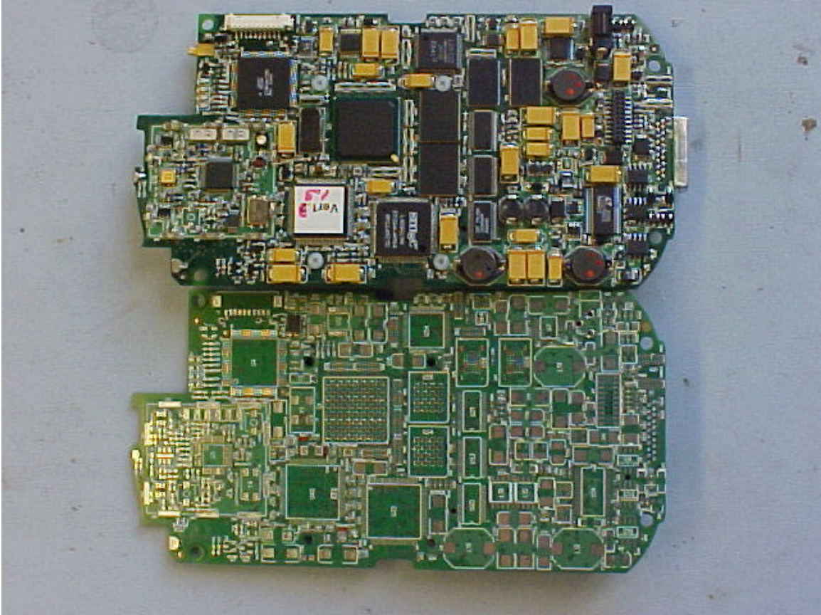
PCB BACKSIDE
