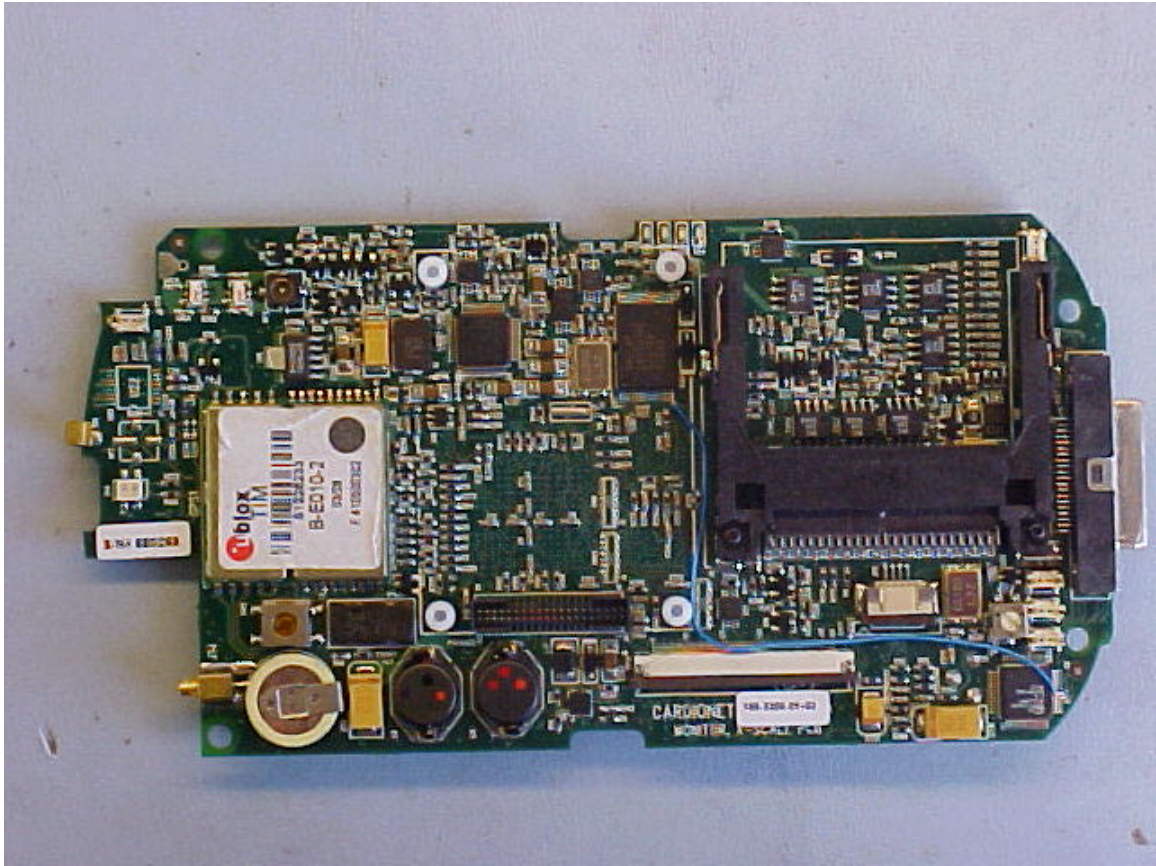
PCB TOPSIDE
