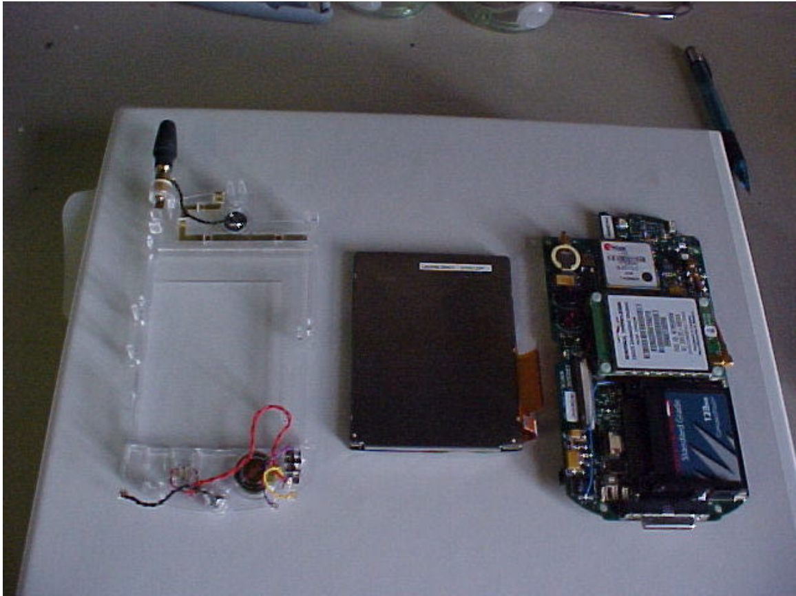
MONITOR ELECTRONICS
