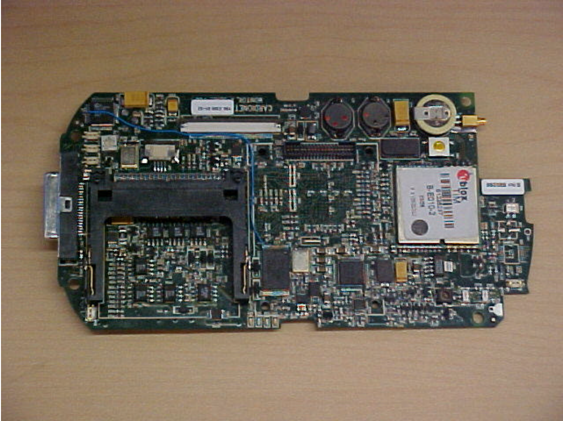
MONITOR PCB TOPSIDE
