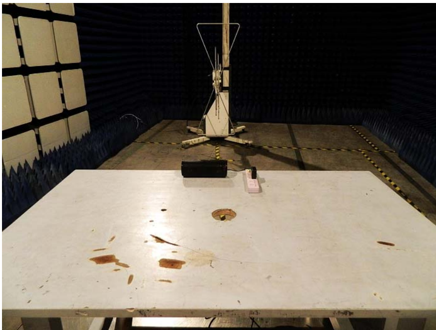
Radiated Emission
