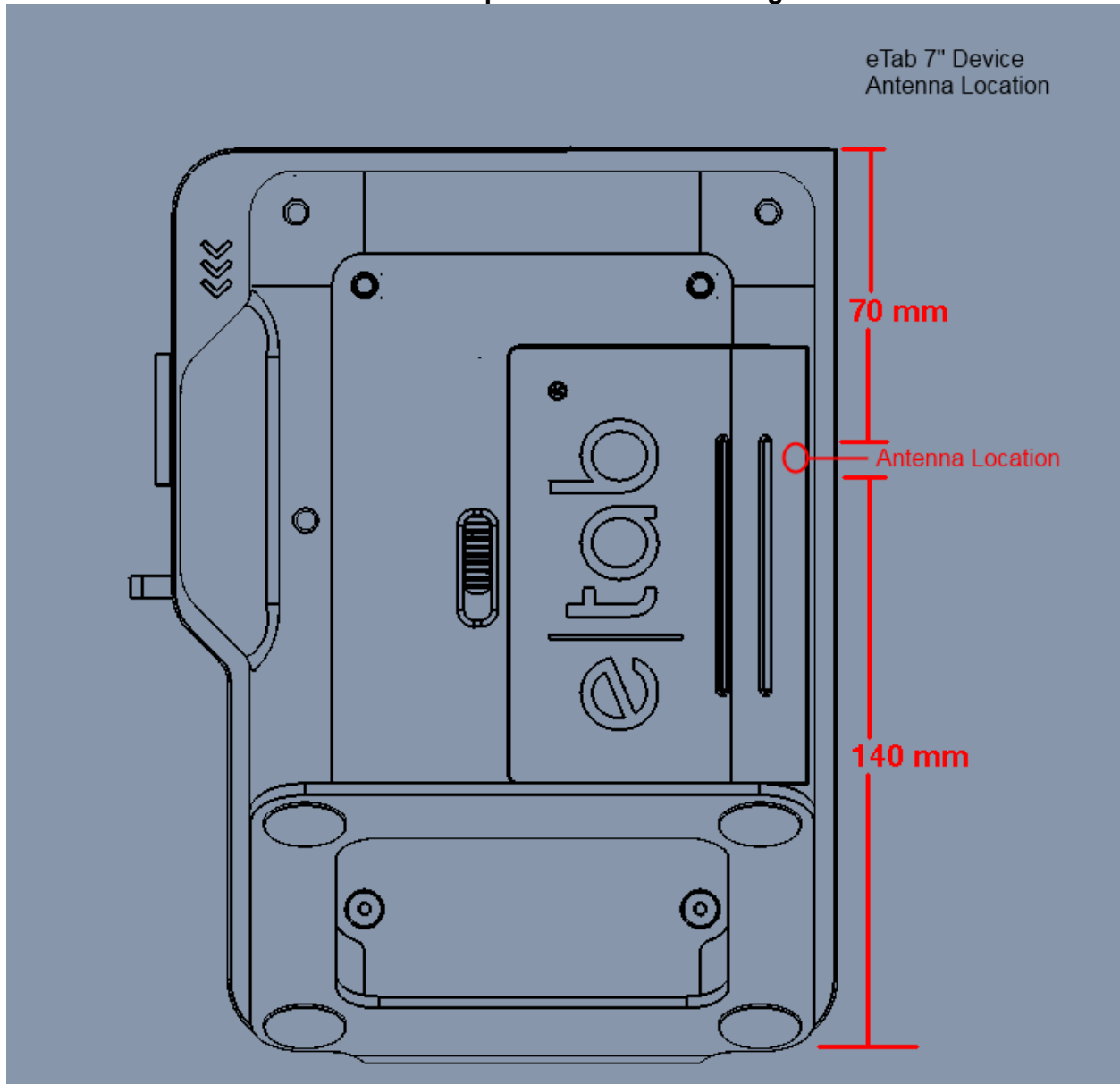
Antenna Locations
