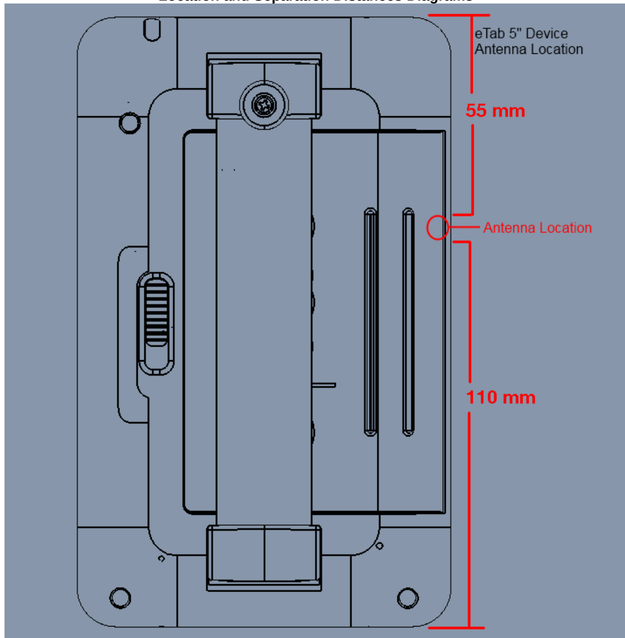
Antenna Location
