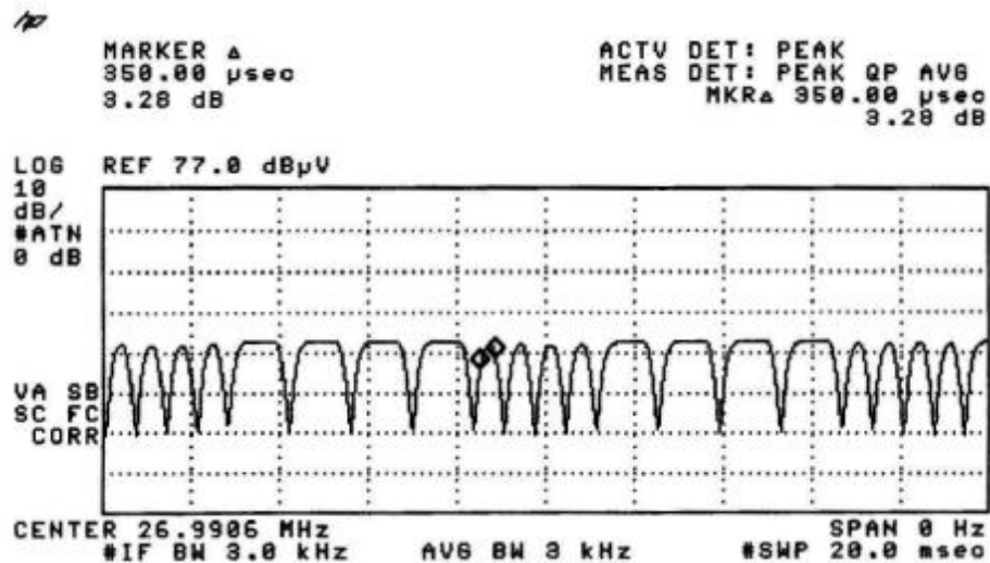
Figure C [Short Pulse]
