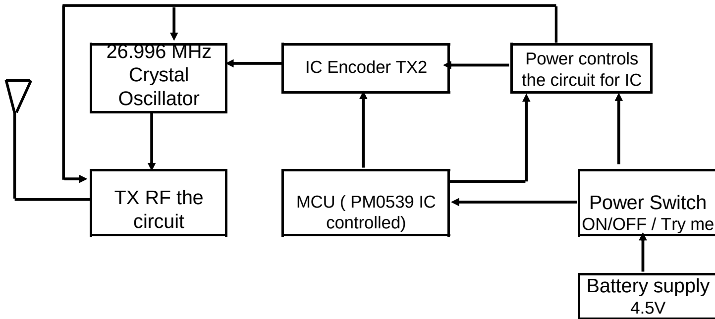
31805 13 " Hide & Seek TX bear , transmit the circuit block-diagram
