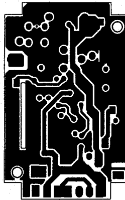
EEPCB2340A Bottom Layout
