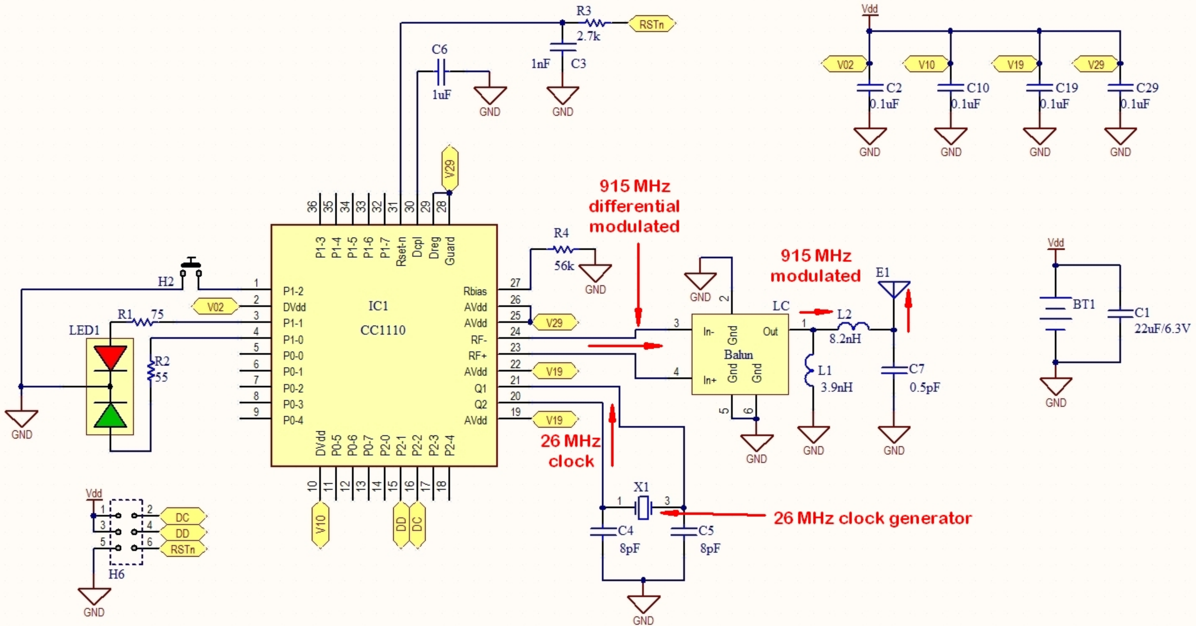
reelyActive RA-T411-02 schematic diagram
