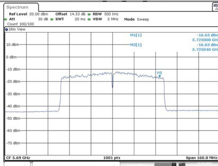
11AC80MIMO Ant2 5690 UNII-3
