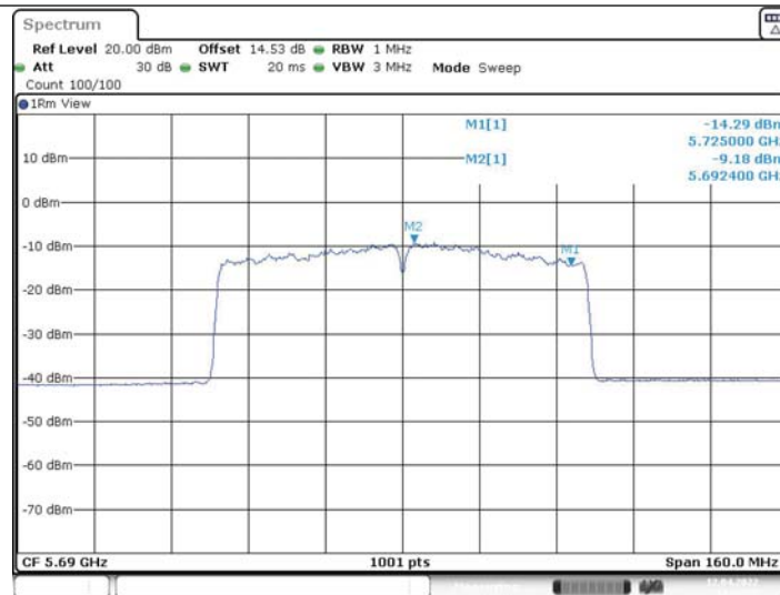
11AC80MIMO Ant1 5690 UNII-3
