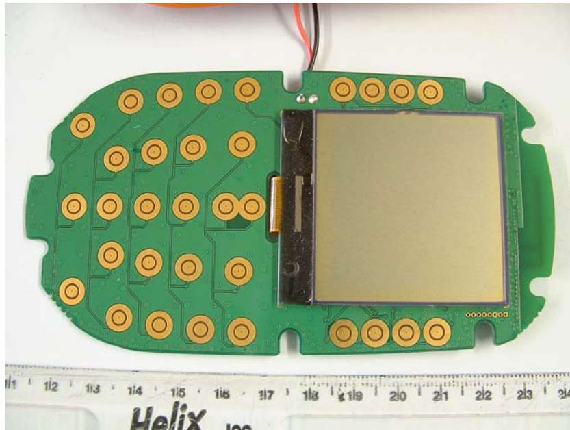
PCB Tack Side
