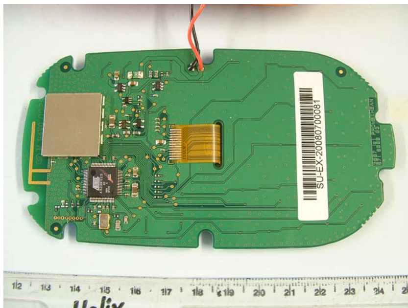
PCB Component Side
