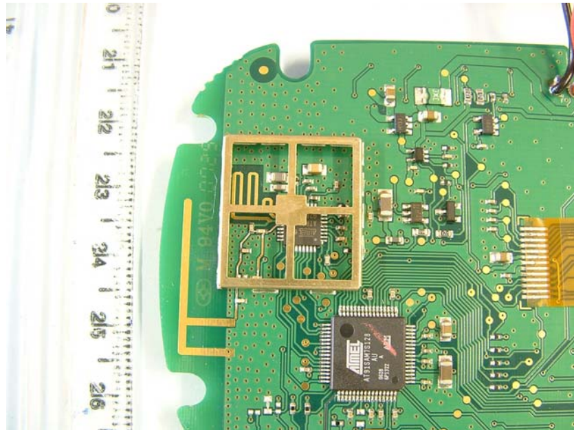
Close Up Of RF Section Can Cover Removed
