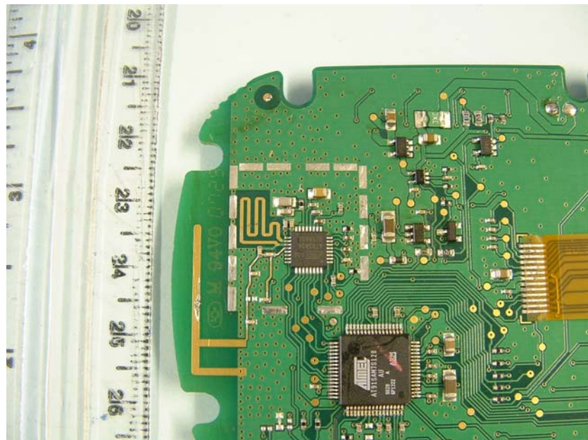
Close Up Of RF Section Can Removed
