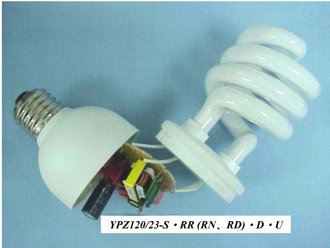
FIGURE 7 SELF-BALLASTED LAMPS FOR GENERAL LIGHTING (M/N: YPZ120/23-S • RR (RN, RD) • D • U) COVER REMOVED
