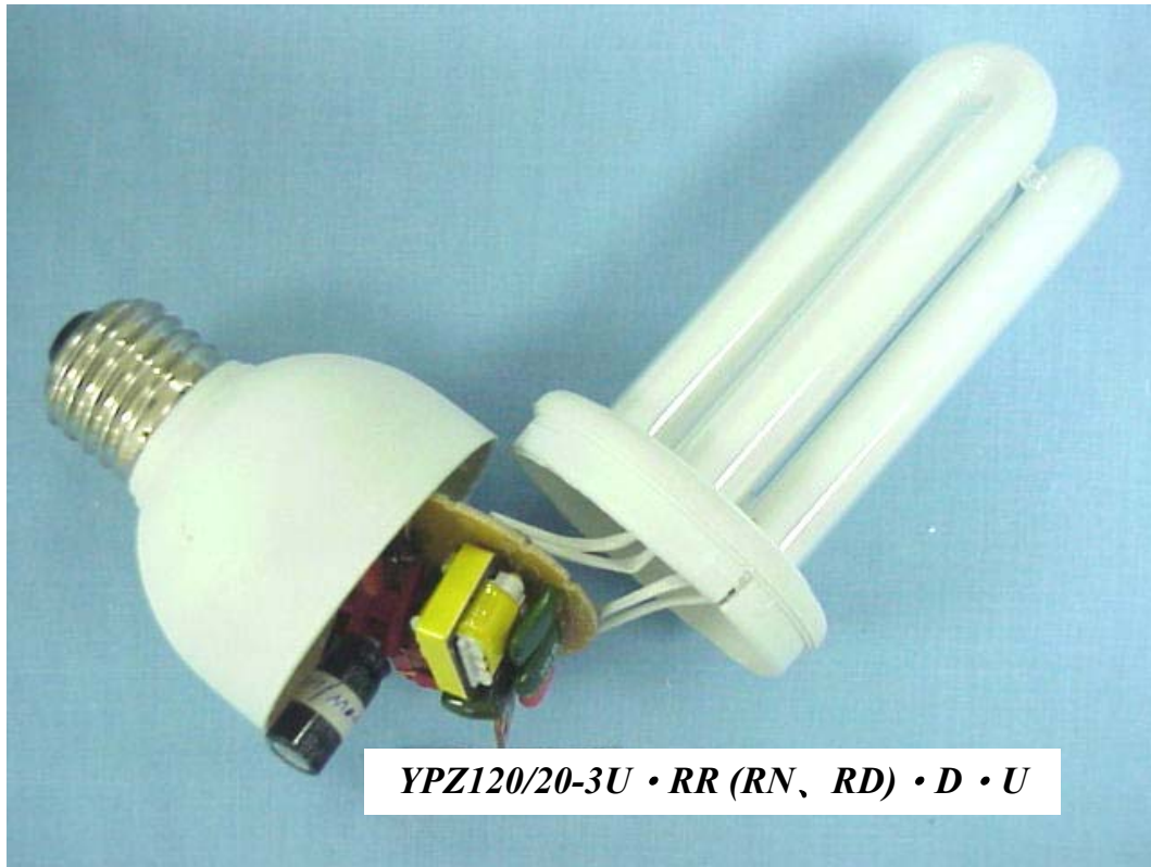
FIGURE 10 SELF-BALLASTED LAMPS FOR GENERAL LIGHTING (M/N: YPZ120/20-3U • RR (RN, RD) • D • U) COVER REMOVED
