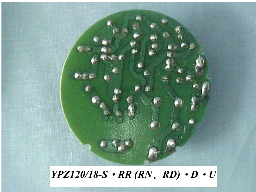
FIGURE 6 SELF-BALLASTED LAMPS FOR GENERAL LIGHTING (M/N: YPZ120/18-S • RR (RN, RD) • D • U) MAIN BOARD (SOLDERED SIDE)
