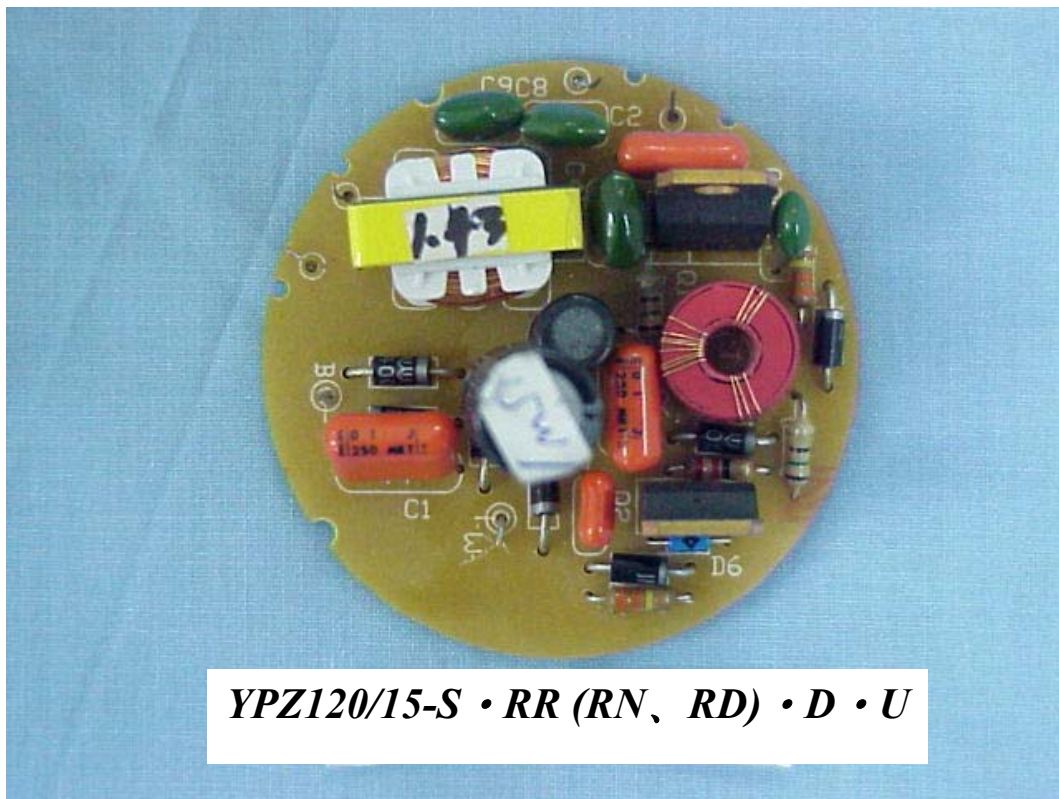
FIGURE 2 SELF-BALLASTED LAMPS FOR GENERAL LIGHTING (M/N: YPZ120/15-S • RR (RN, RD) • D • U) MAIN BOARD (COMPONENT SIDE)
