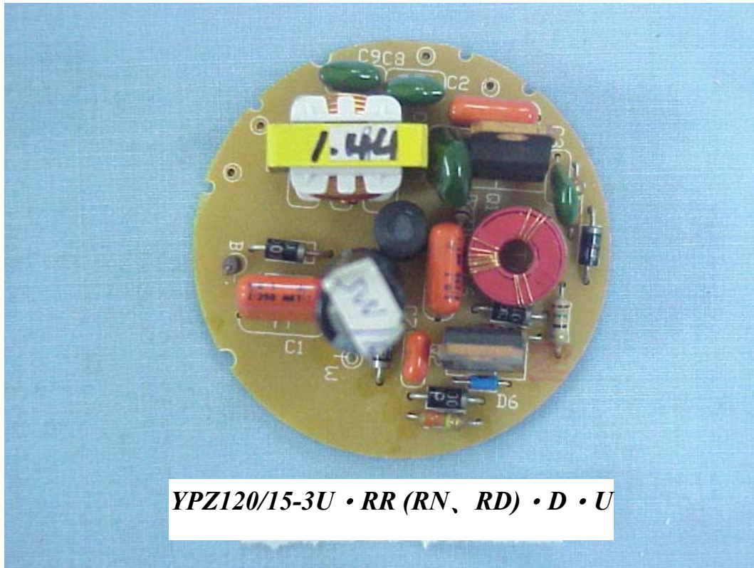
FIGURE 14 SELF-BALLASTED LAMPS FOR GENERAL LIGHTING (M/N: YPZ120/15-3U • RR (RN, RD) • D • U) MAIN BOARD (COMPONENT SIDE)
