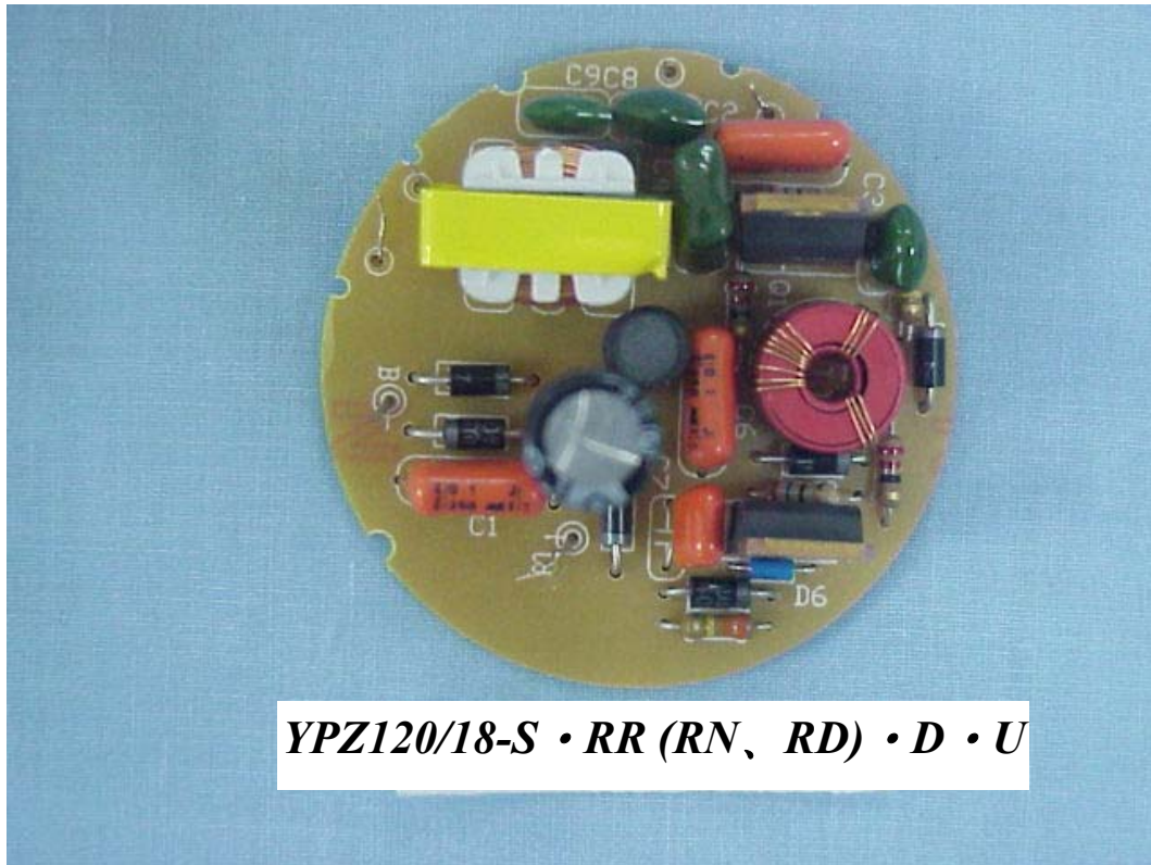
FIGURE 5 SELF-BALLASTED LAMPS FOR GENERAL LIGHTING (M/N: YPZ120/18-S • RR (RN, RD) • D • U) MAIN BOARD (COMPONENT SIDE)
