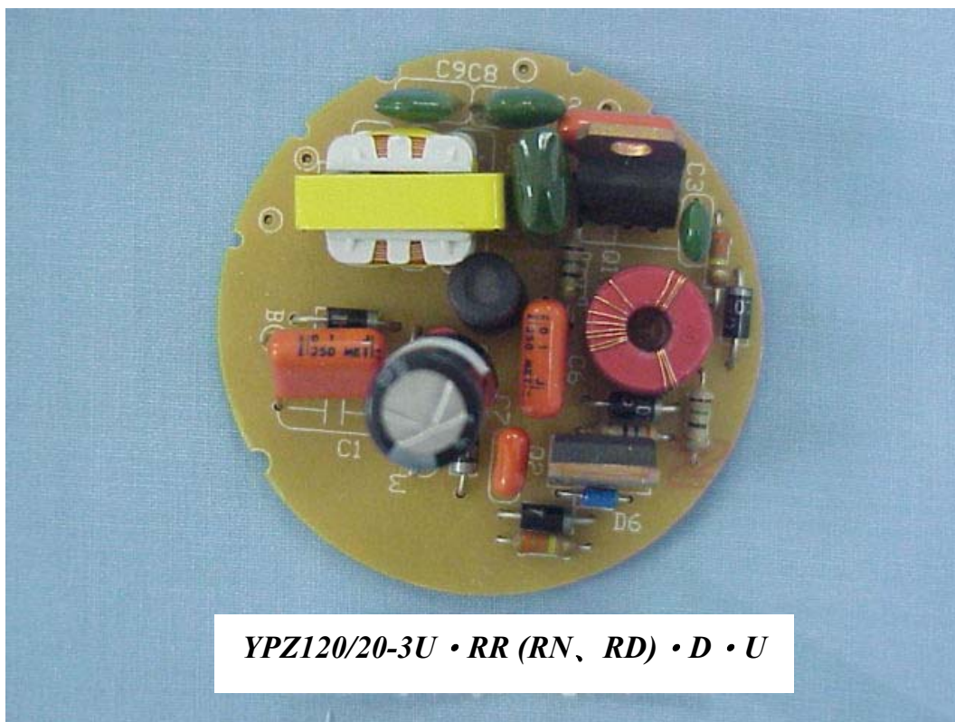
FIGURE 11 SELF-BALLASTED LAMPS FOR GENERAL LIGHTING (M/N: YPZ120/20-3U • RR (RN, RD) • D • U) MAIN BOARD (COMPONENT SIDE)
