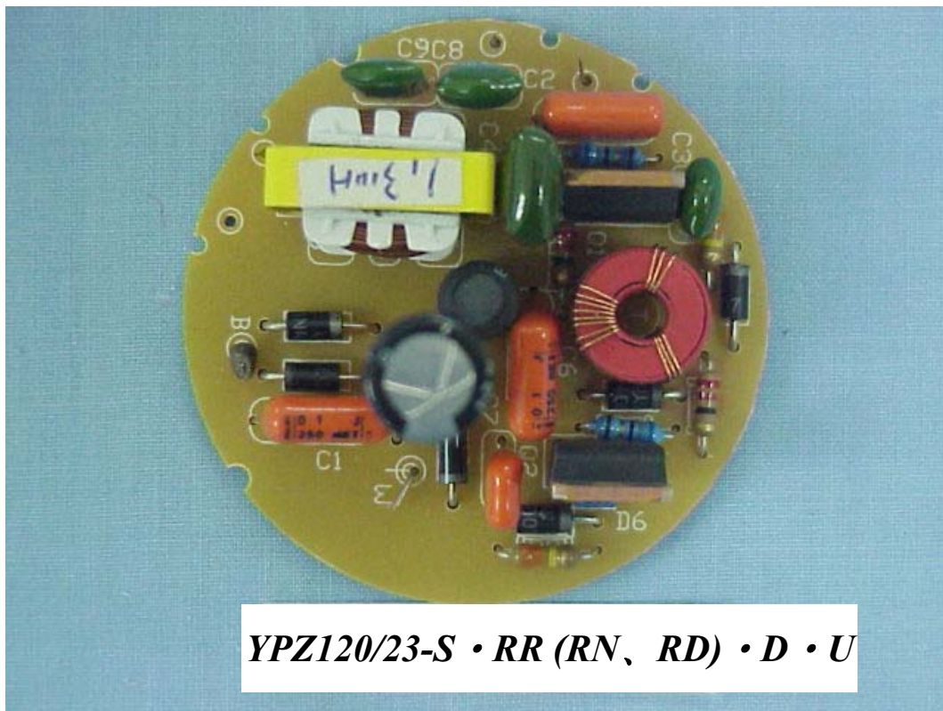
FIGURE 8 SELF-BALLASTED LAMPS FOR GENERAL LIGHTING (M/N: YPZ120/23-S • RR (RN, RD) • D • U) MAIN BOARD (COMPONENT SIDE)
