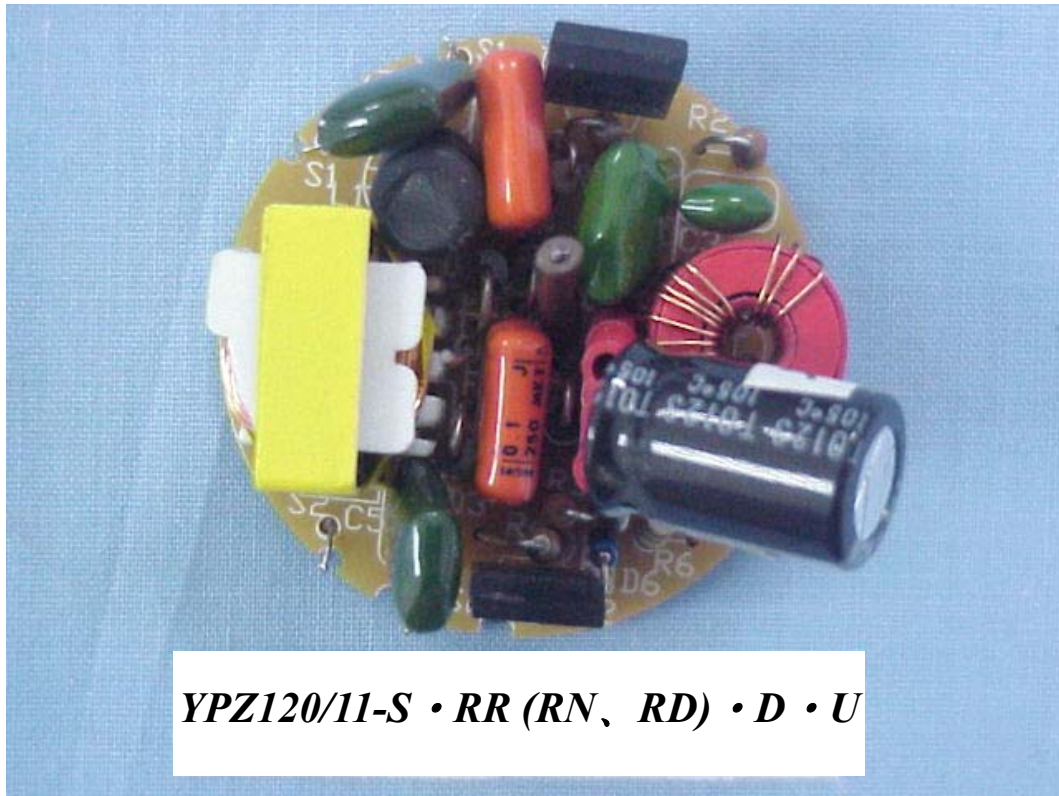
FIGURE 5 SELF-BALLASTED LAMPS FOR GENERAL LIGHTING (M/N: YPZ120/11-S • RR (RN, RD) • D • U) MAIN BOARD (COMPONENT SIDE)
