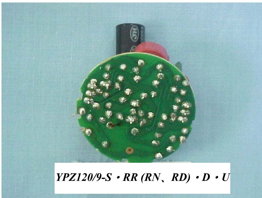
FIGURE 3 SELF-BALLASTED LAMPS FOR GENERAL LIGHTING (M/N: YPZ120/9-S • RR (RN, RD) • D • U) MAIN BOARD (SOLDERED SIDE)
