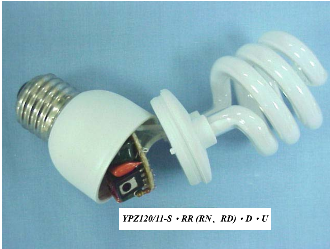
FIGURE 4 SELF-BALLASTED LAMPS FOR GENERAL LIGHTING (M/N: YPZ120/11-S • RR (RN, RD) • D • U) COVER REMOVED
